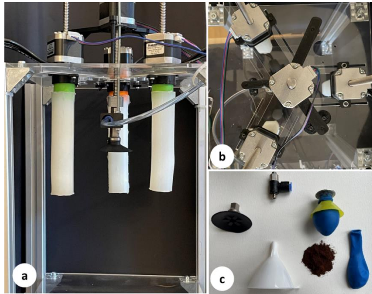
Figure 4.5. Schematic view of the proposed set-up assembly: a) The three soft fingers with variable lengths, b) The stiffed rod assemblies with their through-type stepper motors, c) Two easily interchangeable palms (suction cup and granular one).
