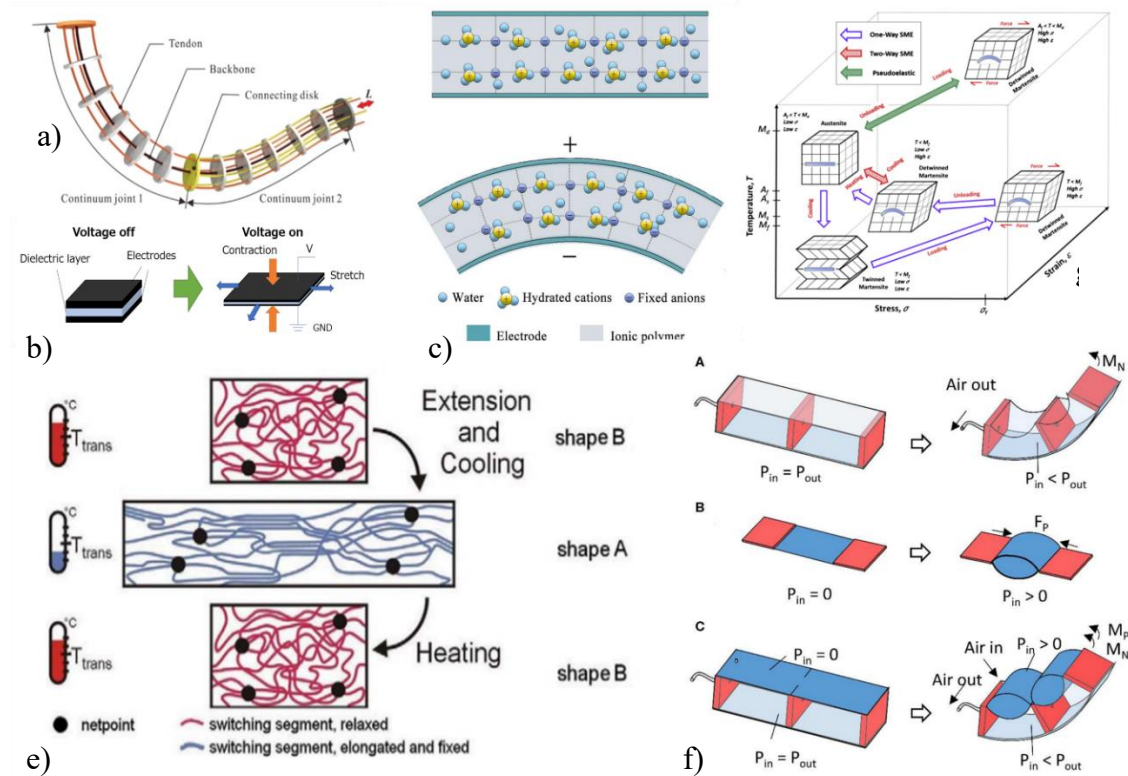
Figure 2.1. Different types of actuations in soft robots. a) Tendon-driven mechanisms [29], b) Dielectric elastomer actuators (DEAs) [30], c) Ionic polymer-metal composites (IPMCs) [31], d) Shape memory alloys (SMAs) [32], e) Shape memory polymers (SMPs) [33], f) Soft fluidic actuators (SFAs) [34].
