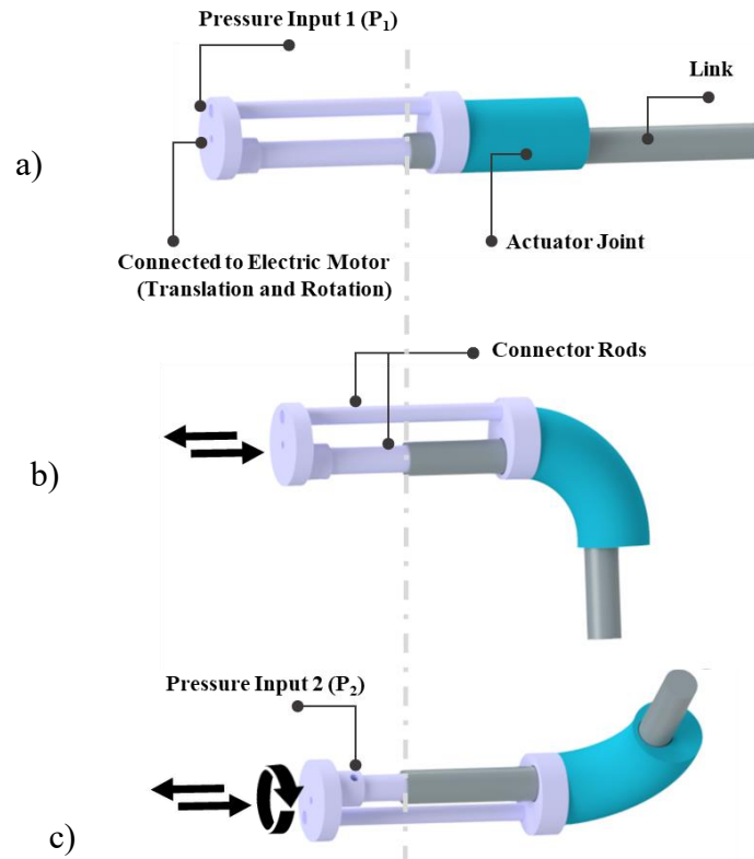
Figure 3.1. a) Schematic view of the proposed finger. b) sliding the joint along the link will change the bending point and the effective length of the finger. c) rotation of the joint along with its axis results in changing the bending direction in 3D space.
