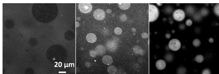
FIGURE 44. CLSM IMAGES OF A/P EMULSIONS WITH 0.2 wt% CNC WITHOUT PEC (LEFT), 0.11 wt% PEC (MIDDLE) AND 0.8 wt% PEC (RIGHT). THE CONTRAST WAS ENHANCED TO FACILITATE VISUALIZATION. THE BRIGHTNESS ARE DUE TO THE 5 ppm NB USED TO LABEL THE CNC. ALL IMAGES ARE AT THE SAME SCALE.
