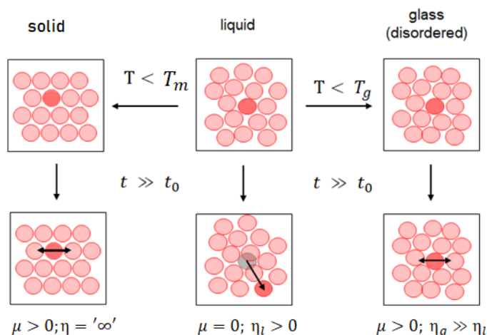
Figure 1.2: Schematic representation of a system in the 3 states: crystalline solid, liquid and glassy phase. Here T_m is the melting point and T_g is the dynamic glass transition temperature. Viscosity for the solid, liquid and glass is noted as \eta , \eta_l and \eta_g respectively and the elastic shear modulus is \mu for all cases. t_0 is the time which a particle needs to move across its own size. When a liquid is cooled towards T_g , the values for the shear modulus \mu and the viscosity \eta_g start to increase and the liquid-glass transition occurs. For the glass \eta_g is not infinite as it is for an ideal crystal but it is still much larger than in the case of the liquid, \eta_g \gg \eta_l . Let us wait long enough so that the measurement time t is much larger than the time t_0 , and look at the structure of each state again. For crystals one can see that atoms show ordering and vibrate around their regular equilibrium positions. In liquids atoms are able to move far. However, for glasses despite the similar disordered structure atoms are not able to move far.
