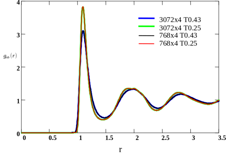
Figure 3.3: The radial distribution functions for nonbonded monomers, g_{\text{nb}}(r) , for two systems, 3072 \times 4 and 768 \times 4 at T = 0.43 (blue and black curves) and at T = 0.25 (green and red curves). The curves for different systems superimpose perfectly on one another.
