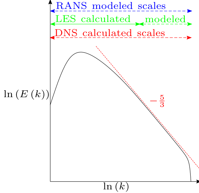
Figure 2-1: Schematic illustration of the distribution of turbulent kinetic energy by wavenumber and the different strategies available for simulation of turbulent flows.
