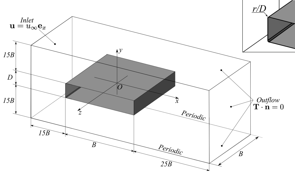
Figure 6-1: Sketch of the computational domain.
