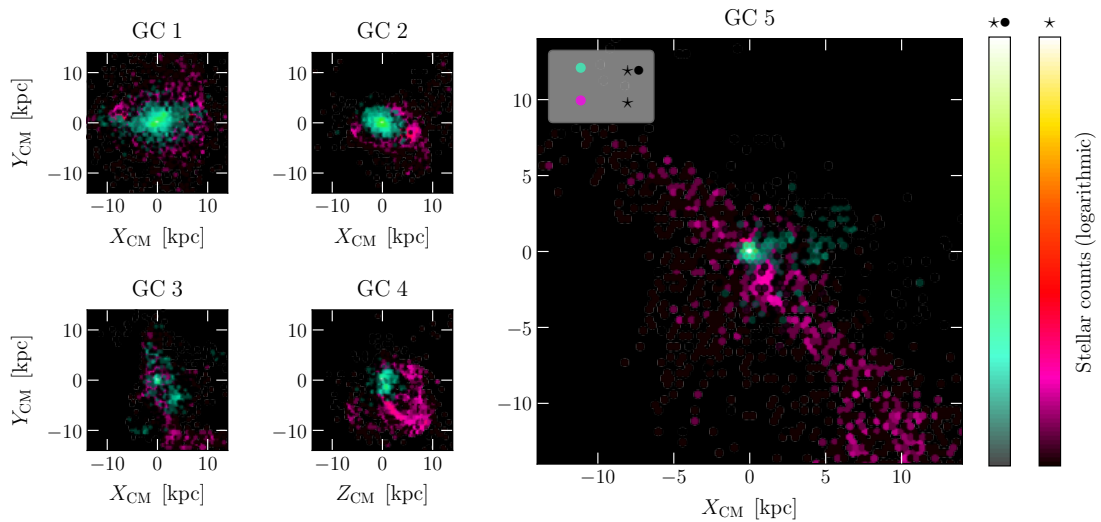
Figure 44: Dark matter impact on tidal tails : Stellar distribution of globular clusters formed in dark matter mini-halos ( \star\bullet , turquoise) and globular clusters devoid of dark matter ( \star , magenta) at the last snapshot of our simulations. The hexagonal bins were colour-coded by the bin's stellar counts in a logarithmic scale indicated in the colour-bars. The stellar distribution is projected on the X vs. Y plane for GC1, GC2, GC3 and GC5, while GC4 is projected in the Z vs. Y plane for better visualisation of its particular orbit. This plot highlights more prominent tails in the dark matter-free case, while clusters formed inside dark matter mini-halos present a diffuse stellar envelope with much smaller dimensions than its respective tails. This figure was originally published in Vital and Boldrini, 2022 .
