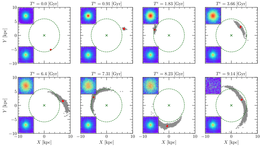
Figure 48: Formation of tidal tails : Snapshots of the GC simulated in Boldrini and Vitral, 2021 , at different times. Bound and unbound particles are represented in red and grey, respectively. The subplots on the left are a zoomed-in view of the bound particles at each time, over a region up to \sim 6 pc from its centre, with the top plots representing the evolving GC in our simulation and the bottom plots depicting a NGC 6397-like GC. The green cross points the centre of the galaxy and the green circle has a radius of 5.91 kpc, i.e. the galactocentric distance of the GC. One can notice extended tidal tails of sizes greater than 1 kpc in roughly 3.66 Gyr, which is well below the age of NGC 6397 (12.87 Gyr). Consequently, we predict that NGC 6397 should exhibit tidal tails and these should be clearly observable. This figure was originally published in Boldrini and Vitral, 2021 .
