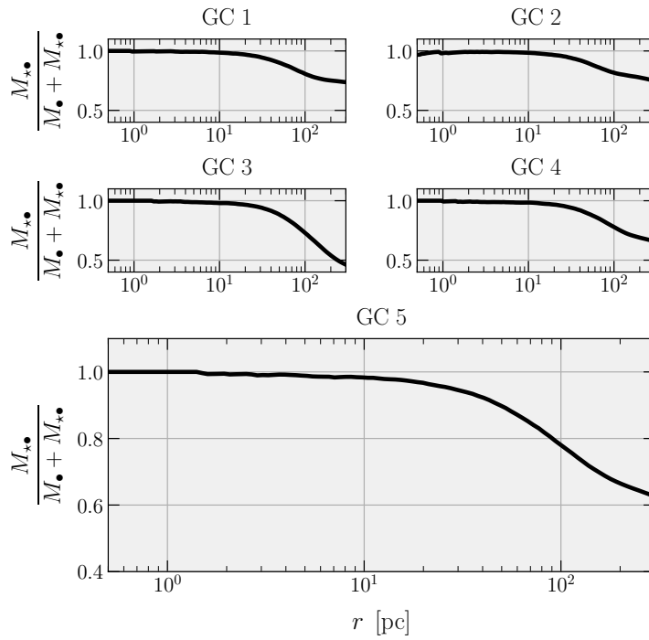
Figure 47: Cumulative mass ratio : Comparison of the cumulative mass ratio of stellar to total mass (i.e., M_{*•}/[M_{•} + M_{*•}] ) as a function of distance to the cluster centre (in pc), for globular clusters simulated inside dark matter mini-halos at the end of our simulations. This plot exalts how difficult it is to detect considerable amounts of dark matter up to hundreds of pc away from the cluster centre. This figure was originally published in Vitrail and Boldrini, 2022 .
