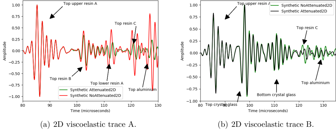
Figure 4.16. For the zero-offset data case in 2D: comparison between the synthetic 2D data with viscoelastic rheology (attenuation) and the synthetic 2D data with elastic rheology (no attenuation) for the traces A (Figure 4.16(a)) and B (Figure 4.16(b)). All the data are filtered with a 250-650 kHz band-pass filter.
