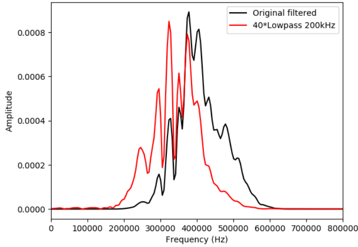
Figure 4.31. Spectra of the original band-pass filtered source and the low-pass filtered source.
