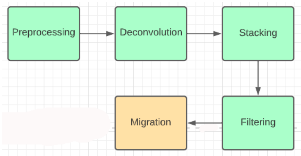
Figure 1.9. Principal processing steps.
