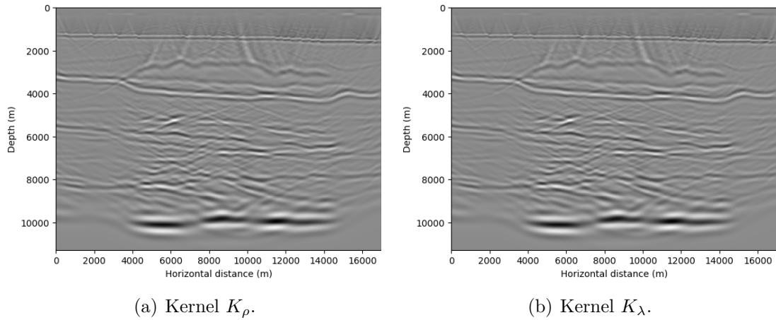
Figure 3.14. Kernels K_\lambda and K_\rho using free-surface conditions to compute the forward and adjoint problems using the model M2 as the a priori model, applying the case 1 with f^\dagger = d_{obs} - d_{calc} . The observed data are computed using free surface conditions at the top of the copoutational domain (free-surface multiples are present). The sources and receivers are located at the top of the water.
