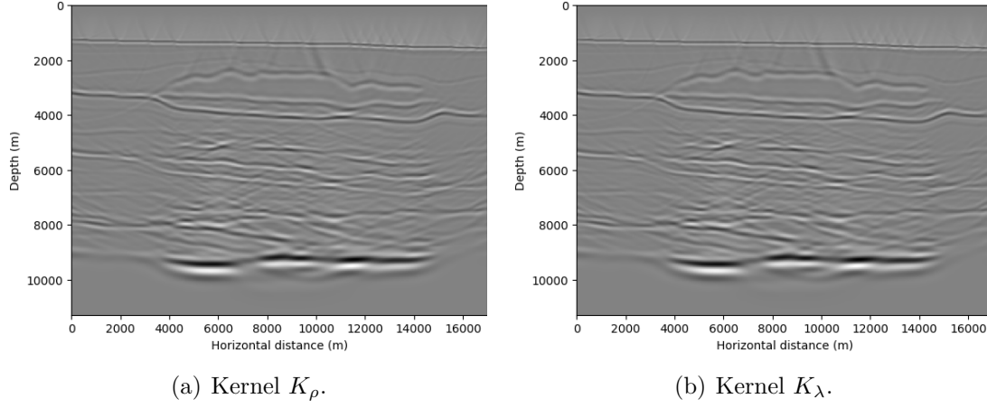
Figure 3.16. Kernels K_\lambda and K_\rho using absorbing-boundary conditions to compute the forward and adjoint problems using the model M2 as the a priori model, applying the case 2 with \mathbf{f}^\dagger = \mathbf{d}_{obs} - \mathbf{d}_{calc} . The observed data are computed using free surface conditions at the top of the computational domain (free-surface multiples are present). The sources and receivers are located at the top of the water.
