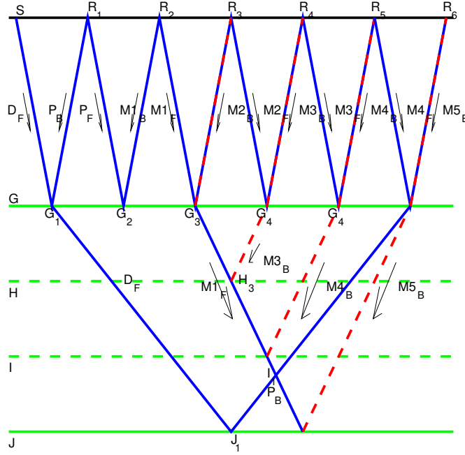
Figure 2.2. Correlation between the direct wavefield \mathcal{D}_{\mathcal{F}} of the forward wavefield \mathcal{F} and the primaries and multiples ( \mathcal{P}_{\mathcal{B}} and \mathcal{M}_{\mathcal{B}} ) of the back-propagated wavefield \mathcal{B} . We can see that the direct wave \mathcal{D}_{\mathcal{F}} interacts with the primary \mathcal{P}_{\mathcal{B}} from receiver R_1 at the interface G represented with a solid green line (the exact interaction is at the point G_1 ), and it interacts with the primary coming from receiver R_6 at the interface J represented with a solid green line (the exact interaction is at the point J_1 ). However we can also see that the multiple M1_F interacts with different "back-propagated" multiples ( M3_B and M4_B ) from receivers R_4 , R_5 at spurious interfaces H and I respectively (represented with dashed green lines). We can also see another phenomenon called interference: the multiple M1_F interacts with the multiples M5_B from receiver R_6 at the true interface J .
