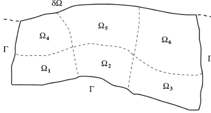
Figure D.2. Example of a discretization in the Finite Element method. Note that the elements are not necessarily equal. Therefore, they could adapt to the edges of the model. Taken from Komatitsch and Tromp [1999].
