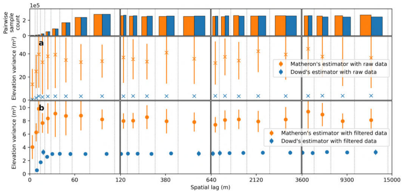
Fig. S11: Effect of estimator's robustness on variogram estimation. a-b , Empirical variogram of elevation differences for estimators by Matheron [148] and Dowd [146] ( a ) before and ( b ) after outlier filtering, with 1\sigma dispersion estimated by the standard deviation of 100 independent realizations. Both variograms are estimated directly on elevation differences, without standardization. a , A simple filtering of elevation differences greater than 500 m is performed. b , Elevation differences outside a 7NMAD interval centered on the median are excluded, for each category of slope and maximum absolute curvature (Fig. 3).
