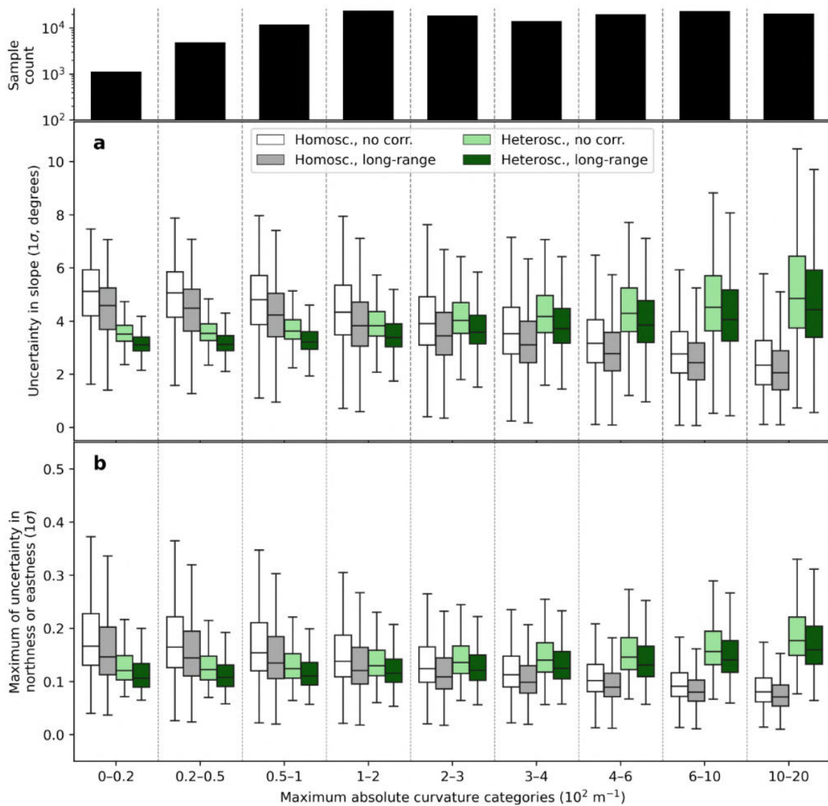
Fig. S20: Impact of maximum absolute curvature on uncertainty propagation to terrain slope and orientation. a-b, Distributions of slope and orientation uncertainties by category of maximum absolute curvature for each scenario, with boxes denoting the interquartile range and whiskers extending to the whole distribution.
