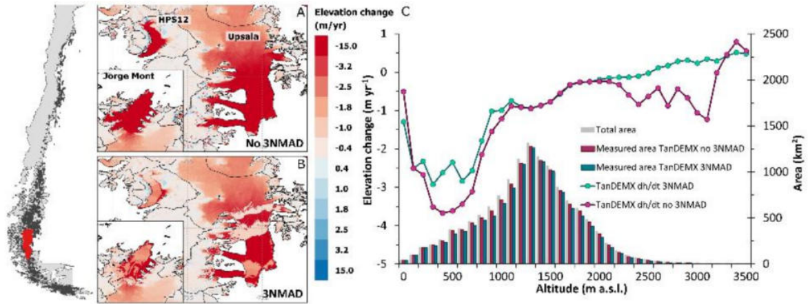
Figure 3.8: Influence of the NMAD filter in hypsometric glacier elevation change interpolation. From Dussaillant et al. (2019). Example at the Southern Patagonian Icefield. TanDEM-X elevation changes of Braun et al. (2019) are used due to their nearly-complete coverage. (A) TanDEM-X elevation changes for Jorge Mont, HPS12 and Upsala glaciers without filter. (B) TanDEM-X elevation changes using a 3 NMAD filter for each 100 m elevation band of the SPI. (C) TanDEM-X hypsometric elevation changes for the entire icefield, without filter (purple) and with a 3 NMAD filter (blue).
