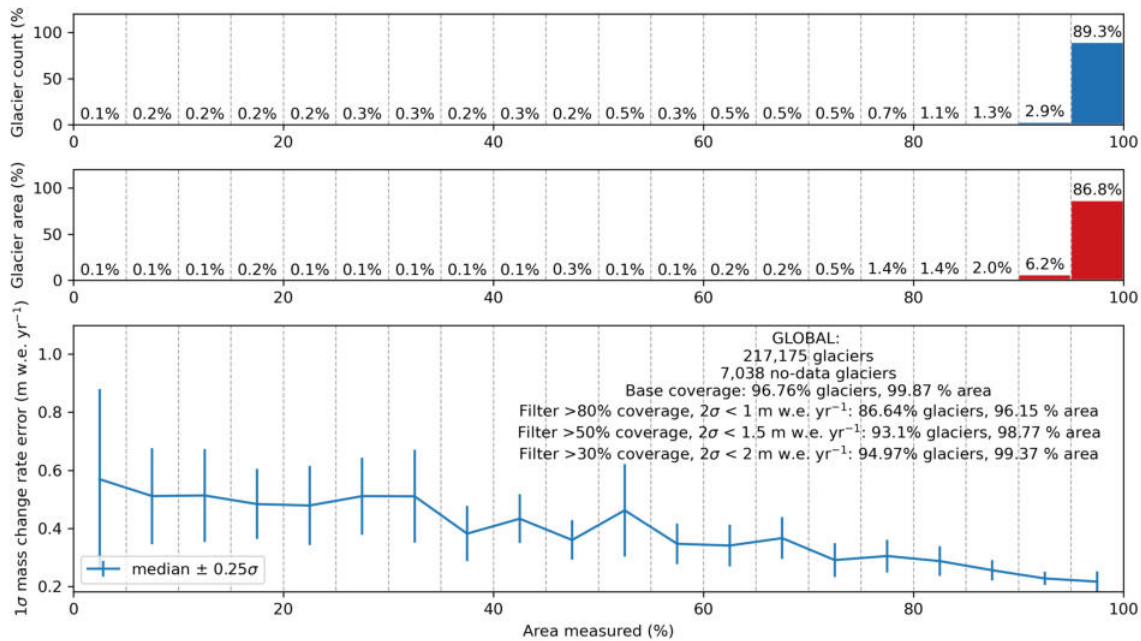
Figure 3.30: Coverage and uncertainties of glacier estimates. Uncertainty of glacier mass change estimates of Hugonnet et al. (2021) aggregated by percentage of glacier area measured. The top two panels show histograms of glaciers in each bin, per number of glacier and per glacierized area. The first filtering choice listed was kept for the study of Rounce et al. (in review) to ensure highest quality estimates. Glaciers without observations were calibrated on the regional average.
