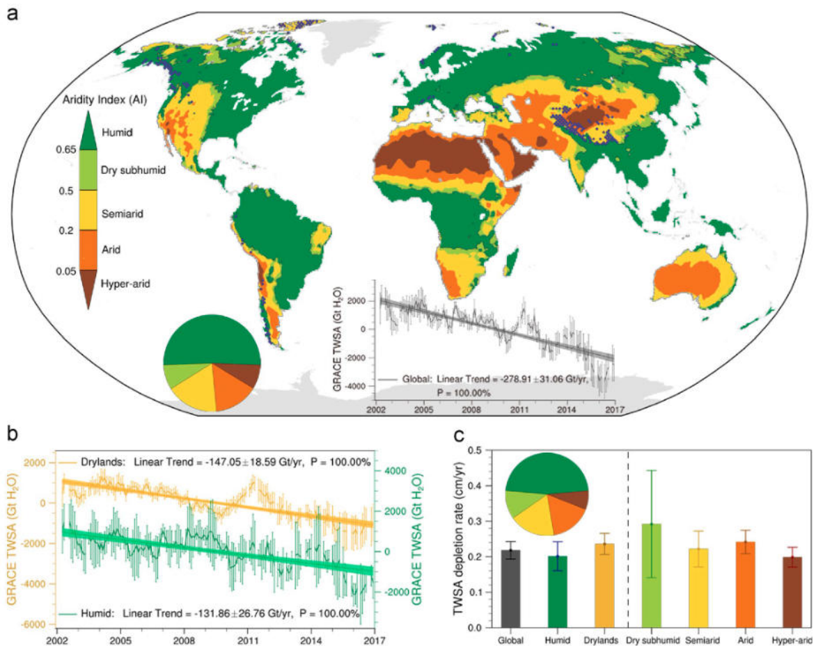
Figure 3.35: Terrestrial water storage trends over different climate zones from GRACE observations, 2002–2016. From An et al. (2021) . a , Map of climate zones based on the long-term Aridity Index (1961–1990). Blue dots show glacierized regions. The inset pie chart illustrates the proportions of global land area for each climate zone. The inset time series illustrates monthly deseasonalized TWS anomalies in global landmass, with error bars and shading denoting 95% confidence intervals of monthly anomalies and the best-fit linear trend, respectively. b , Same as the inset time series in (a) , but for monthly deseasonalized TWS anomalies in drylands (yellow) and humid regions (green). c , TWS decline rates (in \text{cm yr}^{-1} ) for each climate zone. Error bars show 95% confidence intervals. The inset pie chart illustrates the relative contributions of each climate zone to the global TWS change (in \text{Gt yr}^{-1} ).
