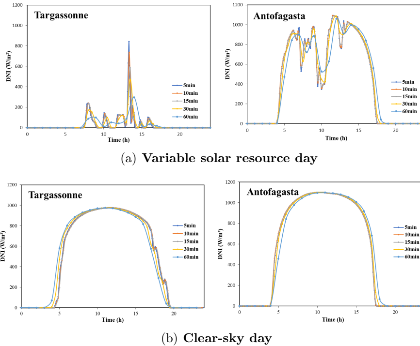
Figure B.14: Variation of estimated DNI resource using Solcast for different time resolutions during: (a) highly variable solar resource days (January 1 st , 2018 at Targassonne and January 2 nd , 2018 at Antofagasta) and (b) clear-sky day (June 19 th , 2018 at Targassonne and January 1 st , 2018 at Antofagasta).
