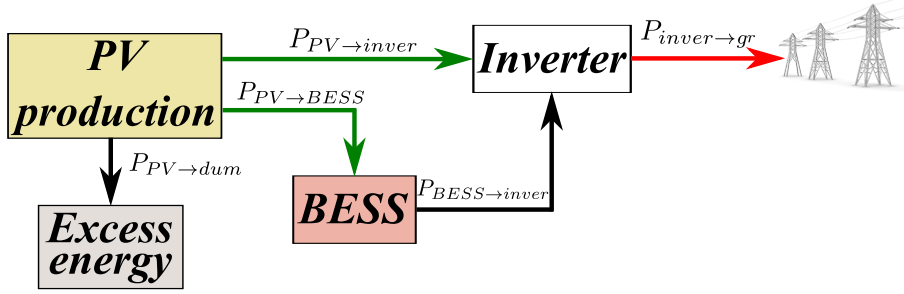
Figure 4.4: Simplified PV with BESS model, summarizing the main power flows.
