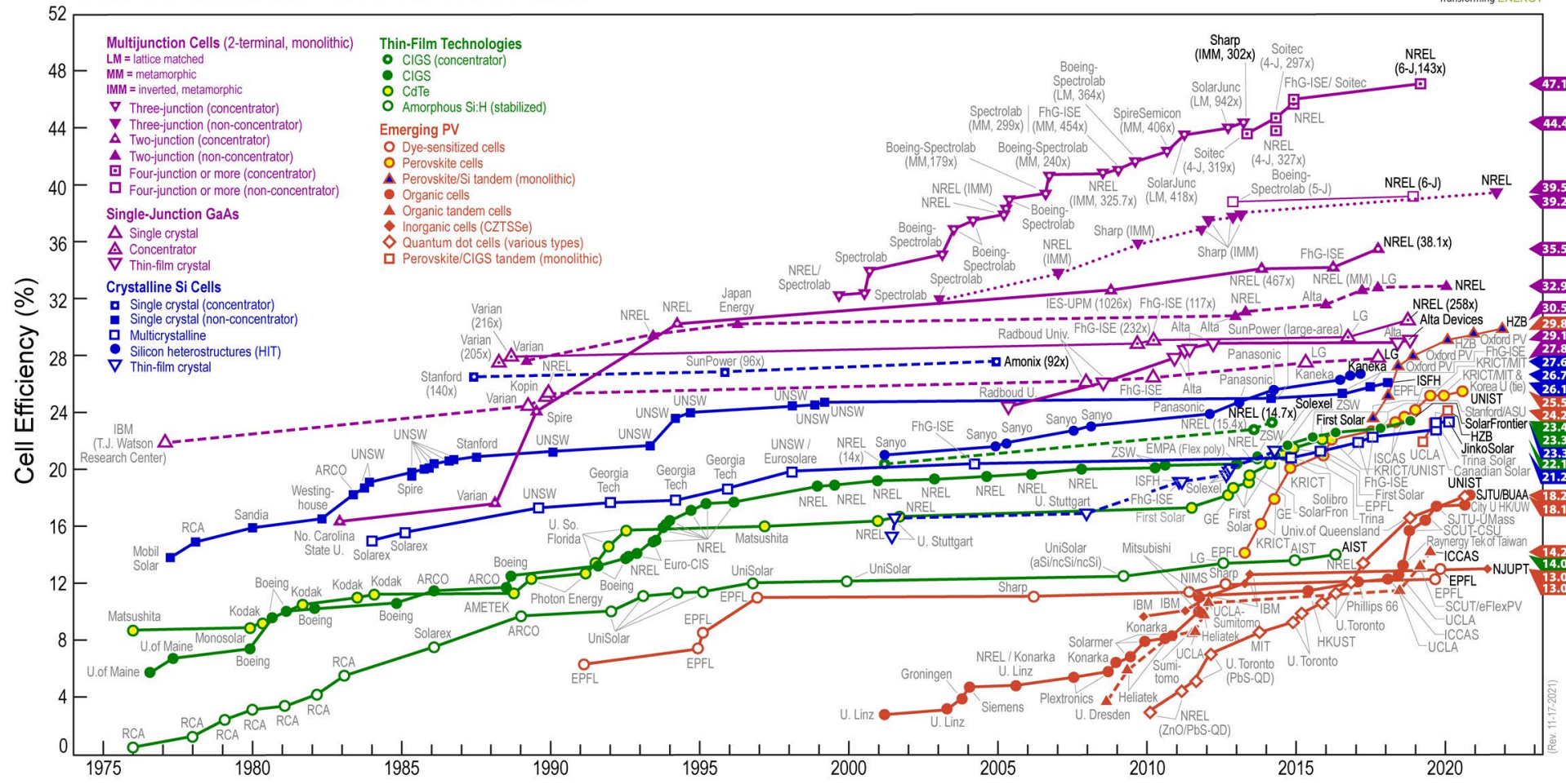
Figure 1.8: Evolution of different cell technologies efficiencies [13].
