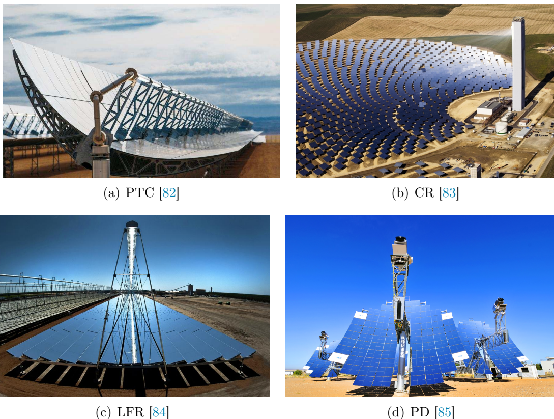
Figure 1.2: Illustration of the four main CSP technologies: (a) PTC (Noor I Ouarzazate, Morocco 160 MW capacity and 3.5 h TES), (b) SPT (PS10 at Seville, Spain 10 MW), (c) LFR (Rajasthan Sun Technique Energy, 100 MW) and (d) PD (tested at Albuquerque, New Mexico).
