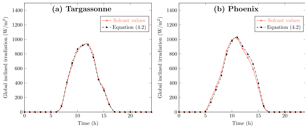
Figure 4.6: Comparison between estimated global irradiance on a tilted surface using Solcast database and Eq. (4.2) at two different locations: (a) Targassonne (FR) and (b) Phoenix (USA).
