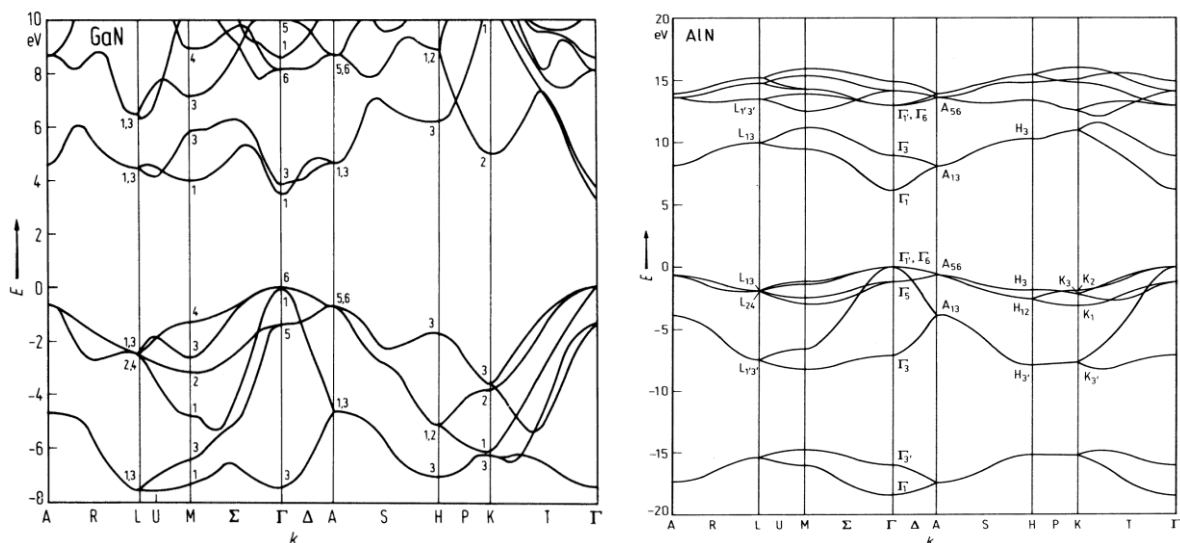
Figure 8. a) Band structure of wurtzite GaN in the 1st Brillouin zone. b) Band structure of wurtzite AlN in the 1st Brillouin zone [18].
