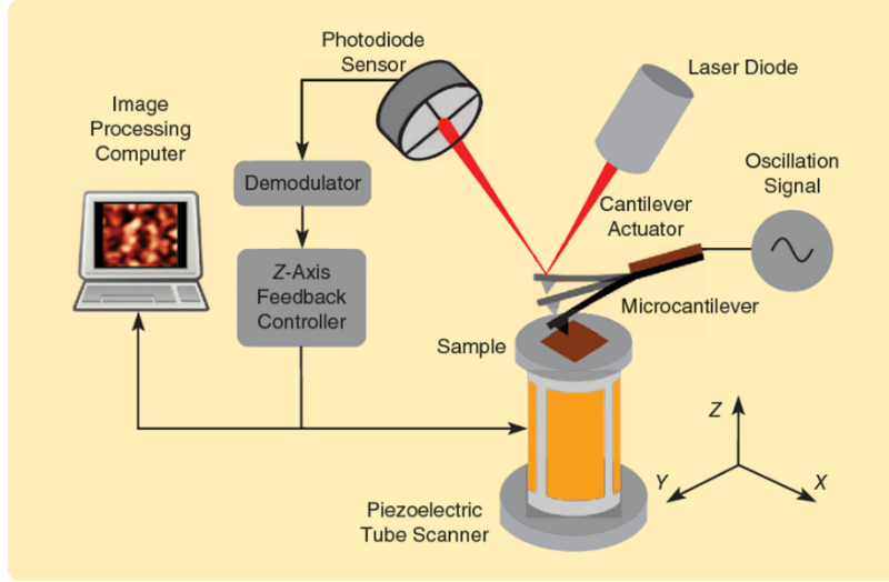
Figure 35. A schematic of the instrumentation of a typical atomic force microscope operating in tapping mode [105].
