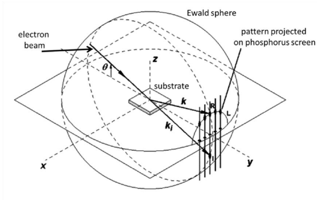
Figure 18. Ewald sphere and the RHEED principle [66].
