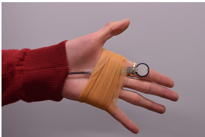
Figure 3.4: A force-sensing resistor used as a rhythm interface, to be used combined with a theremin. The sensor is held in place in the hand that also controls intensity, with the combination of a ring and a fabric strip.
