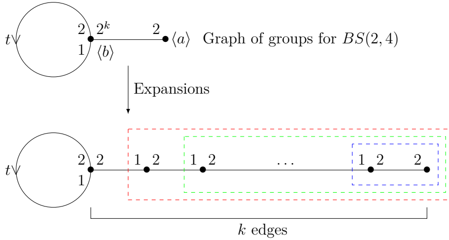
Figure 1.2 – A construction of arbitrary long special factor sequences in BS(2, 4) . The upper graph represents BS(2, 4) with the presentation \langle a, b, t | tbt^{-1} = b^2, a^2 = b^{2^k} \rangle . Expansions from this graph lead to the graph below, which has many edges. The rectangles show some special factors which can be read in the graph below. Here we can construct a sequence of k nested special factors.
