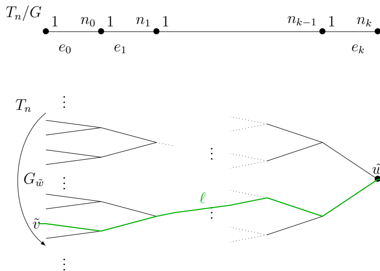
Figure 3.7 – Pre-image of an increasing subsegment
