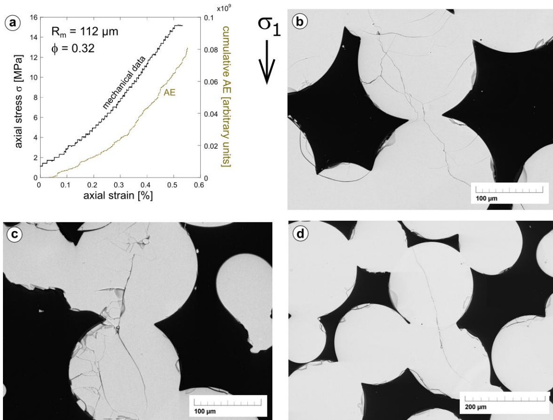
Figure 3.13 (a) Mechanical data and (b)(c)(d) scanning electron micrographs for a synthetic sample with a porosity of 0.32 and mean grain size of 112 \mu\text{m} deformed under uniaxial compression up to an axial strain of approximately 0.5%. The microstructure shows that microcracks initiate at grain-to-grain contacts and form Hertzian fractures.
