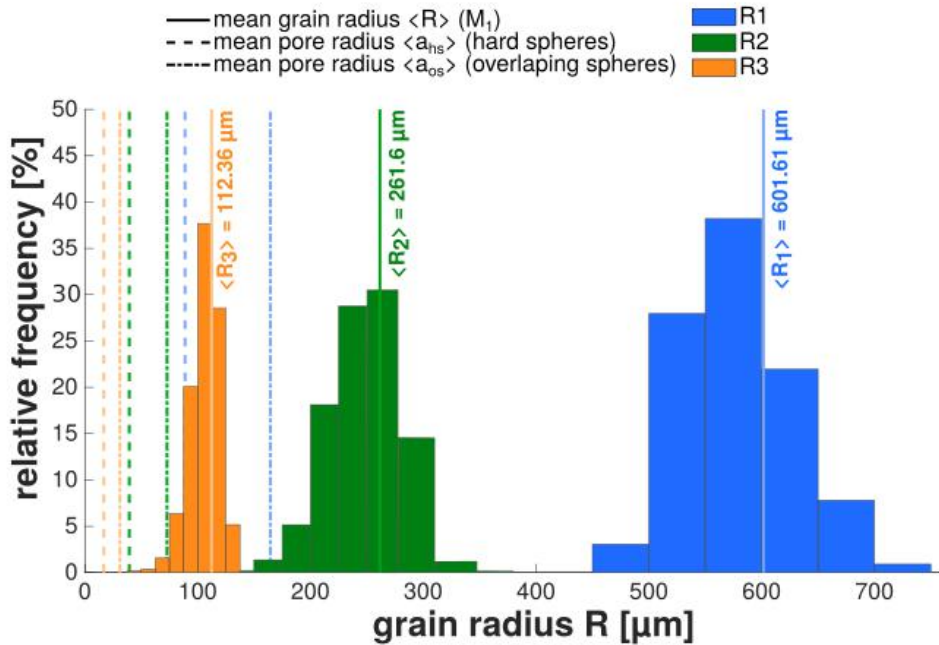
Figure 2.6 Grain radius distributions of the SiLiBeads microspheres used to prepare synthetic samples. The degree of dispersivity S is approximately 0.98 for the three distributions (with S=1 the monodisperse limit).
