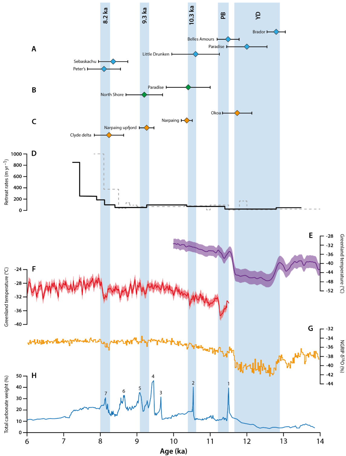
Figure 3.5 (A) Exposure ages of moraine systems of southern Labrador from this study. (B) Exposure ages of moraine systems of Labrador and Québec from Ullman et al. (2016). (C) Exposure ages of moraine systems of LIS outlet glaciers on Baffin Island from Young et al. (2020). Additionally, we used one site from Briner et al. (2007), recalculated in Young et al. (2013). (D) Average retreat rates in southern Labrador reconstructed from this study (black line). Dashed dark gray line is from Dalton et al. (2020). (E) Greenland mean-annual temperatures reconstructed using gas-phase \delta^{15}\text{N-N}_2 measurements (purple – \pm 1\sigma ; Buizert et al., 2014). (F) Greenland mean-annual temperatures reconstructed using gas-phase \delta\text{Ar-N}_2 measurements (red – \pm 2\sigma ; Kobashi et al., 2017). (G) \delta^{18}\text{O} record from NGRIP project (orange; Rasmussen et al., 2014). (H) Total carbonate weight chronology in core MD99-2236 collected on the Cartwright Saddle (blue; Jennings et al., 2015). Vertical bars represent cold intervals discussed in the text. YD: Younger Dryas; PB: Preboreal.
