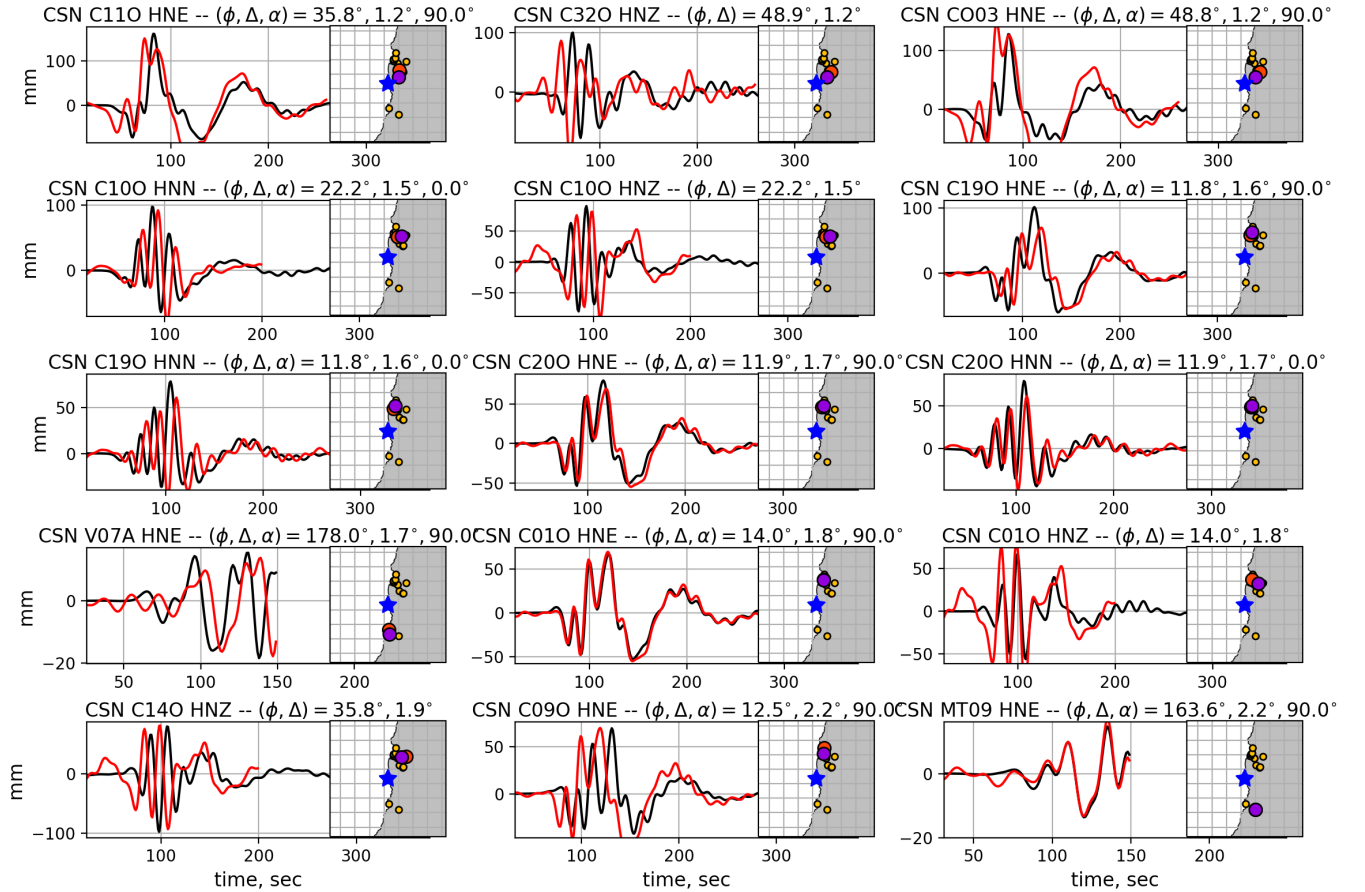
Figure B.1: Comparison between displacements corrected from ground motion records and HRGPS displacements. Red and black waveforms represent HRGPS and strong motion respectively. On the maps, the blue star represents the CSN hypocenter while circles indicate station location (orange for the strong motion station depicted, yellow for the ensemble of strong motion stations, and purple for HRGPS stations). Variation in waveforms is mostly due to differences in colocation.
