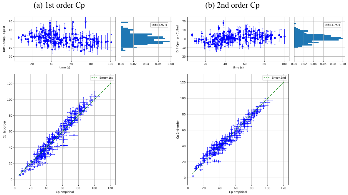
Figure 3.7: Rupture times comparison between different C_p inversion solutions. Comparison between the empirical covariance matrix and the first order (a) and 2nd order (b) approaches.
