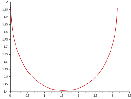
Figure 3.2 – Graph of \ell(x)
