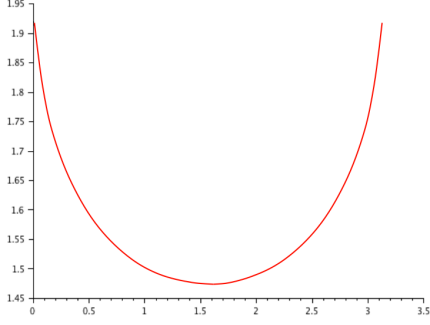
Figure 3.1 – Graph of \ell^{1/2}(x)
