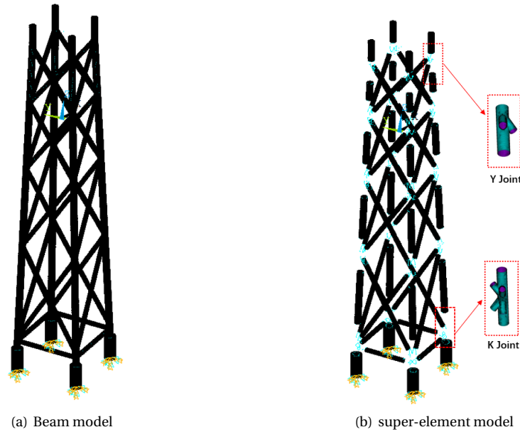
Figure 4.6 – Jacket model
