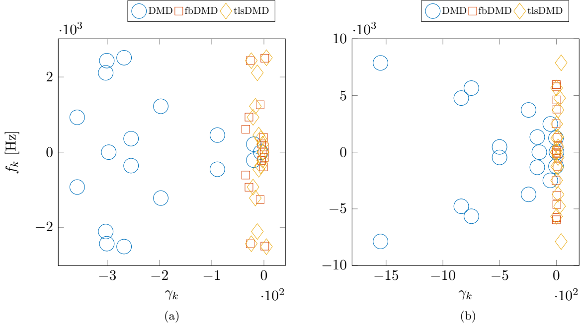
Figure 3.35: Eigenvalues \omega_k = \gamma_k + 2\pi i f_k from three DMD variants (standard, forward-backward and total least-squares) for (a) Lg0 at p_{in} = 2.0 bar and (b) L4 at p_{in} = 1.5 bar.
