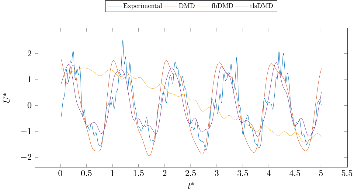
Figure 3.39: Normalized velocity at x/w = 0 and y/w = 12 reconstructed from the standard, forward-backward and total-least-square DMD algorithms (L4 at p_{in} = 1.5 bar). The experimental plot is intentionally cut at t^* for clarity's sake.
