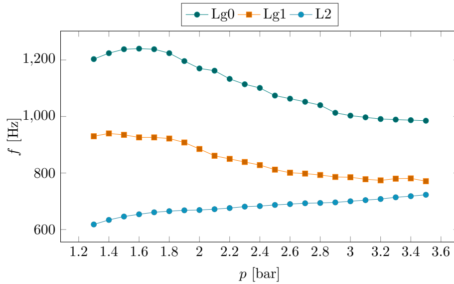
Figure 3.11: Frequency response of the L-prototypes to different inlet pressures.
