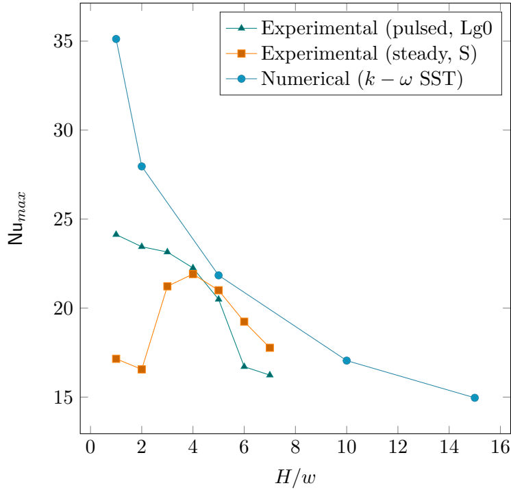
Figure 5.14: Experimental and numerical values of the peak Nusselt number versus standoff distance for p_{\text{in}} = 2.5 bar.
