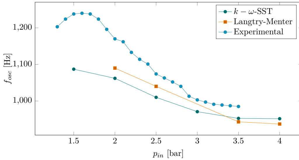
Figure 3.15: Frequency response of Lg0 from numerical results (2D k - \omega SST and Langtry-Menter) and experimental results.
