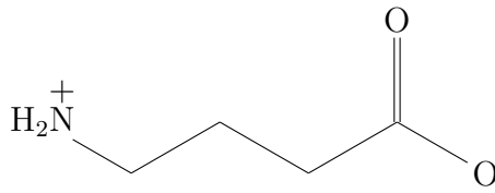
FIGURE 29 – Acide \gamma -aminobutyrique (C 4 H 9 NO 2 )
