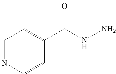
FIGURE 11 – Isoniazide (C 6 H 7 N 3 O)
