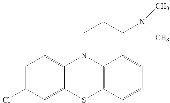
FIGURE 5 – Chlorpromazine (C 17 H 19 ClN 2 S)
