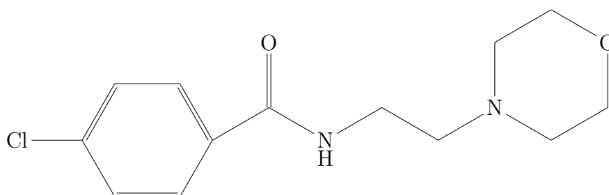
FIGURE 13 – Moclobémide (C 13 H 17 ClN 2 O 2 )
