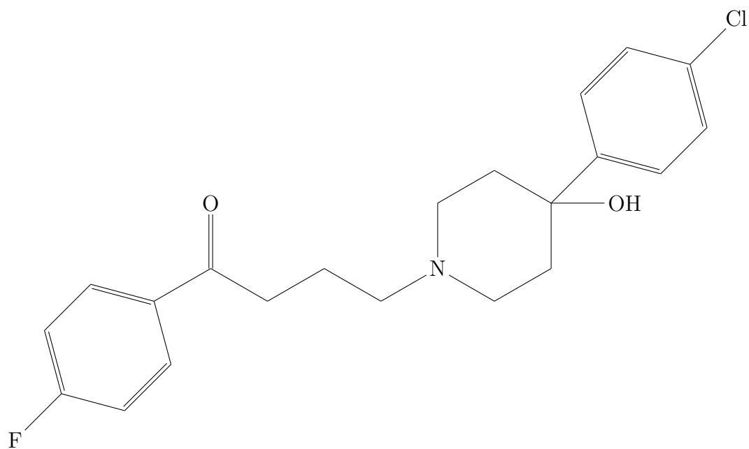
FIGURE 6 – Halopéridol (C 21 H 23 ClFNO 2 )
