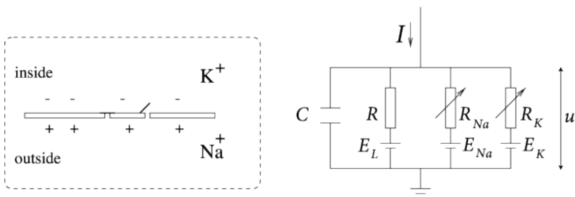
FIGURE 1 – Biophysique des membranes cellulaires (d’après Alan L. HODGKIN et Andrew F. HUXLEY. « A quantitative description of membrane current and its application to conduction and excitation in nerve ». In : The Journal of Physiology 117.4 (1952), p. 500-544
