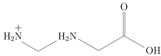
FIGURE 30 – Glycine (C 2 H 5 NO 2 )
