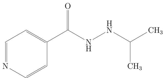
FIGURE 12 – Iproniazide (C 9 H 13 N 3 O)
