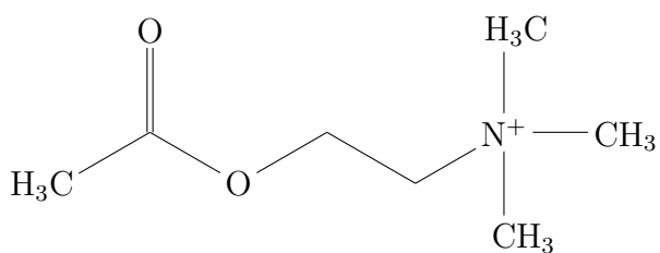
FIGURE 21 – Acétylcholine (C 7 H 16 NO 2 )
