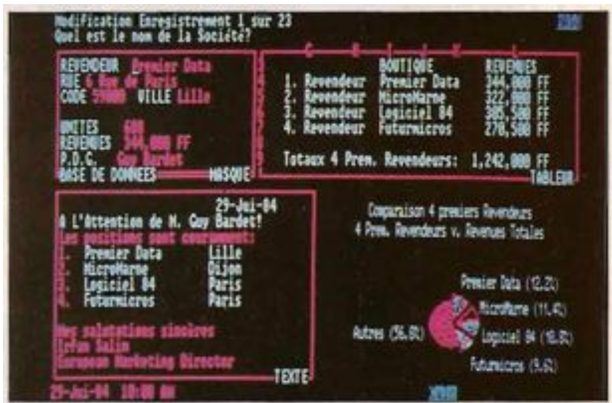
Figure 21. Ecran Symphony 20 .
