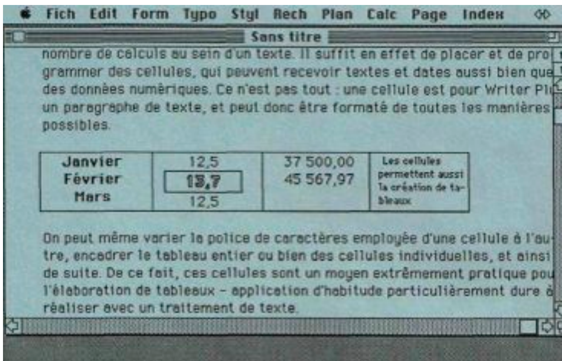
Figure 40. Writer Plus 38 .
