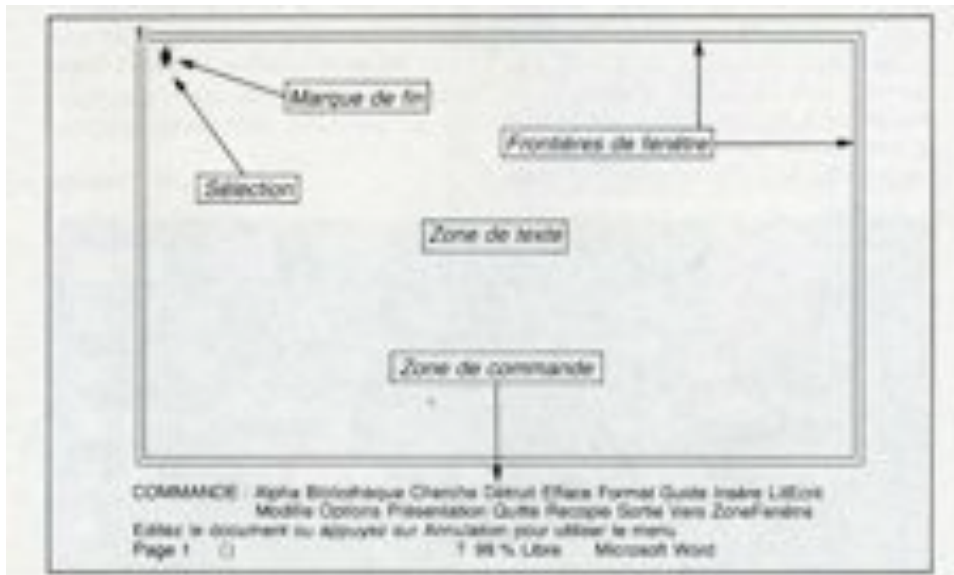
Figure 37. Word 35 .
