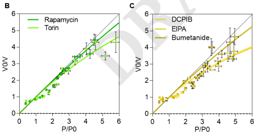
Fig. 7. Supplementary || Cell response to osmotic shocks under drug treatment and kinetic of inhibition of mTOR. A , Dynamics of mTOR inhibition under rapamycin and torin1 treatment. Panels represent activation (phosphorylation) of S6K1 (p-p70) and Akt (pAkt) and loading controls. B , Ponder's relation for rapamycin or Torin1 treated cells. C , Ponder's relation for DCPIB or EIPA or Bumetanide treated cells.
