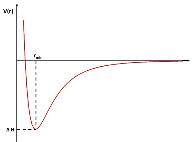
Figure 5. Lennard-Jones potential energy
