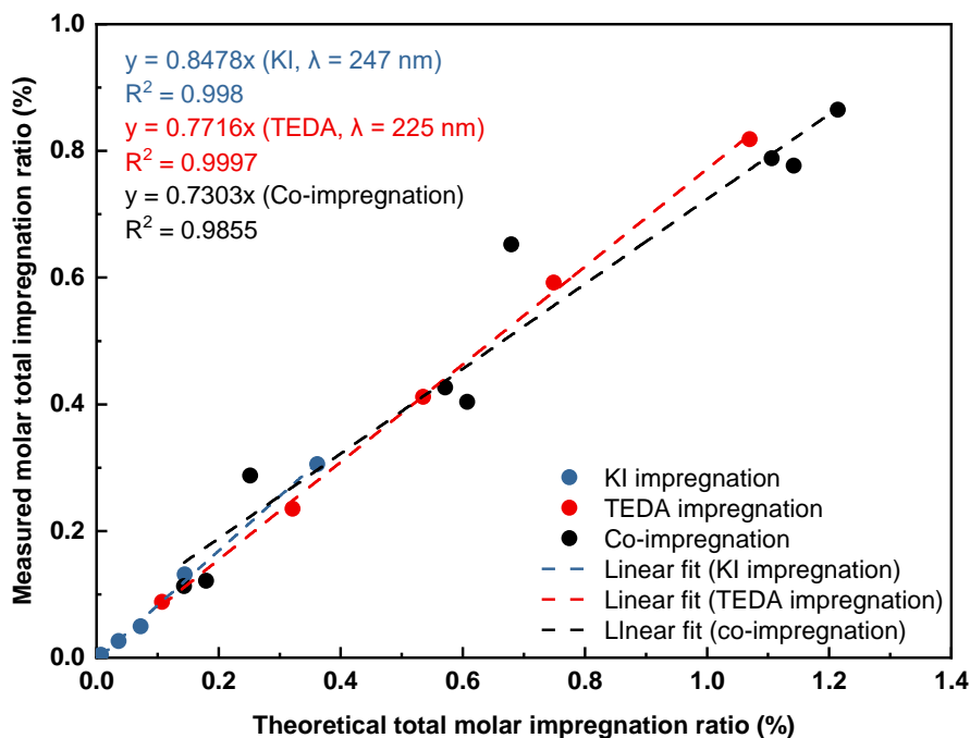
Figure 25. Measured molar impregnation evolution for different AC compared to the “theoretical” impregnation (as reported by the manufacturer)
