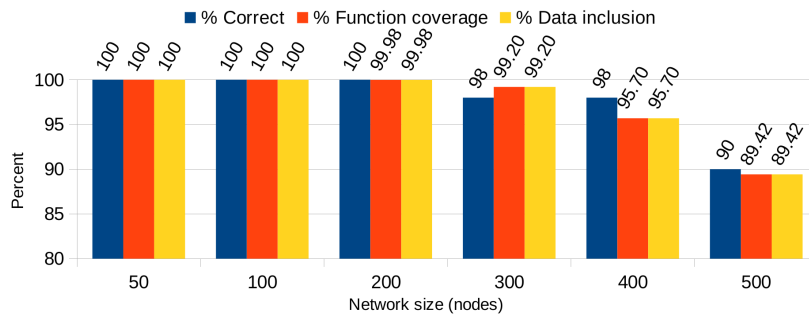
(a) 10,000ms function scope
