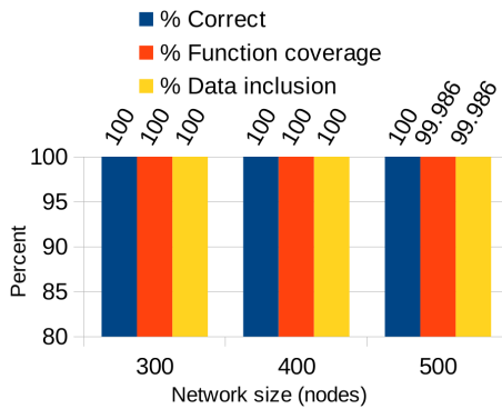
(b) 200,000ms function scope
