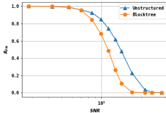
Figure 5.12 - Average evolution of FN rate with SNR . for unstructured sparsity (Joint L_1 ) (blue,"Unstructured") and BlockTree algorithm ( L_{1,2}^B ) (orange,"Blocktree"). BlockTree has a better detection rate than Unstructured sparsity.
