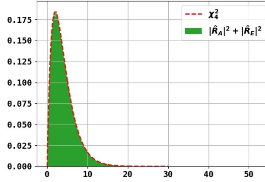
Figure 5.18 – In green is represented the distribution of whitened residuals |\mathcal{A}_S(\mathbf{r})[k]|^2 in Fourier domain. In red is plotted the probability density of the law \chi_4^2 . The residuals manifestly follow the expected law. (Figure extracted from Ref.[10])
