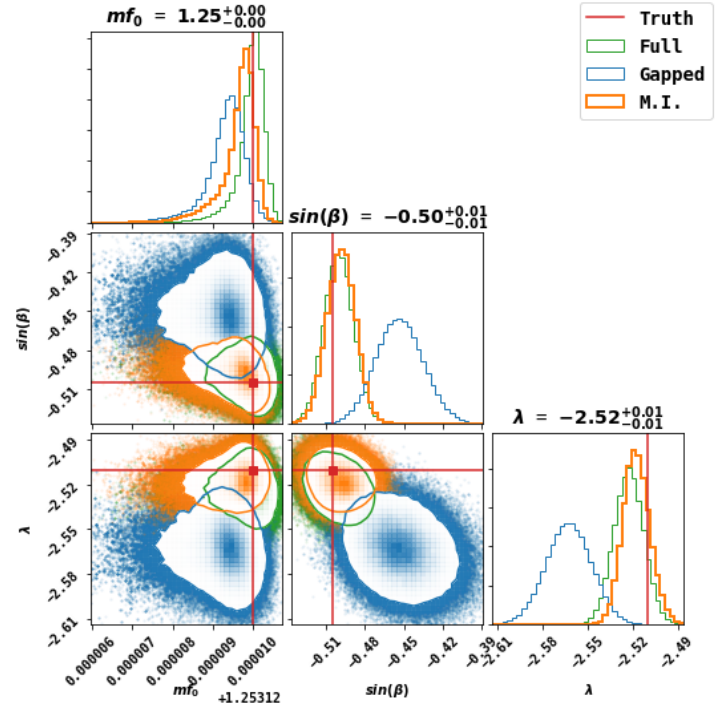
Figure 6.16 – Comparison of the posteriors obtained for a full, ungapped signal (green), a crenel-gapped signal (blue) and an inpainted signal ( orange ). For the gapped and full signal, the posteriors are identical to the one presented in Fig.6.7. The data loss rate is about 28%, combining the three types of gaps. Left : Using classical inpainting. Right : Using modified inpainting. In both cases, the posteriors of inpainted data are really close to the full data posteriors. Using inpainting corrects the impact of the mask on the signal, and thus helps improving the parameter estimation. Using modified inpainting makes the main frequency f_0 estimation a bit harder, as it also adds noise around that frequency. For the sky location, both inpainting methods provide similar results.
