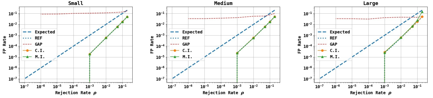
Figure 6.13 – FP rate with rejection rate for real ungapped signal (blue), gapped signal (red), signal inpainted with C.I. (orange) and signal inpainted with M.I. (green) for different types of gaps. Left : Small gaps. Middle : Medium gaps. Right : Large gaps. The FP rate for algorithms C.I. and M.I. is identical to the one obtained for an ungapped signal.
