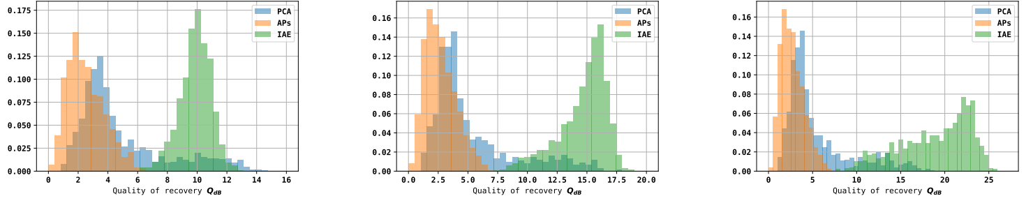
Figure 7.12 – Distribution of quality estimator Q_{dB} for various input SNR for IAE (green), PCA (blue) and APs (orange). Left : SNR = 20 , Middle : SNR = 40 , Right : SNR = 100 . IAE performance improves with the SNR at variance with the two other models.
