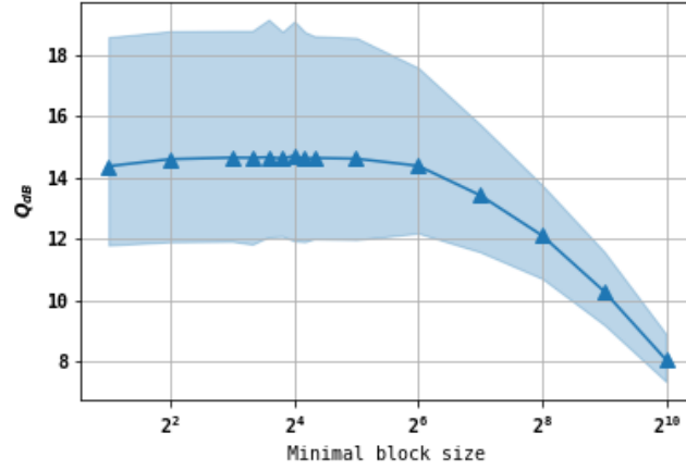
Figure 5.13 – Average quality Q_{dB} of signal recovered using BlockTree for rejection rate \rho_{tree} = 10^{-4} . Input signals have a SNR of 50. There is an operating plateau between |B| = 4 and |B| = 20 . The area filled in light blue shows how 95% of the values are distributed around their average (dark blue line).
