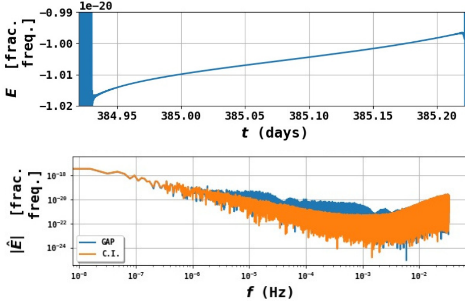
Figure 6.9 – Upper row : Inpainted noise in time domain in a gap for classical inpainting algorithm (C.I.). We only recover noise frequencies for which the correlation length is superior to the gap size. This is not a shortcoming, as Fig.6.1 shows that the PSD deformation is more important for low frequencies than high frequencies. Lower row : Comparison between gapped signal and inpainted signal in frequency domain : the noise spectrum was corrected from the imprint of the gaps. (Figure extracted from Ref.[4])
