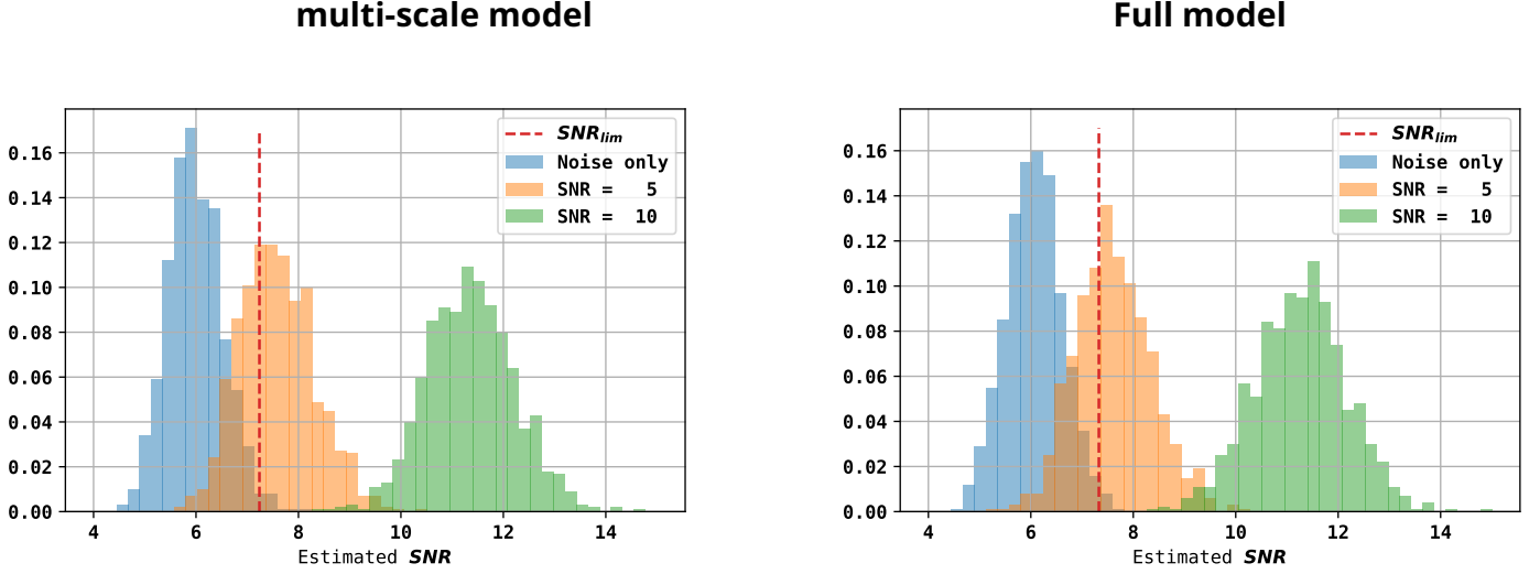
Figure 7.15 – Estimated SNR on IAE output for an input consisting in noise only (blue), in signal with SNR = 5 (orange) and in signal with SNR = 10 (green). The dashed red line shows the limit of detectability set like in Eq.(7.3.7). Left : multi-scale model ; Right : Full model. Both models give coherent results when assessing the detectability threshold.
