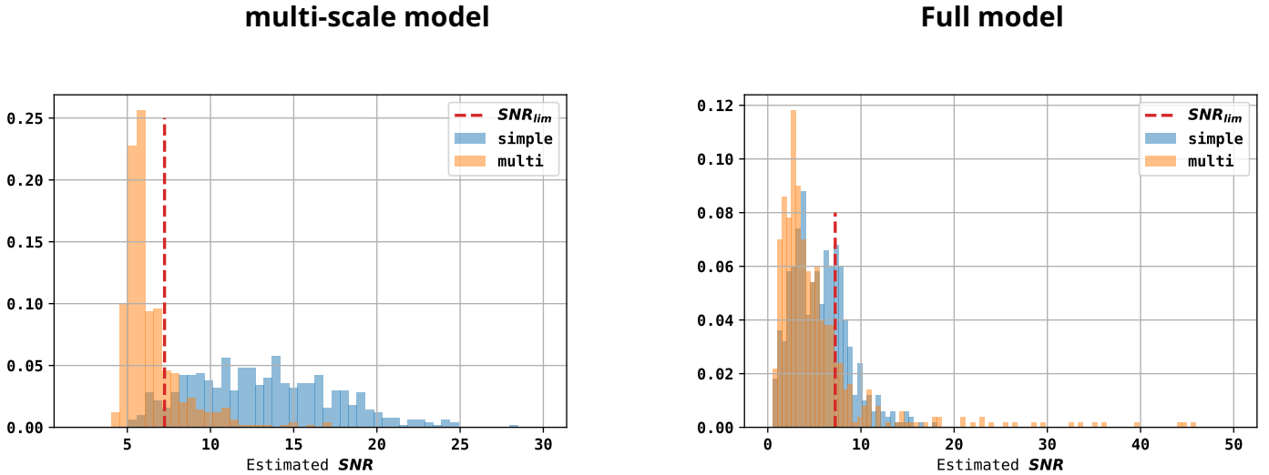
Figure 7.23 – Applying simple BSP on the residuals after subtracting the signal found by either simple BSP (blue) or multi-BSP (orange), we estimate the SNR of the result to check its compatibility with noise. As multi-BSP has a better recovery quality than simple BSP, the residuals better compare to noise.
