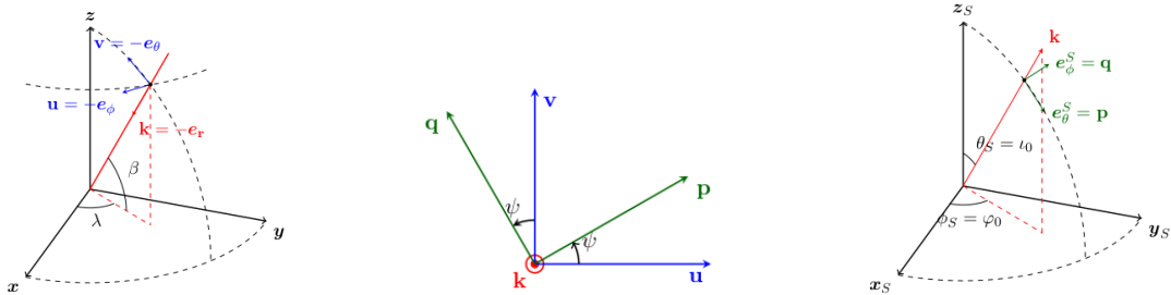
Figure 4.1 – Frame changes between the Solar System Barycenter frame (left) and the source frame (right). This involves a rotation of angle \psi illustrated by the picture in the middle. (Source :[1])
