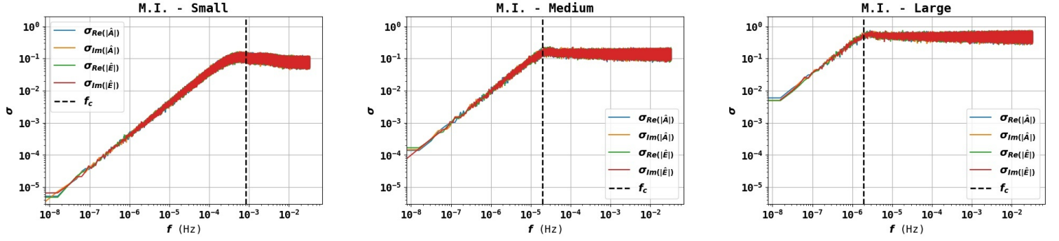
Figure 6.11 – Distribution over 50 samples \mathbf{n}_{\text{samp}} of real and imaginary parts of \mathbf{S}^{-1/2}(f_{CI}(M(\mathbf{n}+\mathbf{n}_{\text{samp}})) - \mathbf{n}_{\text{sample}} - \mathbf{n}) , with \mathbf{n} the input noise (before gaps) and f_{CI}(M(\mathbf{n}+\mathbf{n}_{\text{samp}})) - \mathbf{n}_{\text{sample}} the recovered inpainted noise for M.I. algorithm and sample \mathbf{n}_{\text{samp}} . Left : Small gaps. Middle : Medium gaps. Right : Large gaps. The algorithm acts like a low-pass filter of order 1. The sample that we use in order to fill the gaps only impacts frequencies higher than the cut-off frequency f_c (represented as a dashed black line), which is directly linked to the gap size. The cut-off frequency depends on the gap duration L_{\text{gap}} (in seconds) as : f_c = 1/(2L_{\text{gap}}) . (Figure extracted from Ref.[4])
