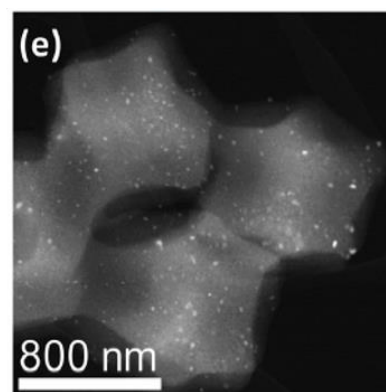
Figure 4: SEM, STEM and TEM images of the different PGM-free materials that will be studied in this work. Images taken from the publications cited in the text.
