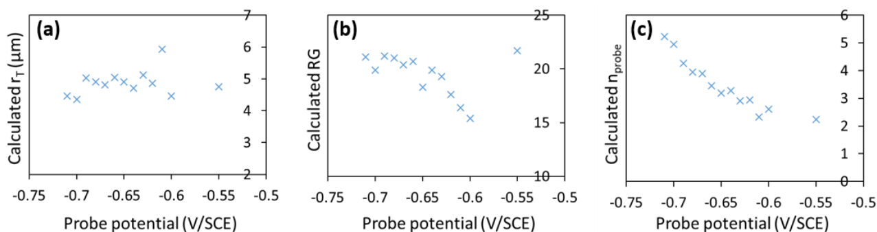
Figure 16: Calculated values of r_T , RG and n_{\text{probe}} from approach curves recorded at different probe potentials
