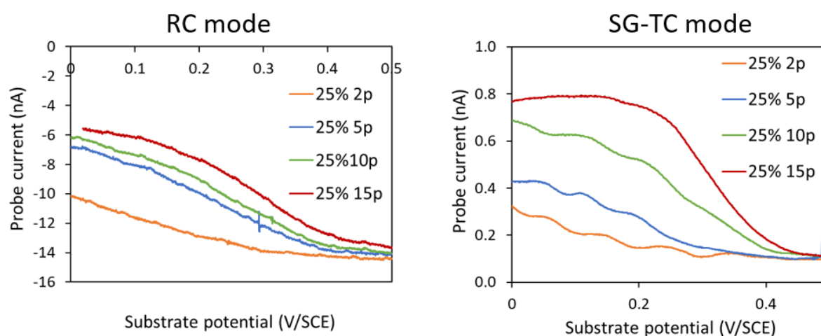
Figure 32: Example of SECM measurements in RC and SG-TC modes (ink dispersed by ultrasonication with 25 % wt of Nafion).
