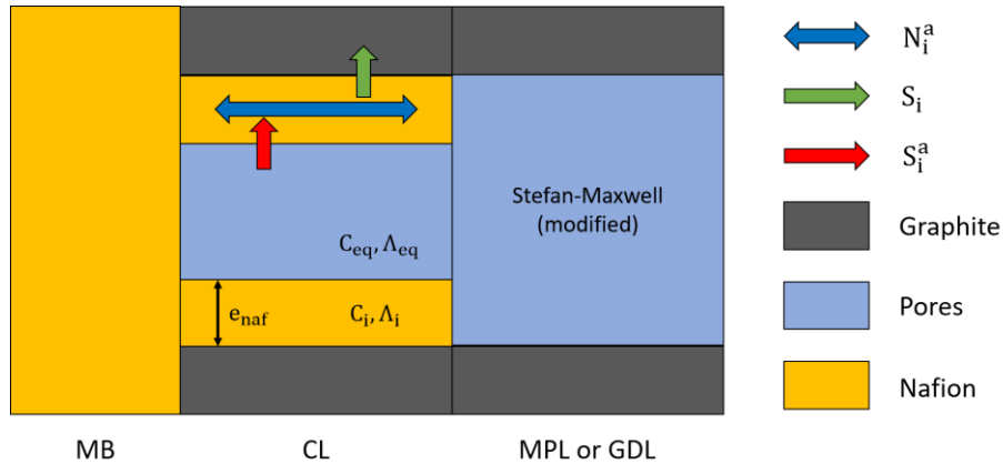
Figure 47: Illustration of the mass balance in the electrolyte phase of the CL. Figure taken from [181].
