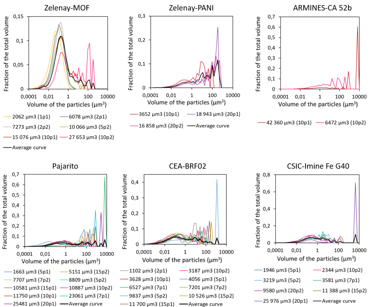
Figure 22: Distributions of particles sizes of the deposits from the different catalysts. An average distribution is shown for each catalyst.
