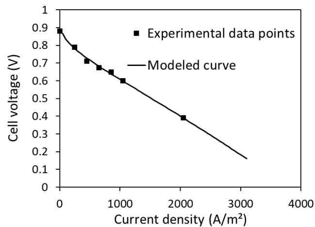
Figure 50: Experimental and modeled polarization curve of the MEA characterization of BRF02 catalyst performed by Heraeus Precious Metals – Hydrogen Systems.
