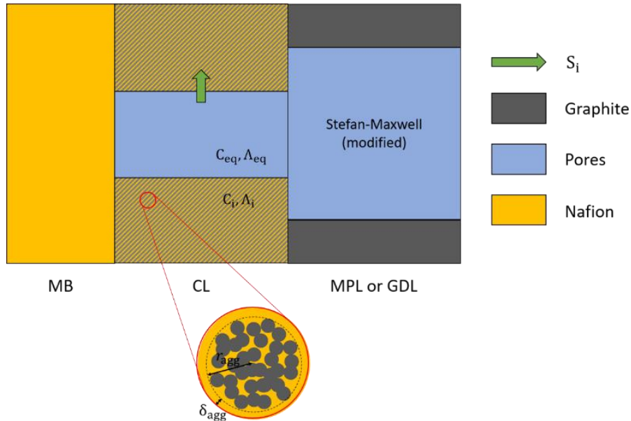
Figure 48: Modeling in the cathodic CL including the agglomerate model.
