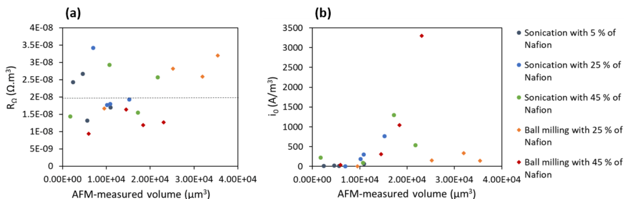
Figure 43: Fitted values of (a) R_{\Omega} and (b) i_0 towards the volume of material for several proportions of Nafion and dispersion methods. The mean value for R_{\Omega} is represented by the dashed line.
