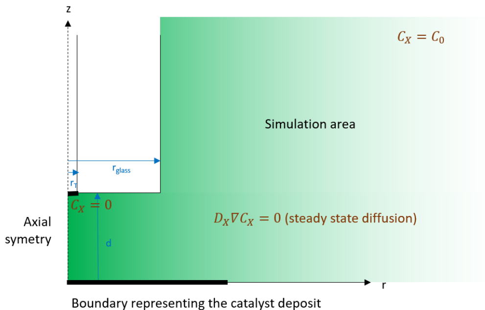
Figure 33: Illustration of the model developed to simulate SECM measurements.
