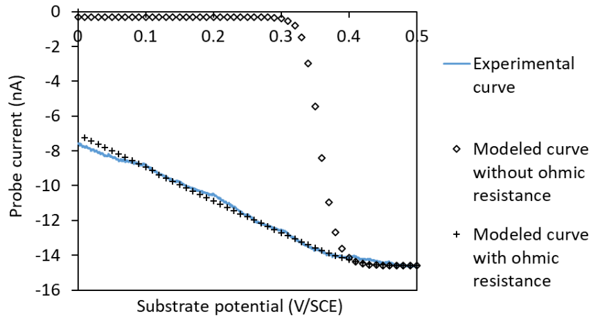
Figure 42: Comparison the model ability to fit an experimental curve with and without the addition of an ohmic resistance.
