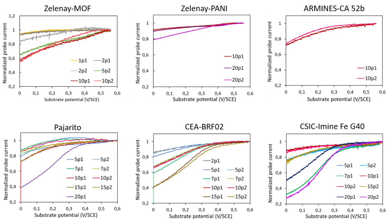
Figure 23: SECM characterization of the deposits from the different catalysts. SECM experiments were performed with a gold probe ( rT \approx 12,5 \mu\text{m} , RG \approx 10 , E_{\text{probe}} = -0.45 \text{ V/SCE} ) in a \text{H}_2\text{SO}_4 50 mM solution saturated with oxygen and a distance probe-substrate of 30 \mu\text{m} . A LSV was applied at the substrate from 0.6 V/SCE to 0 V/SCE with v_{\text{scan}} = 2 \text{ mV/s} . The probe current is normalized by its value at E_{\text{substrate}} = 0.6 \text{ V/SCE} .
