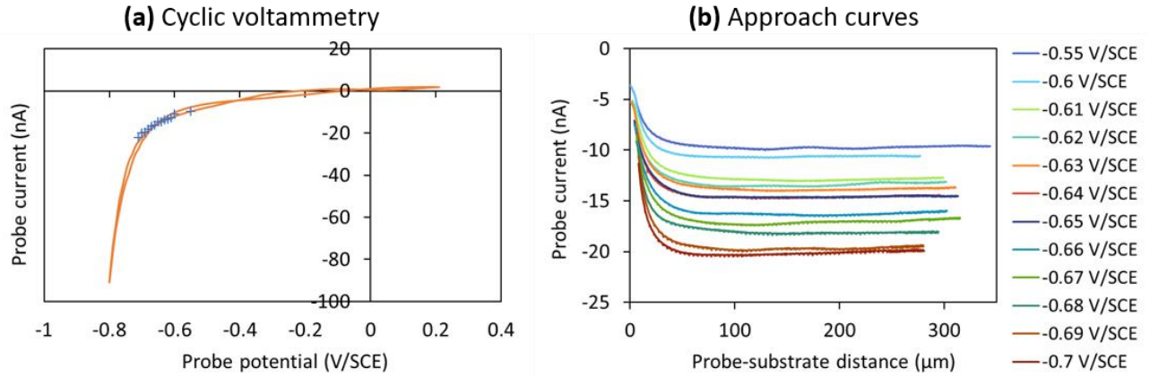
Figure 15: (a) CV from 0.2 V/SCE to -0.8 V/SCE with a scan rate of 10 mV/s, crosses represent the stabilized currents of the approach curves. (b) Approach curves at different probe potentials with a probe-substrate distance from 0 \mu\text{m} to 300 \mu\text{m} and a moving speed of 2 \mu\text{m/s} . (5 \mu\text{m} gold probe in a 0.1 M \text{H}_2\text{SO}_4 solution saturated in \text{O}_2 )
