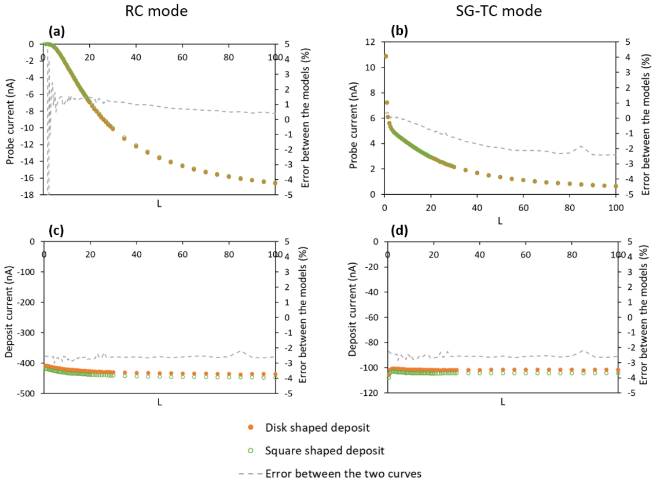
Figure 38: Comparison of the currents calculated at the probe (a and b) and at the catalyst deposit (c and d) in RC mode (a and c) and in SG-TC mode (b and d) for a disk shaped deposit and a square shaped deposit.
