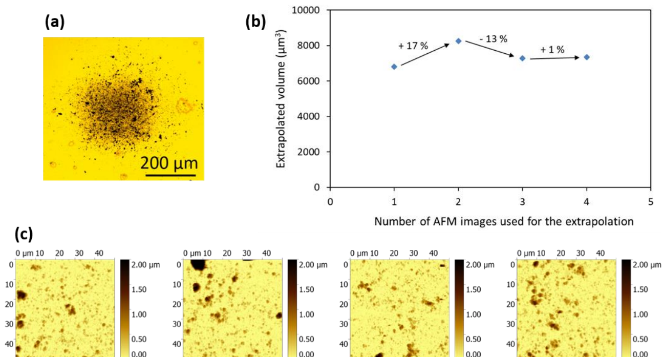
Figure 18: Illustration of how the sufficient number of AFM images is estimated. (a) Optical image of a deposit of catalyst. (b) Evolution of the extrapolated volume towards the number of AFM images acquired. (c) AFM images used for the estimation of the volume of catalyst in the deposit.
