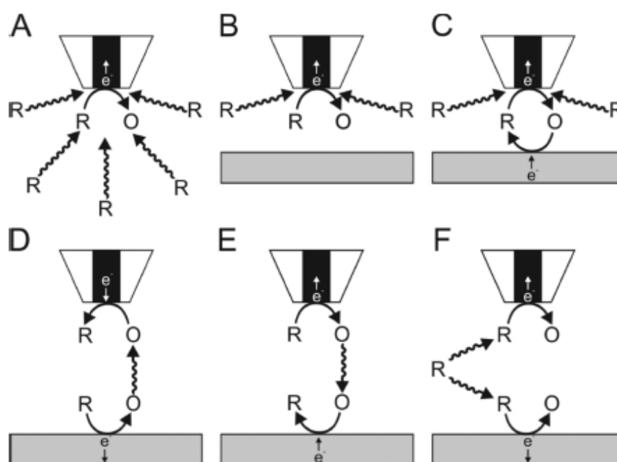
Figure 10: Illustration of the different modes of SECM. (A) UME in bulk solution. (B) Negative feedback. (C) Positive feedback. (D) Substrate generation/tip collection. (E) Tip generation/substrate collection. (F) Redox competition. Figure taken from [79].
