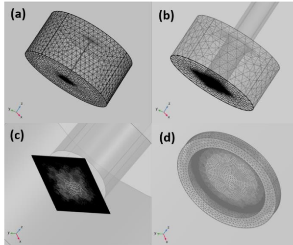
Figure 36 : Meshing of the simulation area for r_T = 5 \mu\text{m} , RG=10 , L=3 , n_T=4 , S_{\text{deposit}} = 200 \times 200 \mu\text{m} . a) Coarse triangles in the bulk domain. b) Refinement around the probe and the catalyst deposit. c) Refinement on the boundaries representing the catalyst deposit and the bottom wall of the probe. d) Refinement on the boundary between the active part and the inactive part of the probe.
