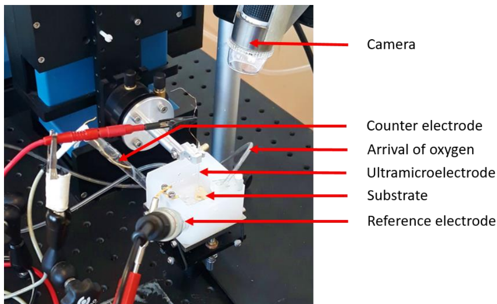
Figure 14: Photography of the SECM set-up.
