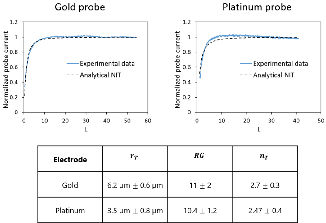
Figure 39: Determination of the parameters of the gold and platinum probe used for the SECM measurements. The values of r_T , RG and n_T are fitted on approach curves in negative feedback mode. The table gives the values averaged on several measurements for each electrode.
