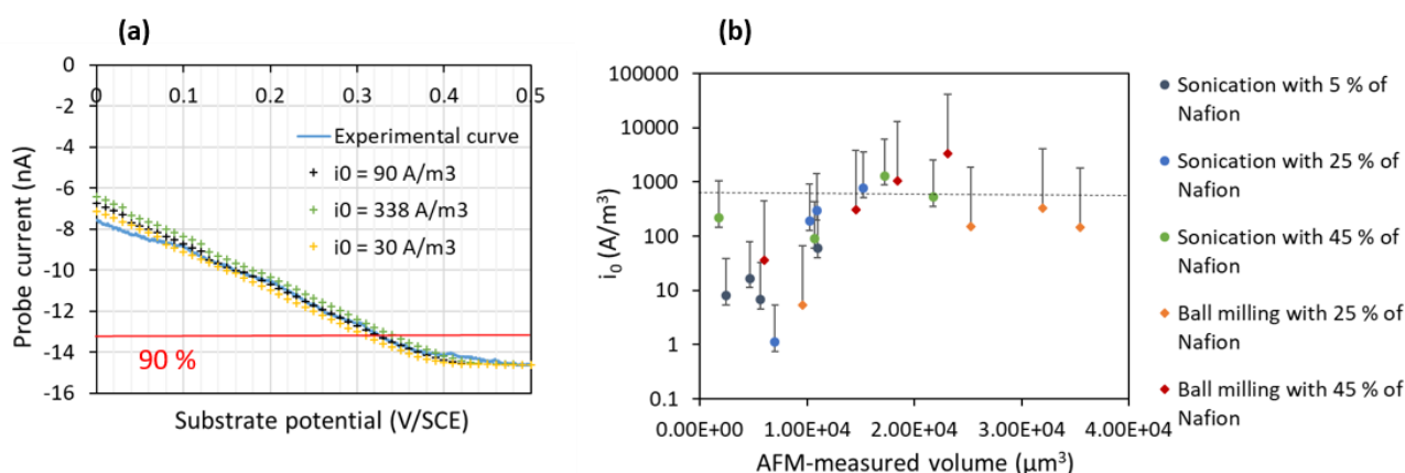
Figure 44: Sensitivity analysis on the parameter i_0 . (a) Determination of the sensitivity for one experiment. (b) Fitted values of i_0 towards the volume of material with error bar corresponding to the parameter sensitivity (logarithmic scale).
