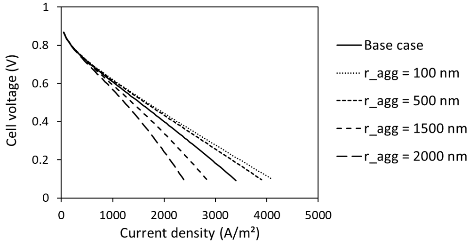
Figure 53: Influence of the agglomerate radius on the cell performance.
