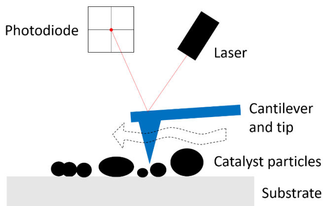
Figure 11: Principle of atomic force microscopy (AFM).
