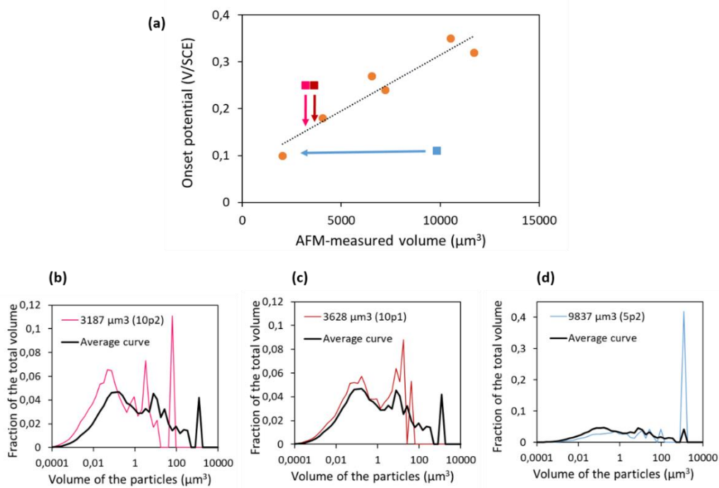
Figure 26: Electrochemical performance of CEA-BRF02 catalyst linked with the agglomeration state of the deposits. (a) Onset potential towards the volume of catalyst. (b), (c) and (d) Distributions of particles sizes of the three points deviating from the trend in (a) and comparison to the average distribution of all the deposits.
