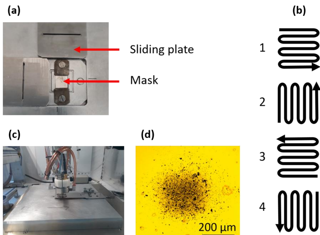
Figure 13: (a) Mask and sliding plates enabling to spray one deposit at a time. (b) Illustration of the path of spraying which consists in the four represented passages sprayed on the same area successively. (c) Sonotek nozzle spraying on the deposition device. (d) Optical image of a deposit obtained with the method developed.
