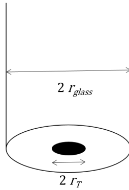
Figure 9: Schematic representation of an ultramicroelectrode.
