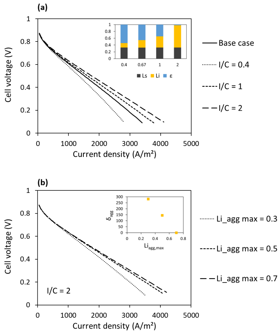
Figure 52: Influence on the cell performance of the amount of ionomer (a) and of its repartition within the agglomerate (b). Insets are showing the composition of the CL in (a) and the thickness of the ionomer layer surrounding the agglomerate in (b).
