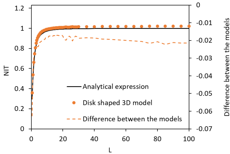
Figure 37: Left axis (points and solid line): negative feedback approach curves calculated with the 3D Comsol model with a disk shaped deposit. Right axis (dashed lines): error to the analytical expression of the two models. r_T=5 \mu\text{m} , R_G=10 , r_C=113 \mu\text{m} and n_T=4 .
