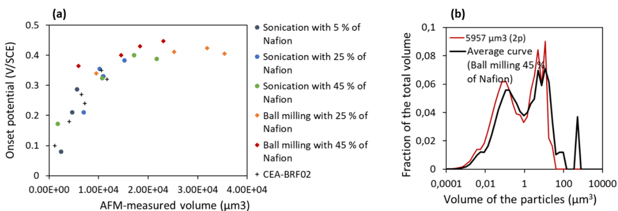
Figure 31: (a) Onset potential of the deposits towards the volume of catalyst. The previously studied series of CEA-BRF02 catalyst is added to the data. Distribution of particles sizes of the point deviating from the tendency, compared to the averaged distributions of the deposits made with the same ink.
