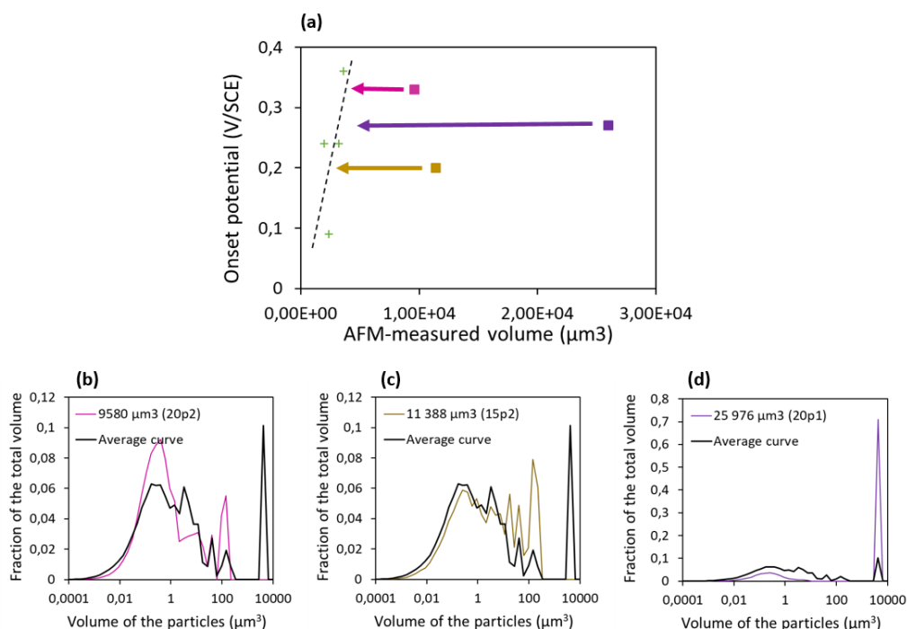
Figure 27: Electrochemical performance of CSIC-Imine Fe G40 catalyst linked with the agglomeration state of the deposits. (a) Onset potential towards the volume of catalyst. (b), (c) and (d) Distributions of particles sizes of the three points deviating from the trend in (a) and comparison to the average distribution of all the deposits.
