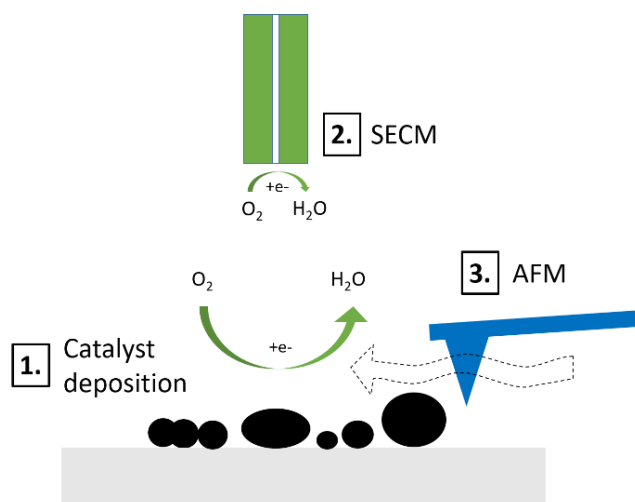
Figure 12: Illustration of the method consisting in combining SECM and AFM characterizations for the study of a catalyst electrochemical activity linked with its agglomeration state.
