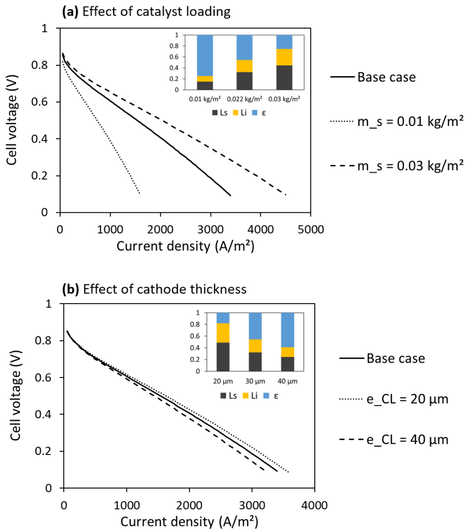
Figure 51: Influence of (a) the catalyst loading and (b) the cathodic CL thickness on the cell performance. The CL composition for each case is presented in the insets.
