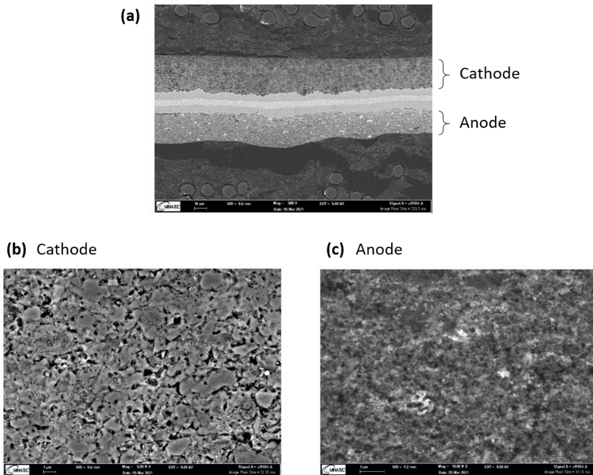
Figure 49: SEM imaging of the MEA used to validate the numerical model. (a) Zoom on the CL and the membrane. (b) Zoom on the cathode CL. (c) Zoom on the anode CL.
