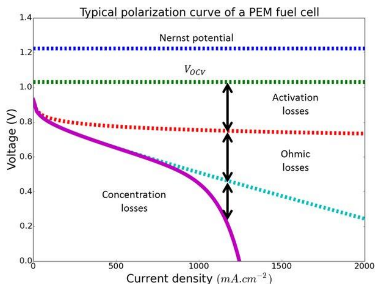
Figure 7: Visualization of the different physical phenomena visible on a polarization curve. Figure taken from [50].
