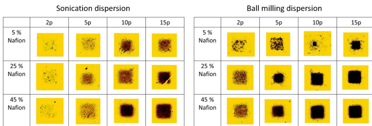
Figure 29: Microscope images of deposits obtained with inks prepared by two different dispersion methods and with three different Nafion contents.
