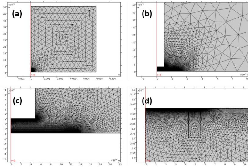
Figure 34: Meshing of the simulation area for r_T = 5 \mu\text{m} , RG=10 , L=3 , r_C = 113 \mu\text{m} . a) Coarse triangles in the bulk domain. b) Refinement around the probe and the catalyst deposit. c) Refinement on the boundaries representing the catalyst deposit and the bottom wall of the probe. d) Refinement on the boundary between the active part and the inactive part of the probe.
