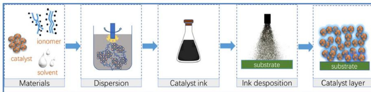
Figure 5: Illustration of the fabrication process of catalyst layer. Figure taken from [39].
