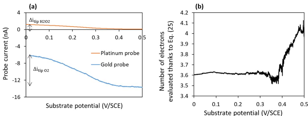
Figure 40: (a) Example of SECM measurements for the determination of the number of electrons exchanged at the probes (gold and platinum). Gold probe: r_T \approx 6.2 \mu\text{m} , R_G \approx 11 , E_{\text{probe}} = -0.65 \text{ V/SCE} . Platinum probe: r_T \approx 3.5 \mu\text{m} , R_G \approx 10.4 , E_{\text{probe}} = 0.9 \text{ V/SCE} . Experiments done in a \text{H}_2\text{SO}_4 0.1 M solution saturated with oxygen and a distance probe-substrate of 30 \mu\text{m} . A LSV was applied at the substrate from 0.5 V/SCE to 0 V/SCE with v_{\text{scan}} = 2 \text{ mV/s} . (b) Evaluation of n_c for the experiment presented in (a) according to Eq. ( 25 ).
