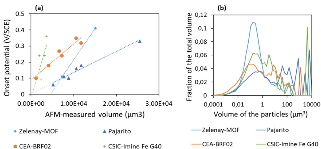
Figure 28: Comparison of (a) the electrochemical performances and (b) the distributions of particles sizes of the four exploitable catalysts.
