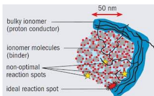
Figure 6: Illustration of the structure of an agglomerate.
