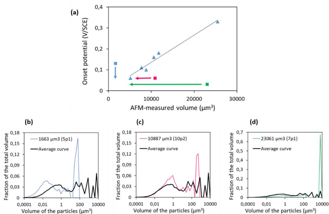
Figure 25: Electrochemical performance of Pajarito catalyst linked with the agglomeration state of the deposits. (a) Onset potential towards the volume of catalyst. (b), (c) and (d) Distributions of particles sizes of the three points deviating from the trend in (a) and comparison to the average distribution of all the deposits.
