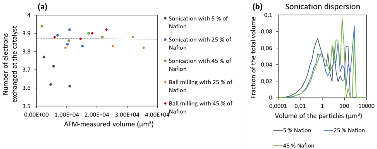
Figure 41: (a) Calculated values of n_c towards the volume of material for several proportions of Nafion and dispersion methods. (b) Distributions of particles sizes of the deposits prepared by sonication.
