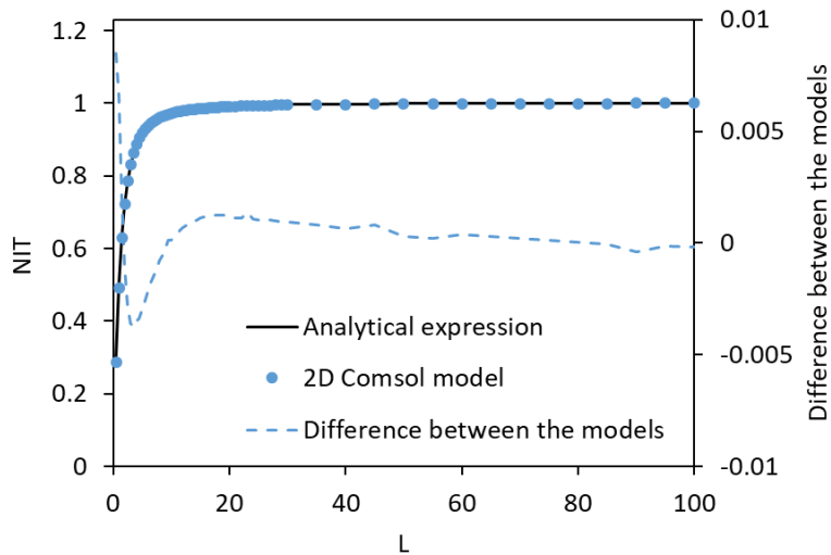
Figure 35: Left axis (points and solid line): negative feedback approach curves calculated with the Comsol model and with the analytical expression from [69]. Right axis (dashed line): difference between the two curves. r_T = 5 \mu\text{m} , RG = 10 , r_C = 113 \mu\text{m} and n_T = 4 .
