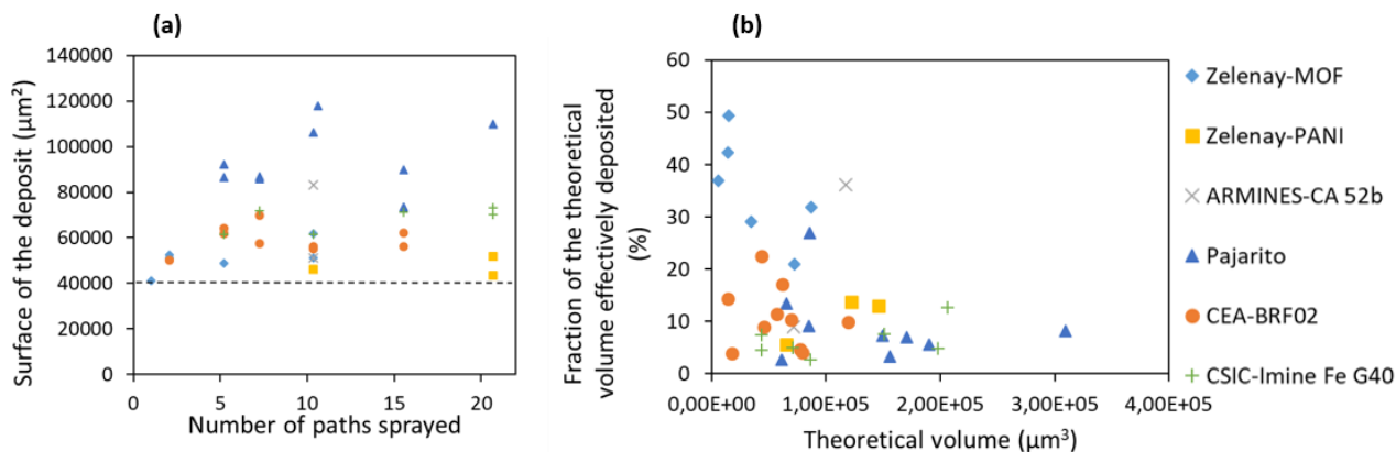
Figure 21: (a) Surface of the deposits, the dashed line represents the surface of the mask. (b) Fraction of the theoretical sprayed volume that was effectively deposited on the substrate.
