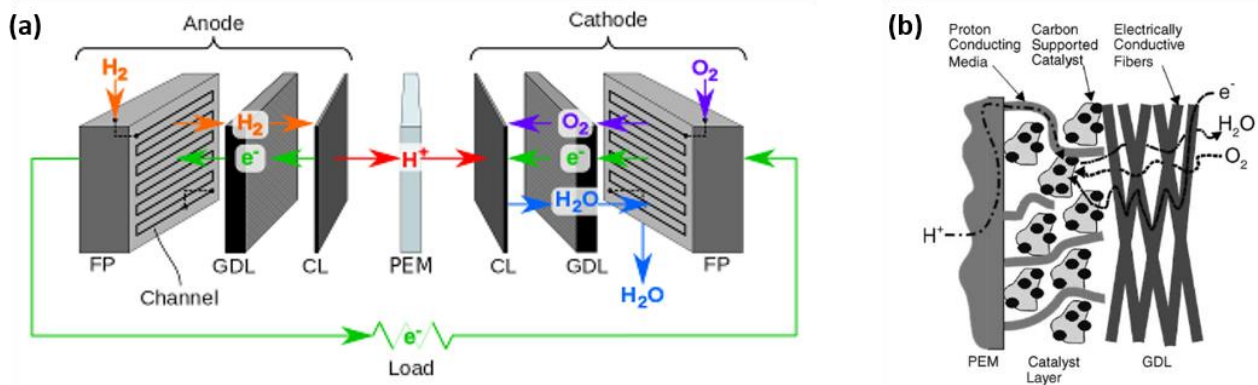
Figure 2: (a) Schematization of a PEMFC fuel cell. (b) Focus on the catalyst layer structure.
