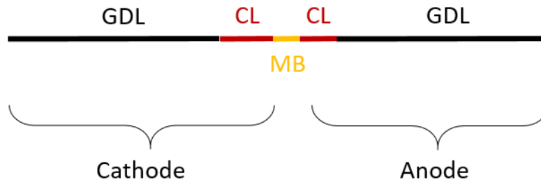
Figure 46: Geometry of the 1D EuROPIUM model. The GDL dimensions are not to scale.
