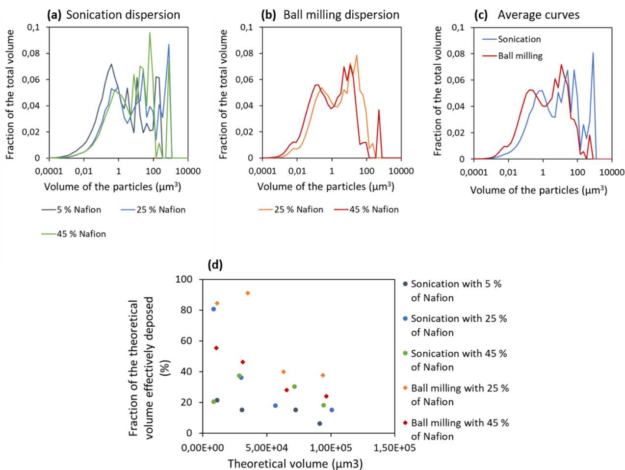
Figure 30: (a) and (b) Distributions of particles sizes for deposits obtained with inks prepared with different dispersion methods and different proportions of Nafion. (c) Distributions obtained by averaging the curves at different Nafion content for each dispersion method. (d) Fraction of the theoretical sprayed volume that was effectively deposited on the substrate.
