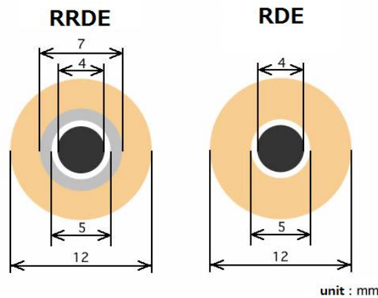
Figure 8: Illustration of the RDE and the RRDE.
