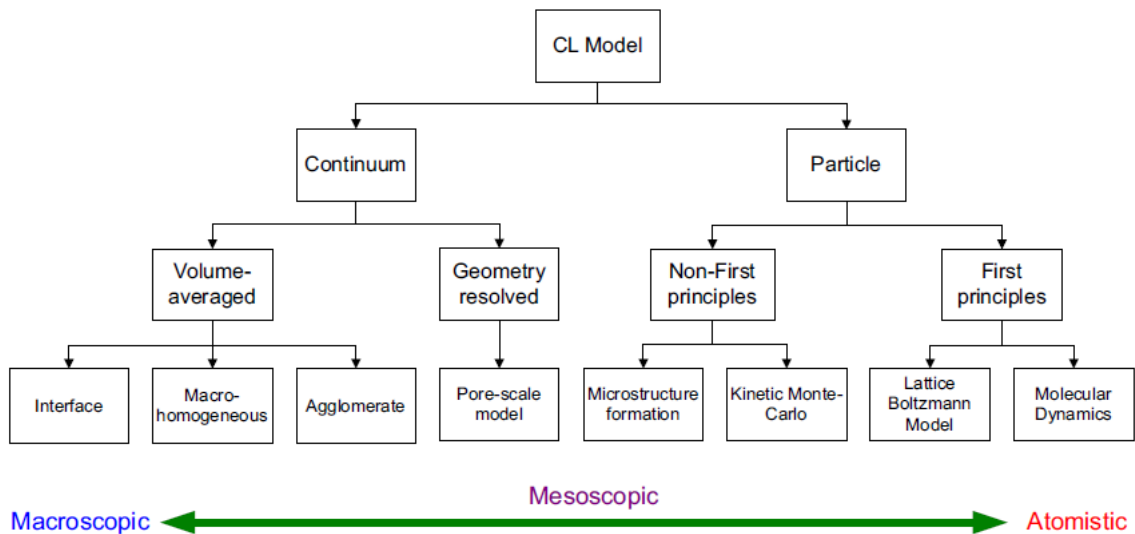
Figure 45: Classification of the different models for describing the CL structure. Figure taken from [174].
