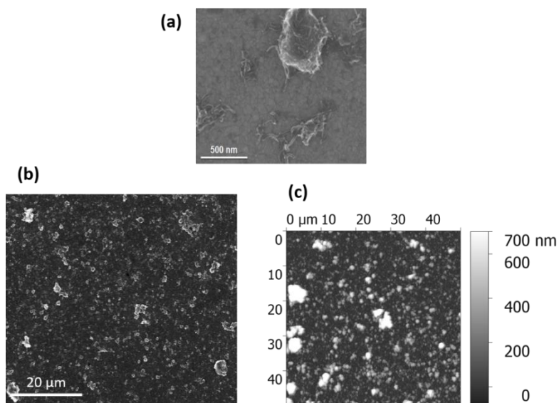
Figure 17: (a) SEM image of some of the smallest particles that can be found in the sample. (b) SEM image taken within a deposit of CEA-BRF02 catalyst. (c) AFM image taken within the same deposit. (b) and (c) show a similar distribution of particles, which confirms that AFM captures correctly the different sizes of particles.
