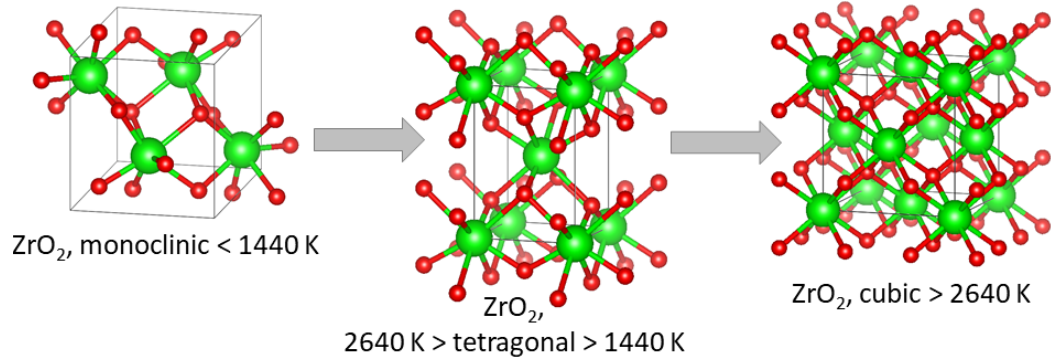
Figure 1.6: Crystallographic structures of Zirconia. From left to right and by increasing temperature: ZrO_2 is monoclinic at room temperature, tetragonal between temperatures of 1440 and 2640 K, and cubic (FCC) above 2640 K. Zr atoms are represented in green and O atoms in red.
