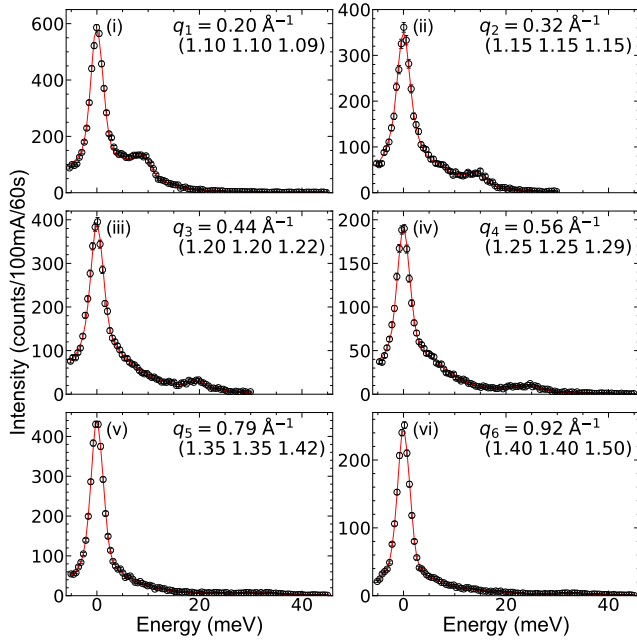
FIG. S9: Energy scans at constant Q for the \Lambda(\text{LA}) polarization, measured by inelastic X-ray scattering on the backscattering beamline ID28@ESRF at 300 K, are plotted as open black circles. The phonon was fit as a damped harmonic oscillator and the fit is shown in red.
