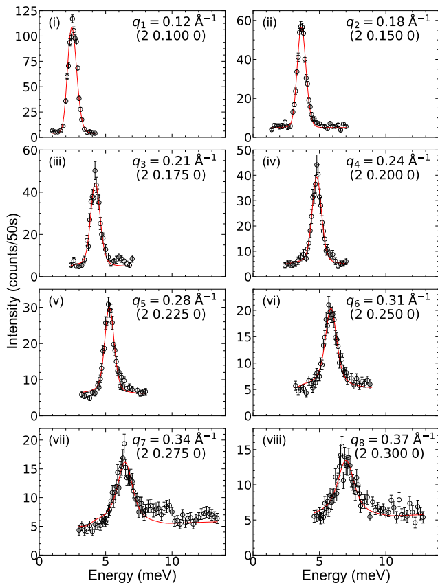
FIG. S3: Energy scans at constant Q for the \Delta (TA) polarization, measured by inelastic neutron scattering on the cold-neutron triple-axis spectrometer 4F2@LLB at 300 K, are plotted as open black circles. The phonon was fit as a damped harmonic oscillator and the fit is shown in red.
