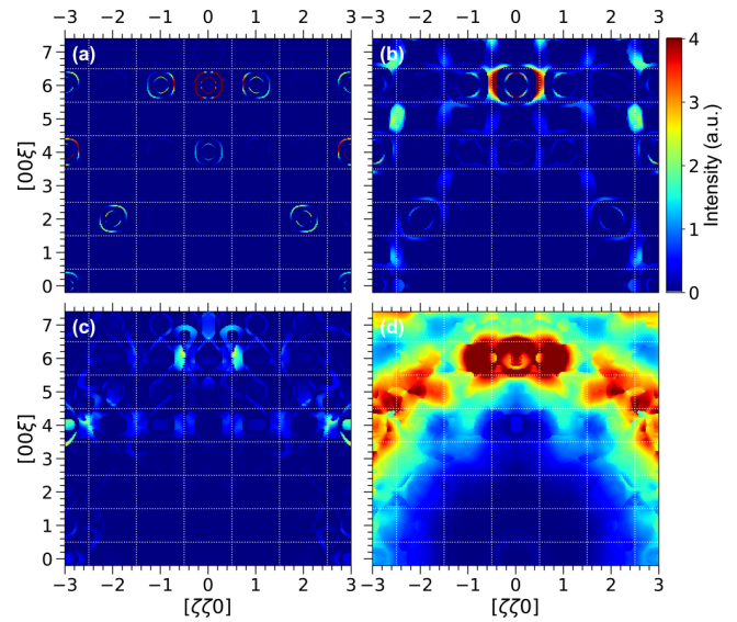
FIG. 6. Simulated two-dimensional neutron scattering function, S(\mathbf{Q}, \omega) , at fixed energy transfer in the momentum plane ([110];[001]) for an ideal ordered model of a type-I clathrate with the composition \text{Ba}_8\text{Ge}_{40}\text{Au}_6 . The first three energy integrations (a)–(c) were taken at 3.5 \pm 0.15 , 4.8 \pm 0.15 , and 6.5 \pm 0.15 meV, respectively. (d) represents a larger integration interval of 9.5 \pm 2.5 meV. The intensity in each map has been normalized to the same intensity scale, which is reflected in the color bar. Dashed white grids show the borders of the Brillouin zones.
