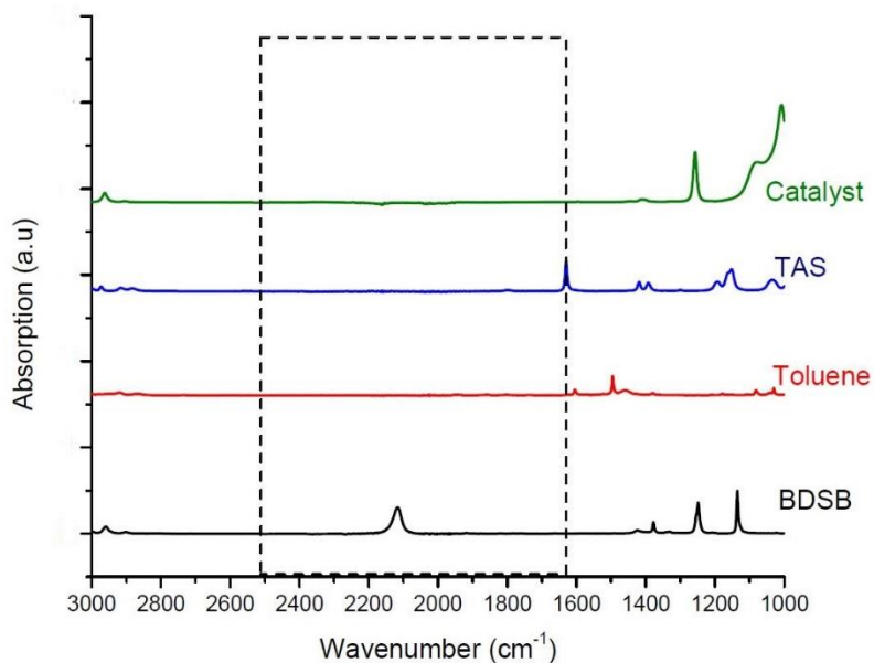
Figure 2.16. IR spectra of Karstedt's catalyst, TAS, toluene and BDSB.
