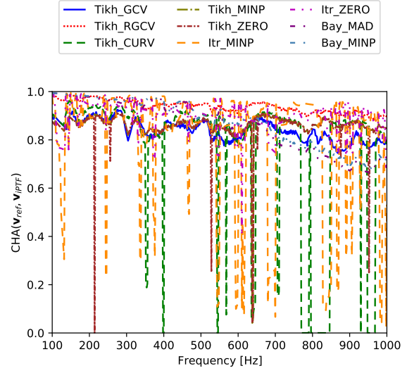
(b) u-iPTF \mathcal{CHA}
