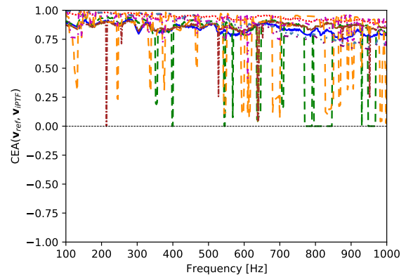
(f) u-iPTF \mathcal{CEA}
