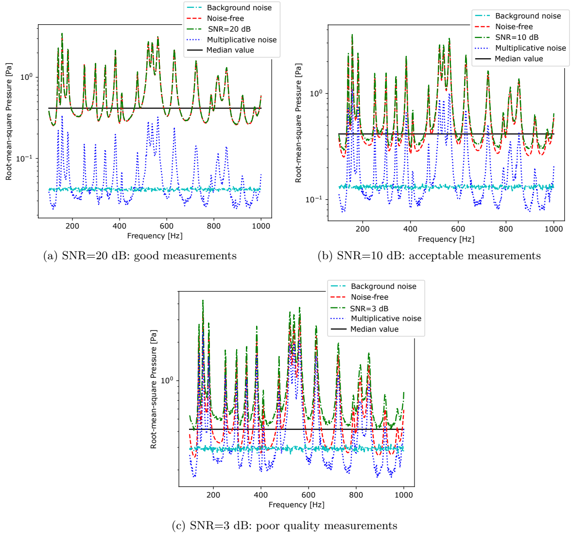
Figure 4.20: Root-mean-square (rms) spectra of the noised acoustic measurement according to [232]
