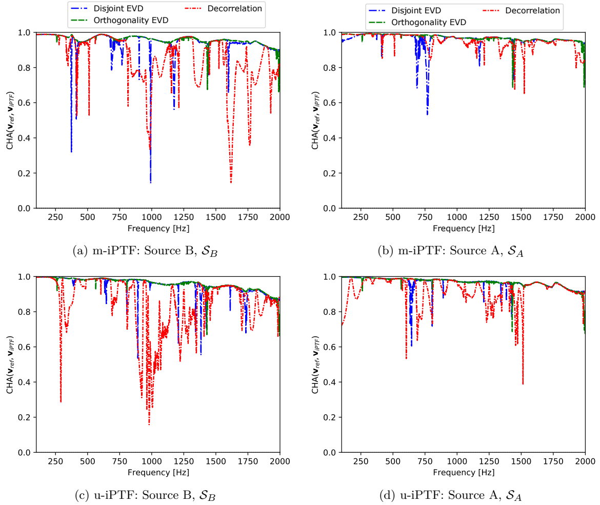
Figure 7.9: Plots of \mathcal{CHA} correlation metric used in the comparison of the separated sources' velocity identified by BSS-iPTF and source velocity computed on the plate (reference) for the full frequency spectrum of study.
