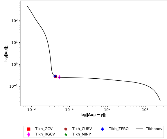
(b) u-iPTF: Tikhonov based methods
