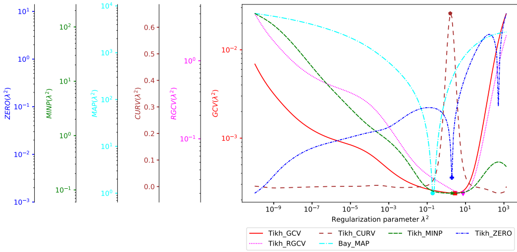
(a) m-iPTF: \lambda^2_{opt} selection criteria for Tikhonov regularization
