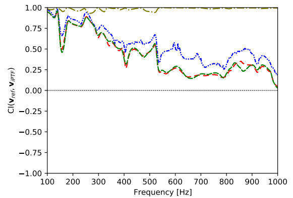
(f) u-iPTF CI fp = 240
