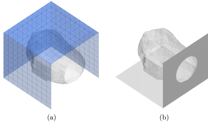
Figure 6.4: Virtual surfaces delimiting the virtual acoustic volume. (a) virtual surface patch mesh and (b) rigid surfaces not discretized into patches. The transparent shape of the e-motor is drawn to see the layout of the surfaces in relation to the e-motor.
