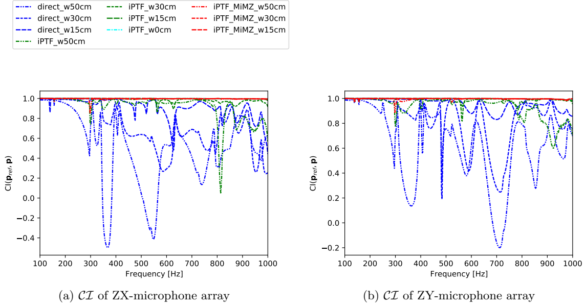
Figure 5.22: Evaluation of the similarities of different directivity patterns compared to the directivity pattern computed without masking object. The \mathcal{CI} metric is used to evaluate the similarity on the 101 points of the semi-circular array. "direct" means that the directivity to be compared to is computed with the presence of the masking object and without the use of iPTF results. "MiMZ" means "Measurement in the masked zone".
