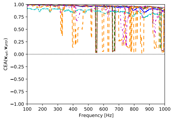
(e) m-iPTF \mathcal{CEA}
