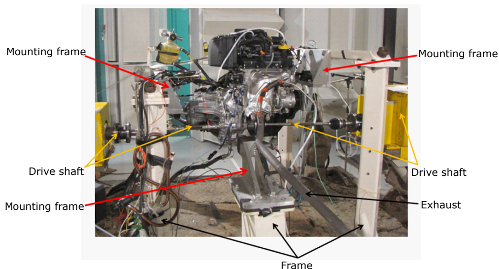
Figure 5.1: Engine test-bench with various masking structures [27].
