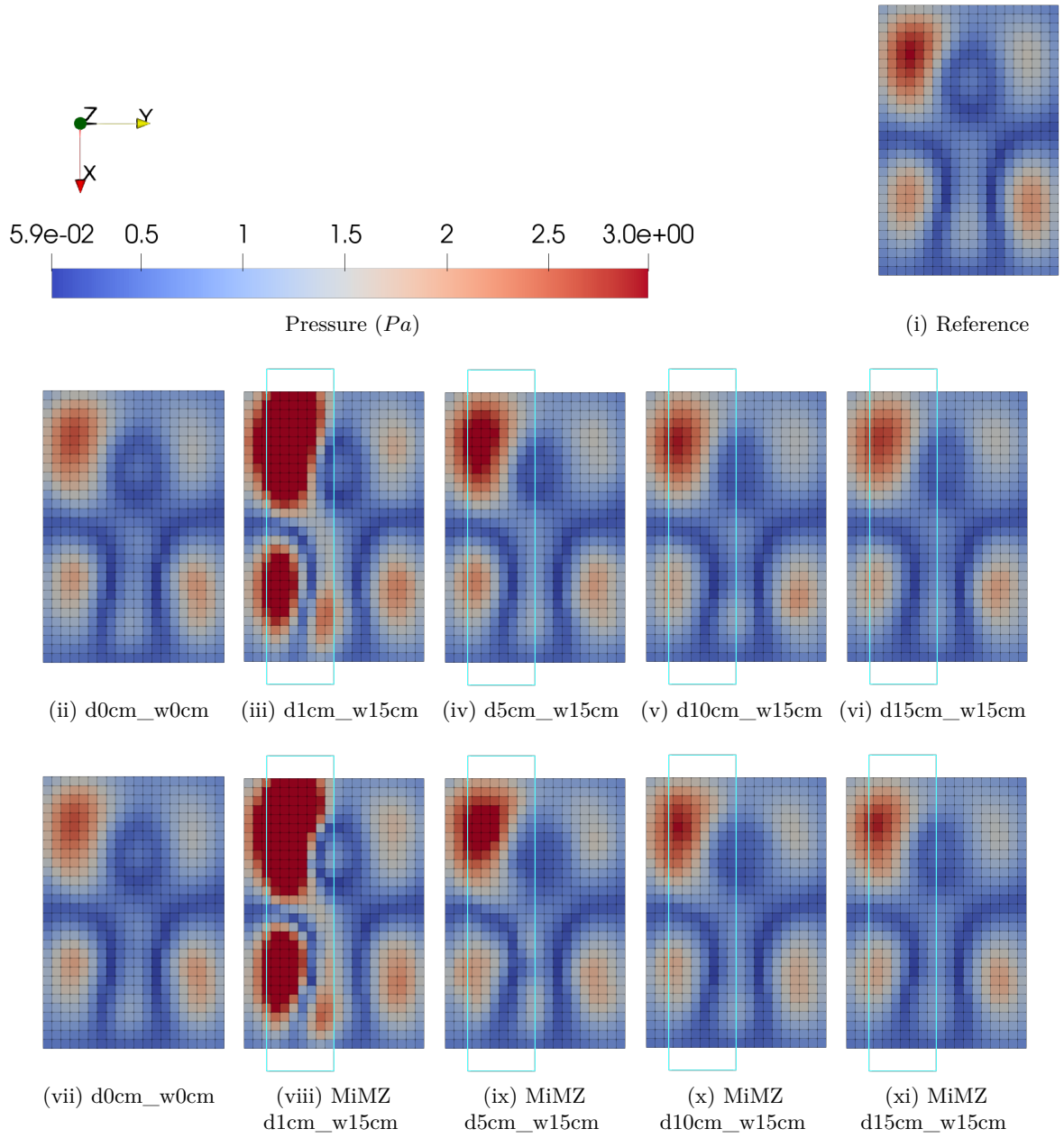
Figure 5.9: Spatial colormap of the amplitude of the acoustic pressure field on the surface of the plate identified with u-iPTF using Tikh_RGCV and the reference computed results at a frequency of 332 Hz for different masking object distance test set-ups. Outline position of the masking object is shown by the cyan-colored rectangle and the acronym MiMZ indicates 'Measurement in Masked-Zone'.
