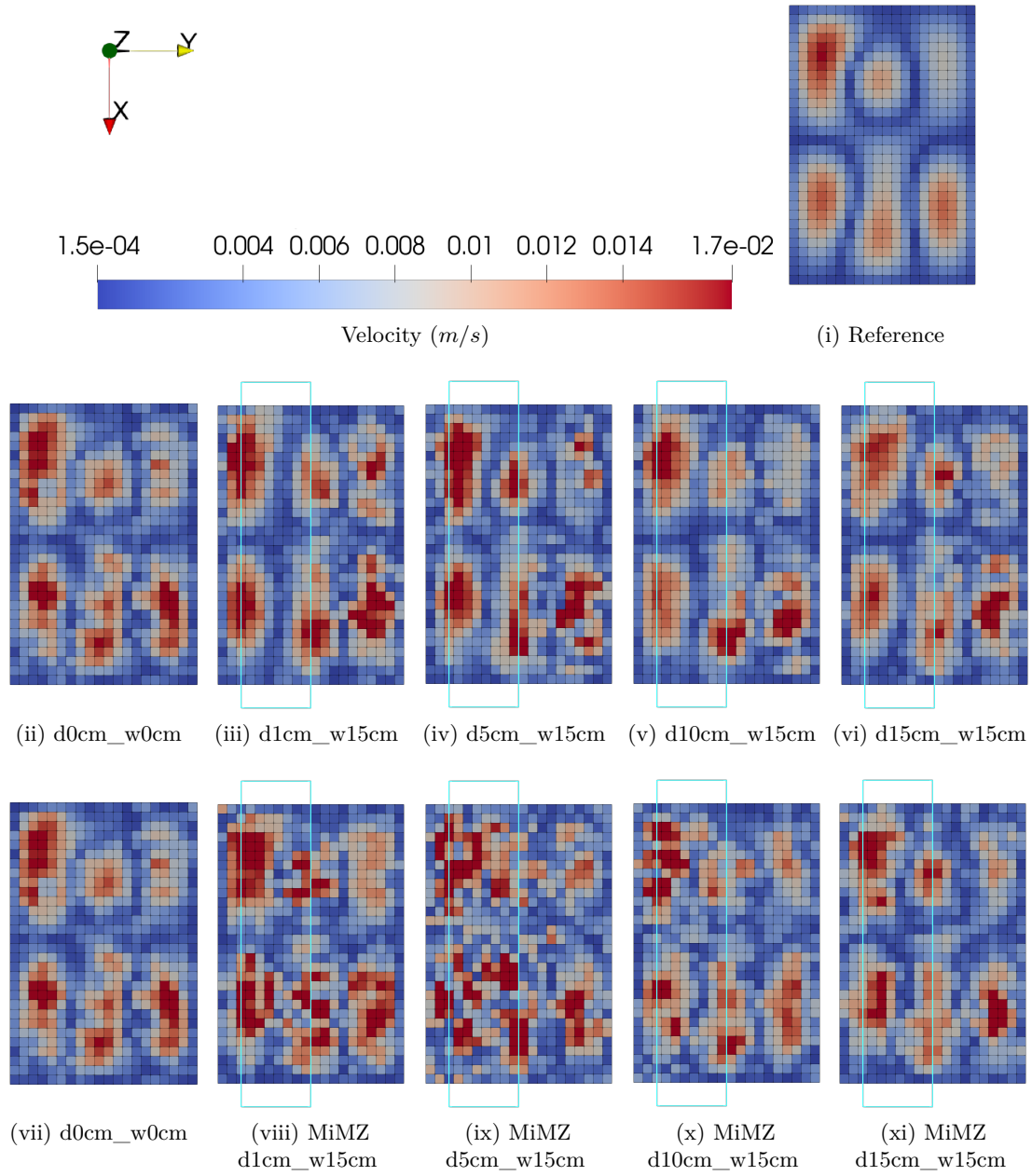
Figure 5.8: Spatial colormap of the amplitude of the acoustic velocity field on the surface of the plate identified with u-iPTF using \text{Tikh\_RGCV} and the reference computed results at a frequency of 332 Hz for different masking object distance test set-ups. Outline position of the masking object is shown by the cyan-colored rectangle and the acronym MiMZ indicates 'Measurement in Masked-Zone'.
