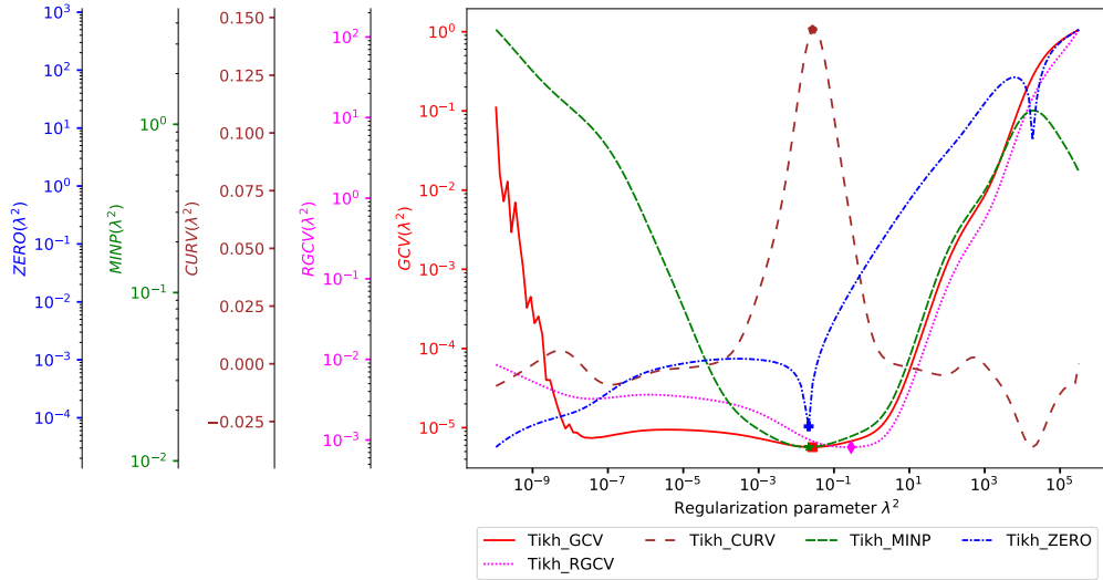
(b) u-iPTF: \lambda^2_{opt} selection criteria for Tikhonov regularization
