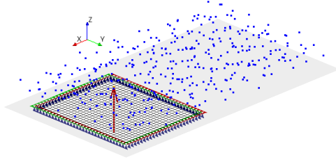
(b) Only plate 1 ( \mathcal{S}_1 ) excited : the radiated sound field is due to a coherent vibration field.
