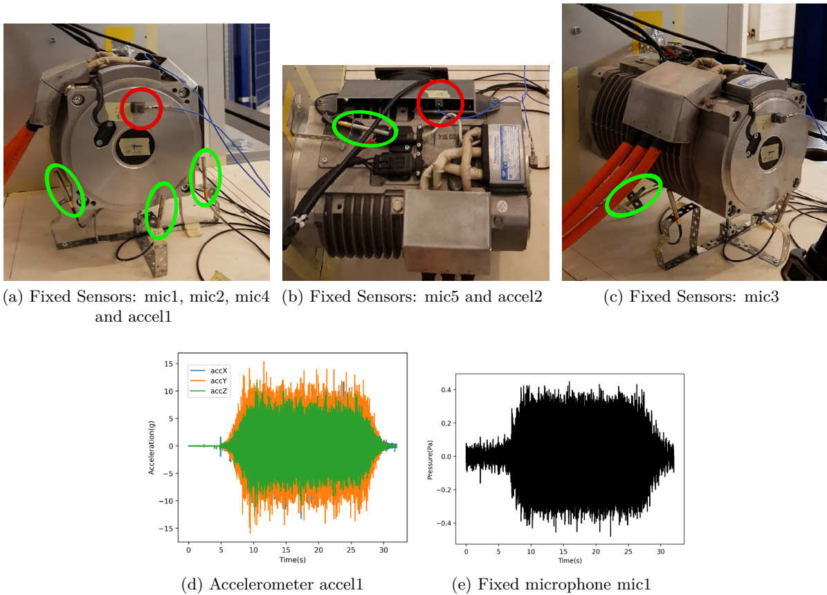
Figure 6.6: (a)-(c) settings of Reference sensors and (d)-(e) time domain signals for accel1 and mic1.
