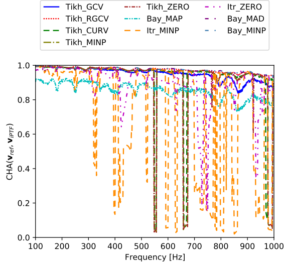
(a) m-iPTF \mathcal{CHA}
