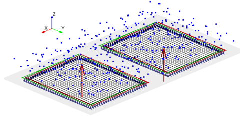
(a) Plate 1 ( \mathcal{S}_1 ) and plate 2 ( \mathcal{S}_1 ) are excited simultaneously with uncorrelated point forces: the radiated sound field is due to two uncorrelated vibration fields.
