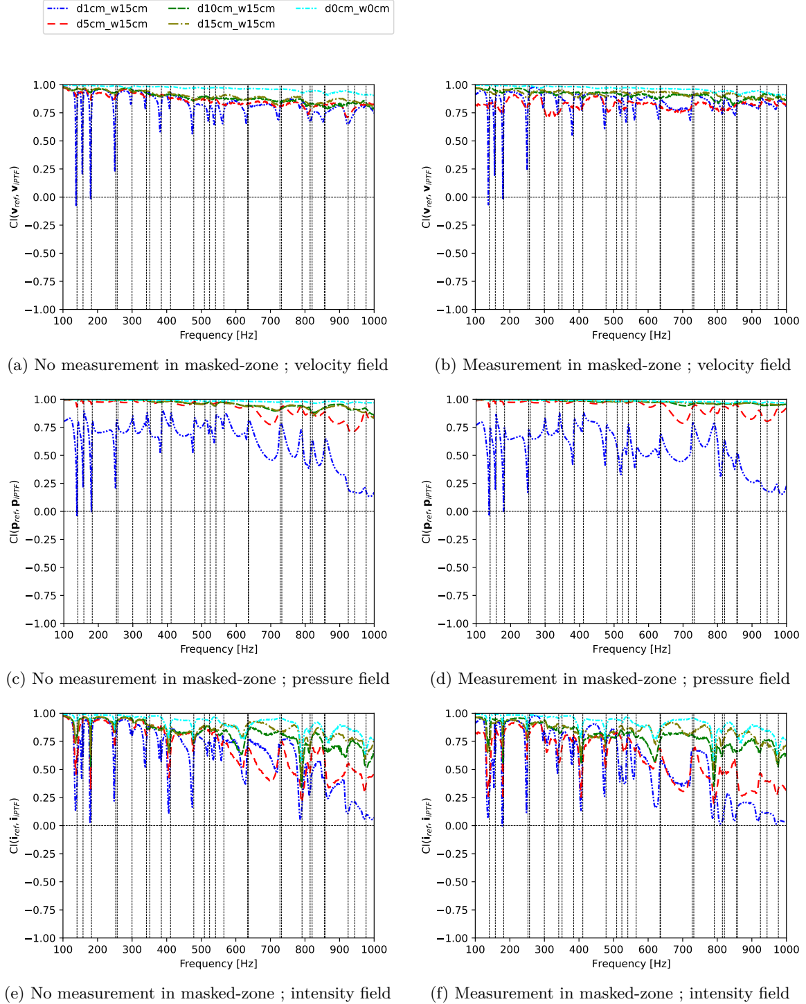
Figure 5.6: Plots of CI correlation metric used in the comparison of the source acoustic indicators identified by iPTF and that computed on the plate (reference) for the full frequency spectrum of the different masking object distance test set-ups. The vertical lines indicate the positions of the plate eigen frequencies.
