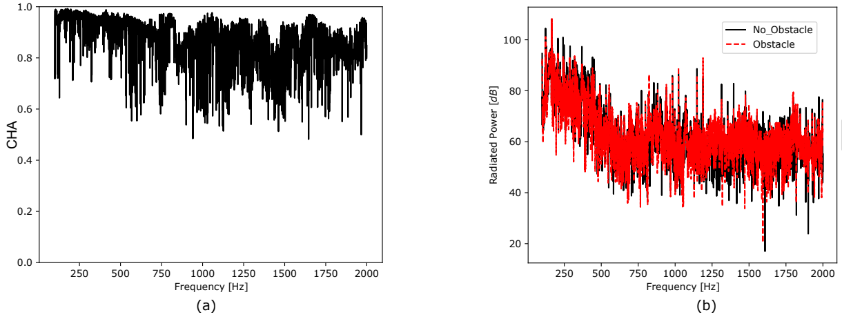
Figure 6.16: Comparison of the characterizations of the SimRod e-motor without and with the masking object. (a) \mathcal{CHA} correlation metric computed by comparing the directivity diagrams obtained from the velocity fields identified from measurements with and without the presence of the masking object and (b) radiated acoustic power spectra computed from fields identified from measurements with and without the presence of the masking object.
