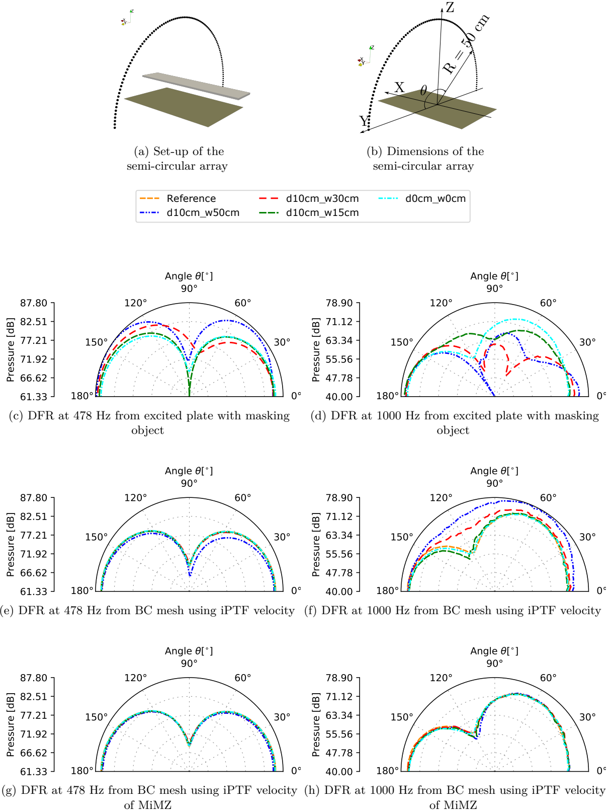
Figure 5.21: Settings and polar pressure radiation pattern of the ZY semi-circular array recorded at a frequency of 478 Hz and 1000 Hz for the different masking object distance test set-ups.
