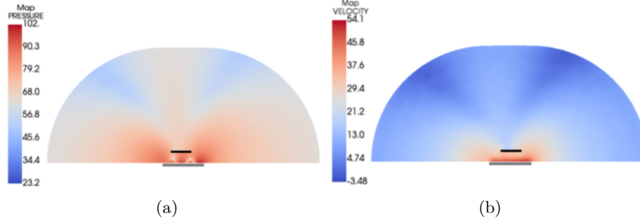
Figure 5.3: A cut- section view of the acoustic radiation from the excited plate in the presence of masking object positioned 10 cm away from the plate at 900 Hz. (a) The radiated pressure field (dB, ref: 2 \times 10^{-5} Pa) and (b) the radiated velocity field (dB, ref: 5 \times 10^{-8} (m/s)).
