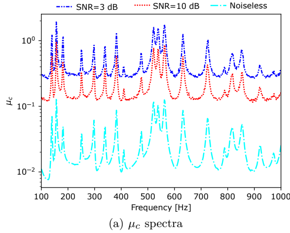
Figure 3.5: Ill-posedness level spectra for m-iPTF problems with different levels of simulated noisified \mathbf{y} for full frequency of study.
