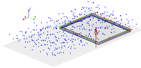
(c) Only plate 2 ( \mathcal{S}_2 ) excited : the radiated sound field is due to a coherent vibration field
