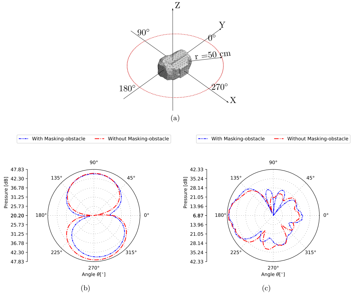
Figure 6.15: Directivity plot for 201 microphones positioned in the XY plane at 50cm from the centroid of the simrod e-motor. (a) settings ; (b) directivity diagram at 545 Hz ; (c) directivity diagram at 1992 Hz.
