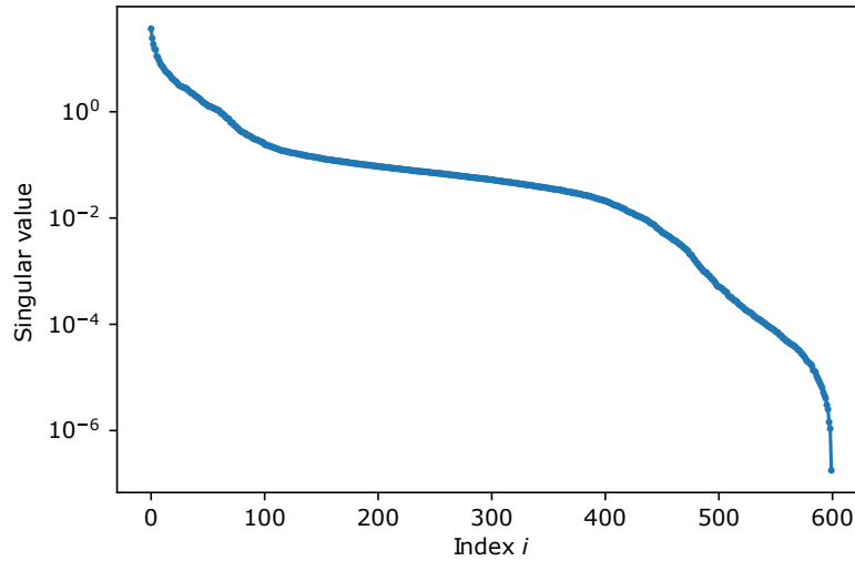
Figure 3.2: Singular value spectrum of the 600 \times 600 impedance transfer matrix \mathbf{Z}_{mj} in Equation (2.30) at 100Hz.
