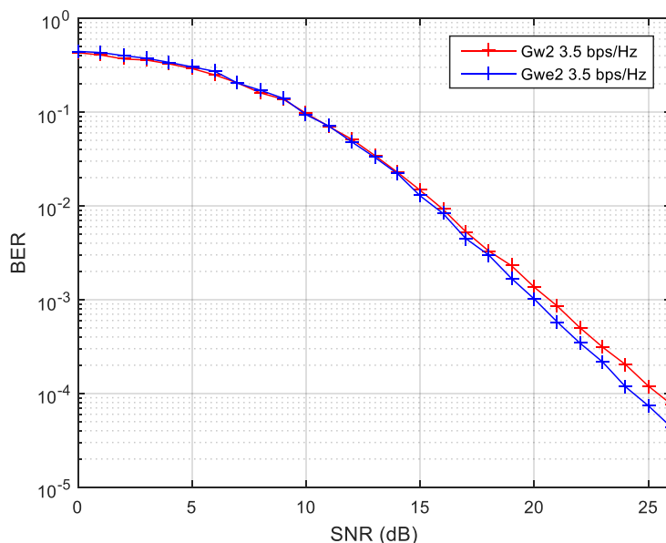
FIGURE 1 – Performance of the selected sets of matrices for \mathcal{G}_{w2} and \mathcal{G}_{we2} (or \mathcal{G}_{wce2} ) for 3.5 bps/Hz
