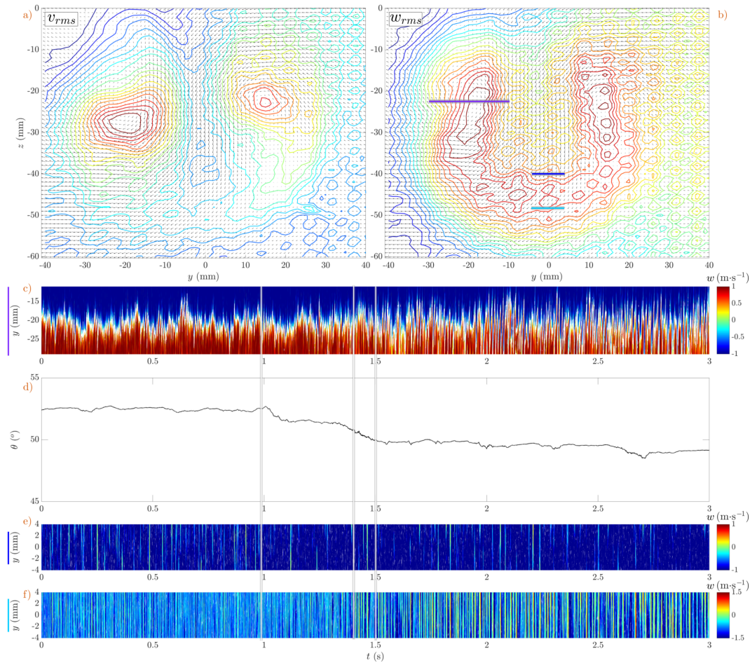
Figure 5.8: Details on the temporal dynamics in the wake for a L→D transition. a-b) Average flow structure and fluctuations over the whole duration of transition (a: v_{rms} , b: w_{rms} ). d) Angular time series. c,e-f) Spatio-temporal evolution of w along a horizontal segment. The corresponding segments for each spatio-temporal diagram are represented with matching colors in panel b.
