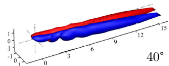
+/- isovorticity [Gao et al. 2018]
