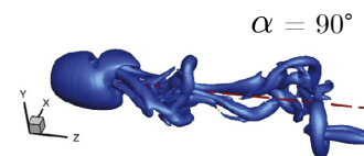
0-isovorticity [Tian et al. 2017]
