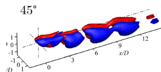
+/- isovorticity [Gao et al. 2018]
