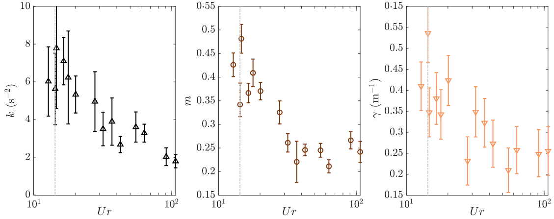
Figure 6.4: Added stiffness k , mass m and damping \gamma obtained for each Ur parameter in the experiments. Dash-dotted line represents 1/St with St \simeq 0.07 .
