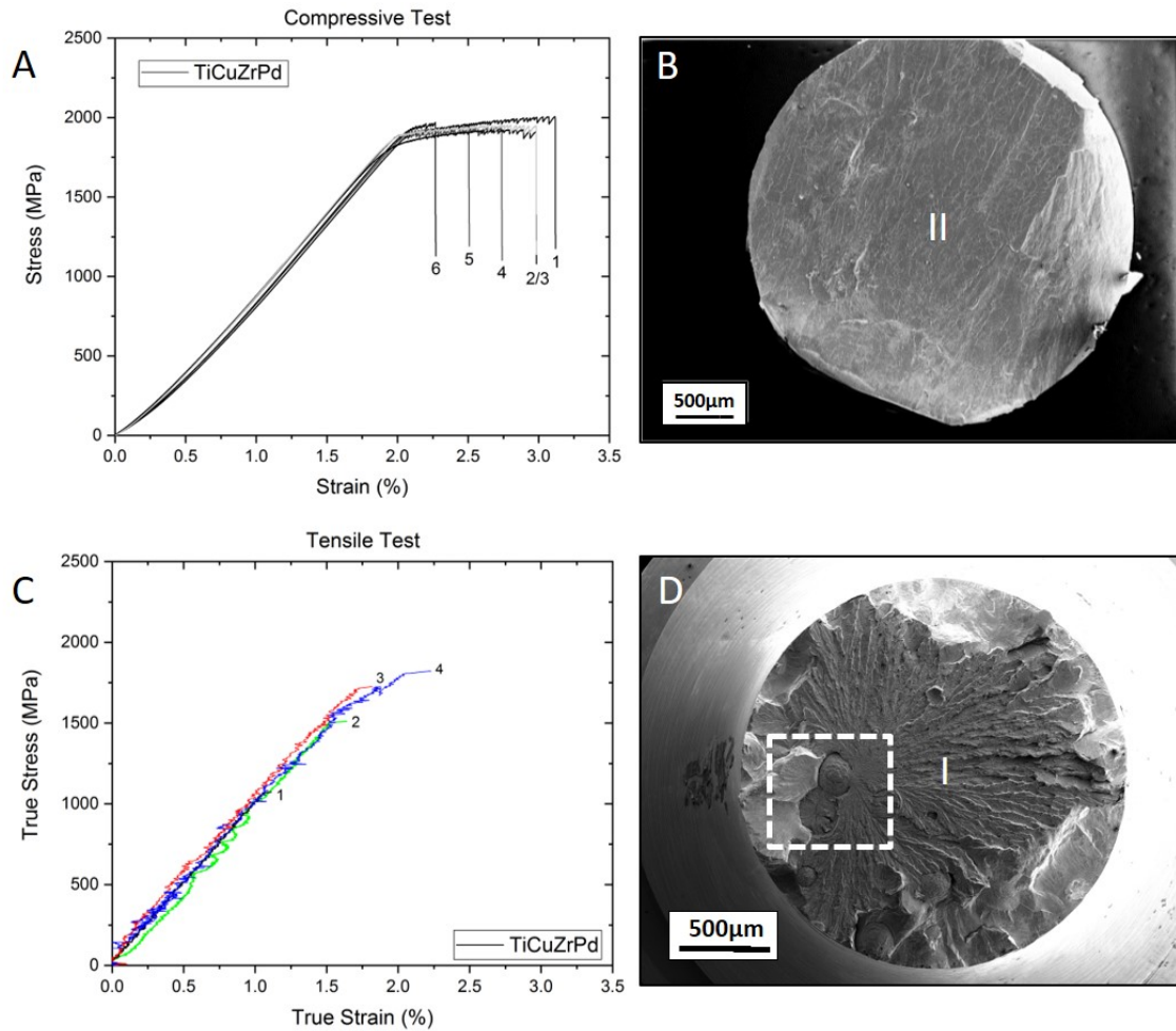
FIGURE 1.8 – (A) compressive stress-strain curves obtained on 6 samples of \text{TiCuZrPd} BMG with (B) SEM picture of a representative fracture surface extract from [LIE 18]. (C) tensile true stress-strain curves obtained on 4 samples of \text{Ti}_{40}\text{Cu}_{36}\text{Zr}_{10}\text{Pd}_{14} with (D) SEM picture of a representative fracture surface which illustrates the presence of casting defects.
