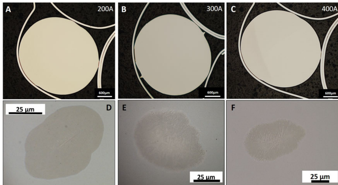
FIGURE 3.2 – Pictures A, B and C were taken using optical microscopy and illustrate the aspect of the microstructure of 3mm casted rods with different electric arc intensities and D,E and F are higher magnification pictures of the spherulite inside the rods. A and D- 200A. B and E- 300A. C and F- 400A.
