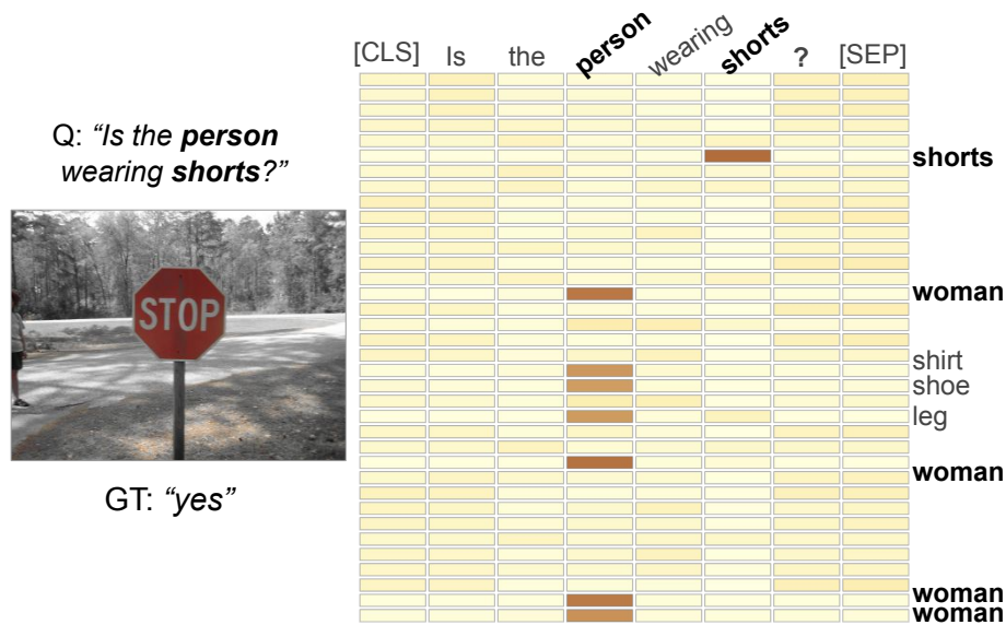
Figure 3.8 – When asked “Is the person wearing shorts?”, the oracle transfer model successfully answers “yes”. It can be observed in its first Language-to-Vision attention maps, that the word “shorts” (column) is strongly associated with the object “shorts” (row). The same phenomenon is also observed for the word “person”, strongly associated with objects labeled as “woman” among others.
