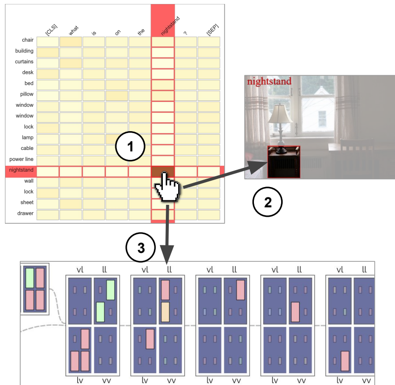
Figure 3.7 – Hovering the mouse over a cell of the attention maps ① filters the corresponding object bounding box in the input image ②. While clicking on this cell filters attention heads in instance-view to display those within which the selected cell is highly activated.
