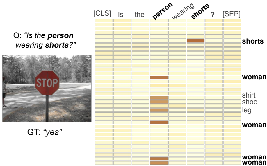
Figure 3.8 – When asked “Is the person wearing shorts?”, the oracle transfer model successfully answers “yes”. It can be observed in its first Language-to-Vision attention maps, that the word “shorts” (column) is strongly associated with the object “shorts” (row). The same phenomenon is also observed for the word “person”, strongly associated with objects labeled as “woman” among others.
