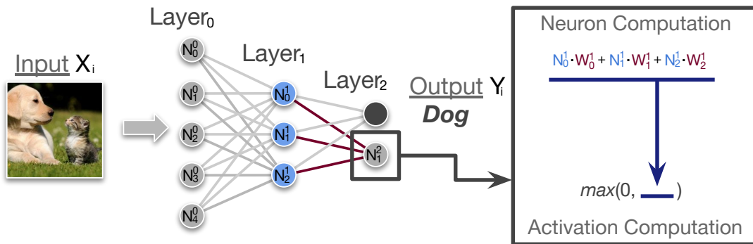
Figure 2.1 – Illustration of the structure of a Deep Neuron Network. With the input image X_i , the neurons of the model, arranged in inter-connected layers, yield the output Y_i "dog". This output is the outcome of a multitude of neuron computations. As depicted on the right of this figure, each neuron ( e.g. here N_1^2 ) relies on the result of neurons from the previous layer. A more formal representation of this computation is depicted in Equation 2.1.
