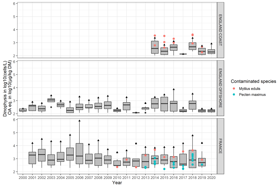
FIGURE 7.2 – Historic of Dinophysis spp. densities ( > 100 \text{ cells.L}^{-1} ) over the years at locations across the Channel and the maximum toxicity values ( > 160 \mu\text{g OA eq.kg}^{-1} in Dry Meat) encountered on two commercial species ( Mytilus edulis and Pecten maximus ).
