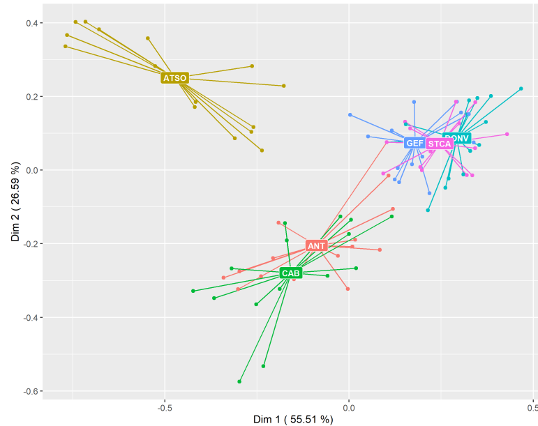
FIGURE 4.3 – Generalized Procrustes Analysis displaying the six stations’ relationship on two axis in an ordination plot. Their closeness relates of their proximity in composition considering the period 2008-2019. Each dot per station corresponds to a functional group’s position.
