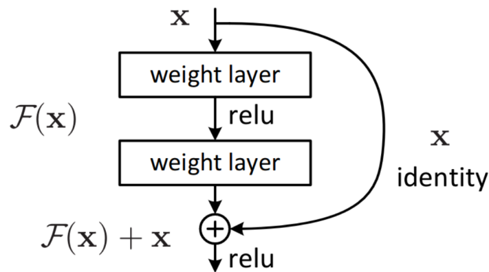
Figure 4.1: Residual learning building block (figure from [HZRS16])
