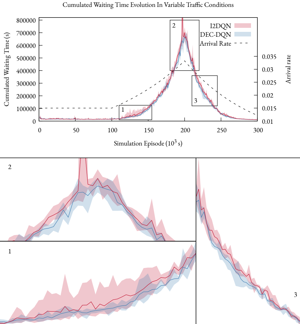
Figure 9.14: Analysis of the I2DQN and DEC-DQN algorithms in variable traffic conditions.
