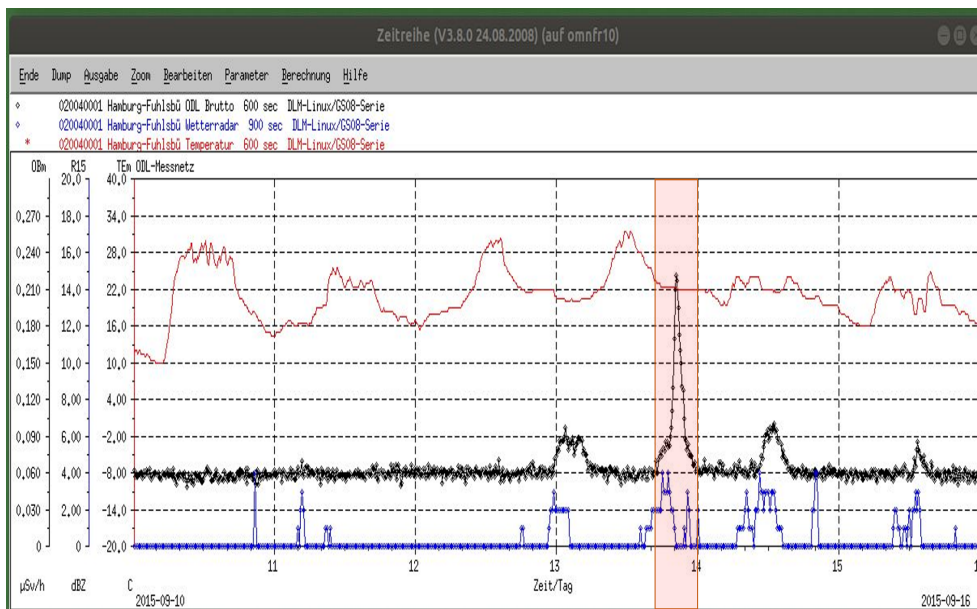
Figure 3.16: Precipitation, temperature, and gamma dose rate data at the time of an incident (highlighted in red)
