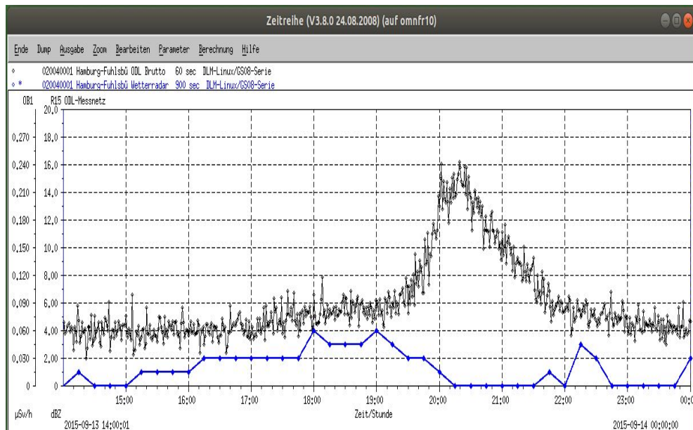
Figure 3.17: Precipitation and gamma dose rate data at the time of an incident (close-up)
