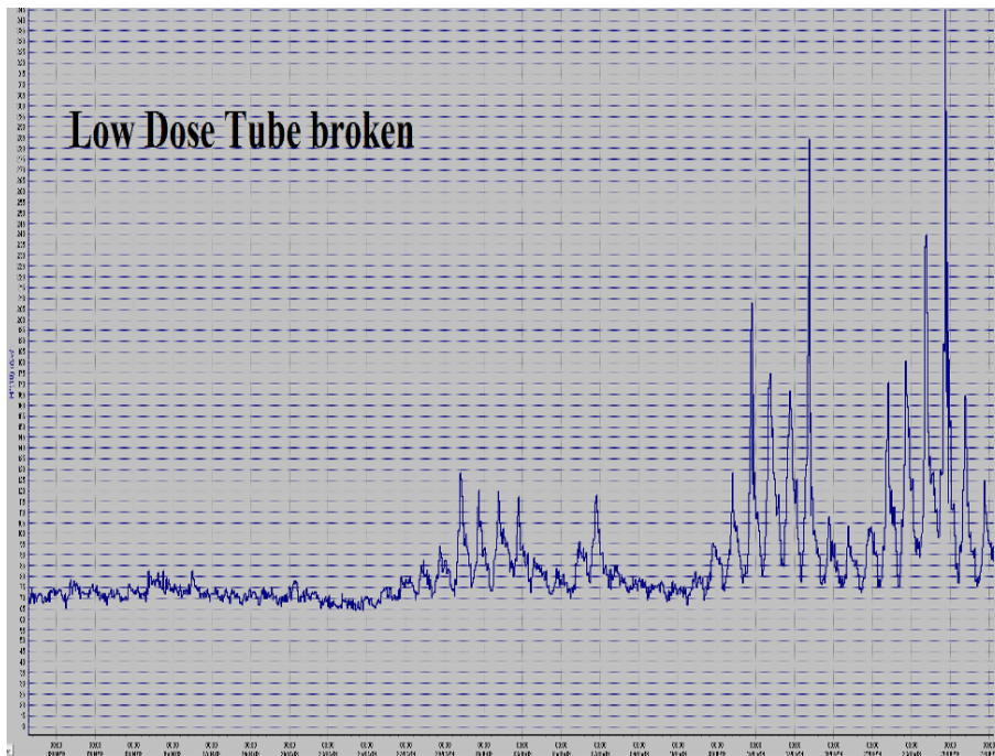
Figure 2.5: Low Dose Tube Broken Effect on Gamma Dose Rate
