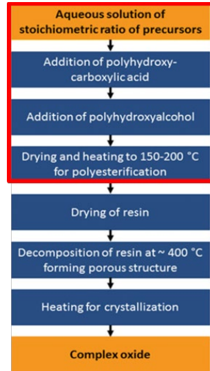
Figure 133: Modified Pechini method steps carried out, highlighted in red rectangle [68]
