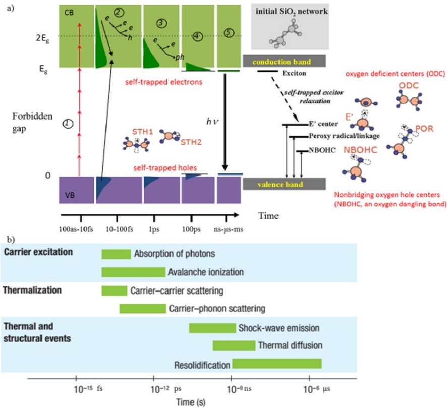
Figure 31: a) Schematic representation of the dynamics of fs laser interactions with dielectrics. The numbers from 1 to 5 correspond to the process as described within the text (after S. Guizard, LSI, CEA, Saclay France and [29]), b) timescale of the physical phenomena associated with the interaction of a fs laser pulse with transparent material [27]
