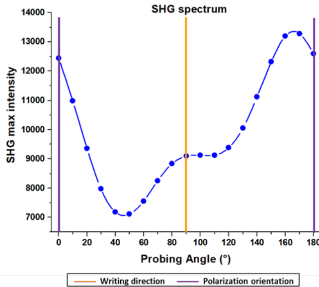
Figure 57: SHG spectrum obtained for LNS13B21 lines written at 1.25 \mu\text{J}/\text{pulse} , at Y_x polarization configuration, at fixed repetition rate equal to 200 \text{ kHz} and scanning speed equal to 1 \mu\text{m}/\text{s} . The reference position of the laser polarizer is 0^\circ , which coincides with the position corresponding to 180^\circ .
