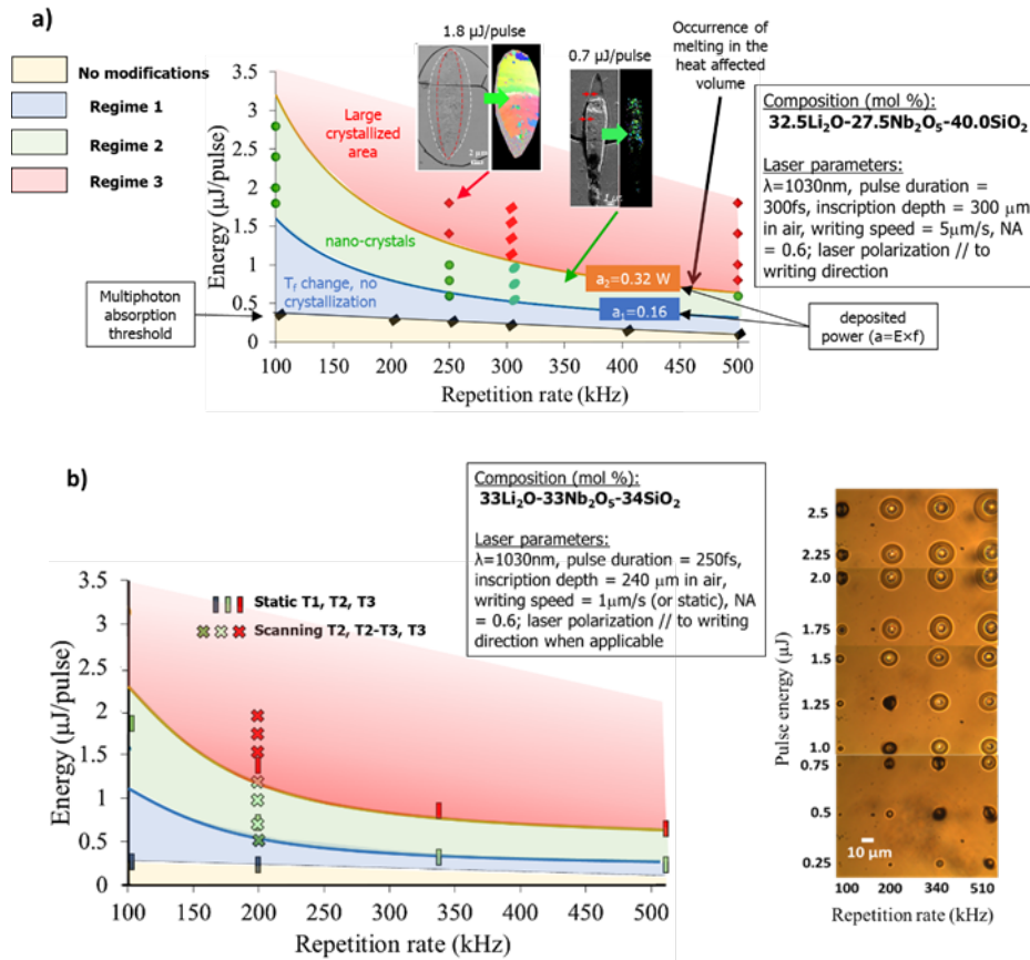
Figure 89: pulse energy-repetition rate landscape highlighting the three regimes of laser induced modifications for a) 32.5Li 2 O-27.5Nb 2 O 5 -40SiO 2 (mol%) [2], [3]; b) for 33Li 2 O-33Nb 2 O 5 -34SiO 2 (LNS34) (mol%). In addition, the trend of dots written in our experiment in static mode revealed the energy thresholds for LNS34 [2].
