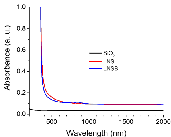
Figure 12: Absorption spectra for LNS (precisely, LNS34), LNSB (precisely, LNS13B21) and SiO 2 (Suprasil) for sake of comparison
