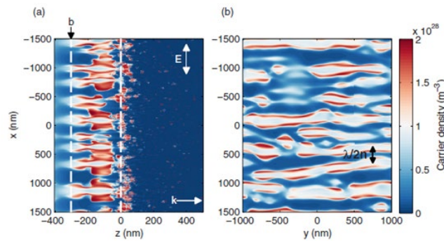
Figure 95: Carrier density generated by a plane wave normally incident on a half-space ( z > 0 ) with many inhomogeneities. The growth structures direction is backwards against the propagation one: from the inhomogeneous/homogeneous border at z = 0 and the grating has a period of \sim \lambda/2n = 275 nm. In a) there is a panel with polarization and laser propagation indicated, while a cut through the grating planes at z = -300 nm is reported in panel b) [46].
