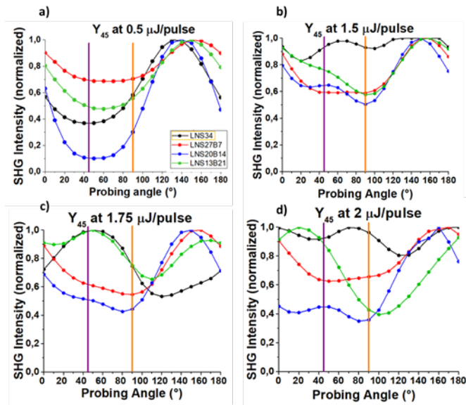
Figure 80: Comparison between four pulse energy values a) 0.5, b) 1.5, c) 1.75 and d) 2 \mu\text{J} at laser polarization configuration Y_{45} . Femtosecond laser conditions used: \lambda = 1030 \text{ nm} , \text{NA} = 0.6 , \text{RR} = 200 \text{ kHz} , focus depth = 240 \mu\text{m} in air, scanning speed = 1 \mu\text{m/s} .
