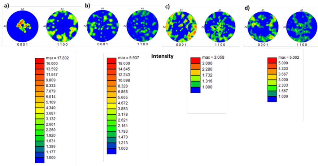
Figure 88: Polar figures referred to LNS34 at 2 \mu\text{m} for a) Y_y , b) Y_x and LNS13B21 at 2 \mu\text{m} for c) Y_y , d) Y_x where A1 is the beam direction, A2 is the laser polarization, A3 is the writing direction
