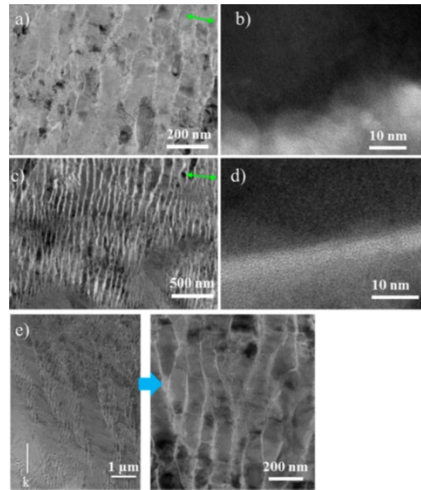
Figure 92: TEM micrographs (bright field mode) of self-assembled nanostructure in LNS glass at various pulse energies (a – b) 0.7, (c – d) 1.3, and (e) 1.8 \mu\text{J}/\text{pulse} . The laser propagation direction is perpendicular to the paper plane for (a – d); nanostructure along the laser propagation direction is illustrated in (e). K is the laser propagation direction. Writing laser polarization direction is indicated by the green double arrows. The micrographs are referred to 33\text{Li}_2\text{O} - 33\text{Nb}_2\text{O}_5 - 34\text{SiO}_2 (mol%), at 1030 nm, 300 fs, 300 kHz, 5 \mu\text{m}/\text{s} , and focus depth 350 \mu\text{m} [3].
