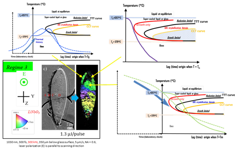
Figure 105: Interpretation of the presence of non-crystallized area in the section of laser traces [3]
