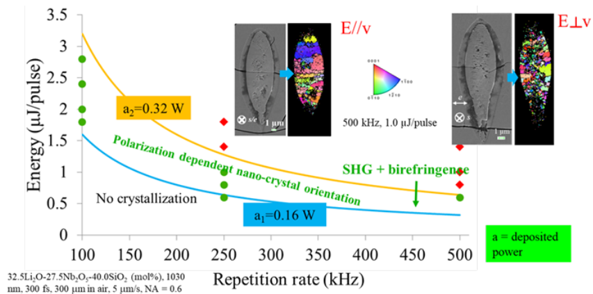
Figure 68: LNS pulse energy-repetition rate landscape [12]
