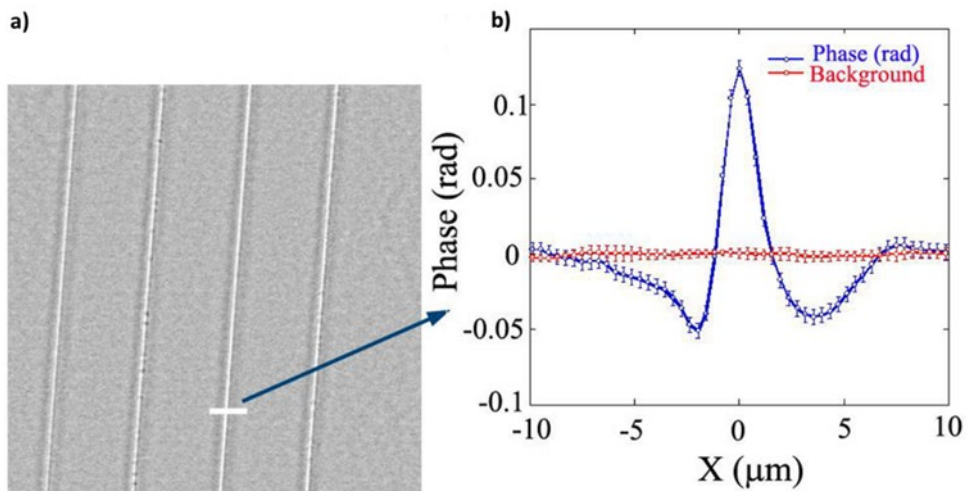
Figure A143: Quantitative phase measurement of the written lines with a line spacing of 50 \mu\text{m} in pure silica: a) phase image and b) profile (line's cross section)
