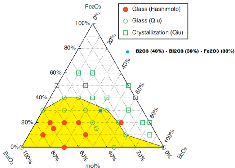
Figure 125: Glass-forming region for \text{Bi}_2\text{O}_3 - \text{B}_2\text{O}_3 - \text{Fe}_2\text{O}_3 system enclosed in yellow [81]: the final and successful composition is reported in light blue point
