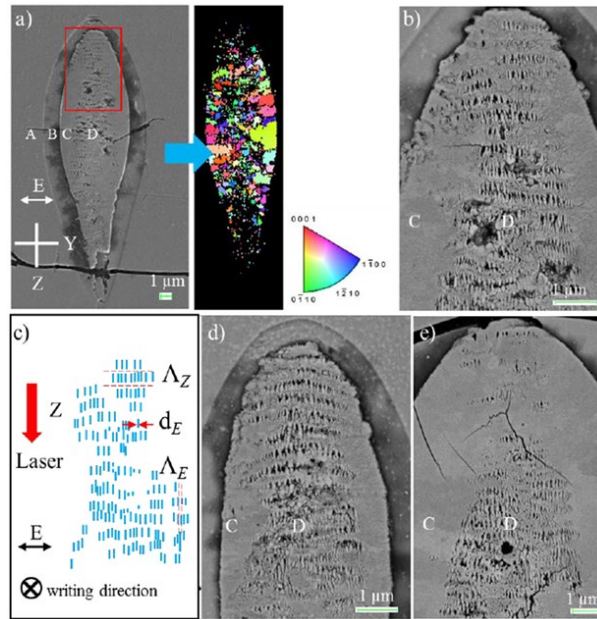
Figure 91: Morphology of the fs laser track with laser polarization, along Y direction, is perpendicular to X direction of scanning: a) SEM micrograph on left side and the corresponding IPF coding along laser polarization direction on the right side for 1 \mu\text{J}/\text{pulse} ; b) this is a magnification of Figure 5.22a enclosed in the red rectangle; c) scheme of laser-induced structures, with forces and main parameters indicated: d_E is the nanostructures thickness, \Lambda_E is the distance between the dashes, \Lambda_Z is the distance between the nanostructure lines; scanning direction is along Z, also writing direction is indicated; morphology of the laser track varying the pulse energy: d) 0.8 and e) 1.4 \mu\text{J}/\text{pulse} . Other fundamental parameters are: 32.5Li 2 O – 27.5Nb 2 O 5 – 40SiO 2 (mol%), 1030 nm, 500 kHz, 300 fs, 5 \mu\text{m}/\text{s} , NA = 0.6, focal depth 300 \mu\text{m} in air [4].
