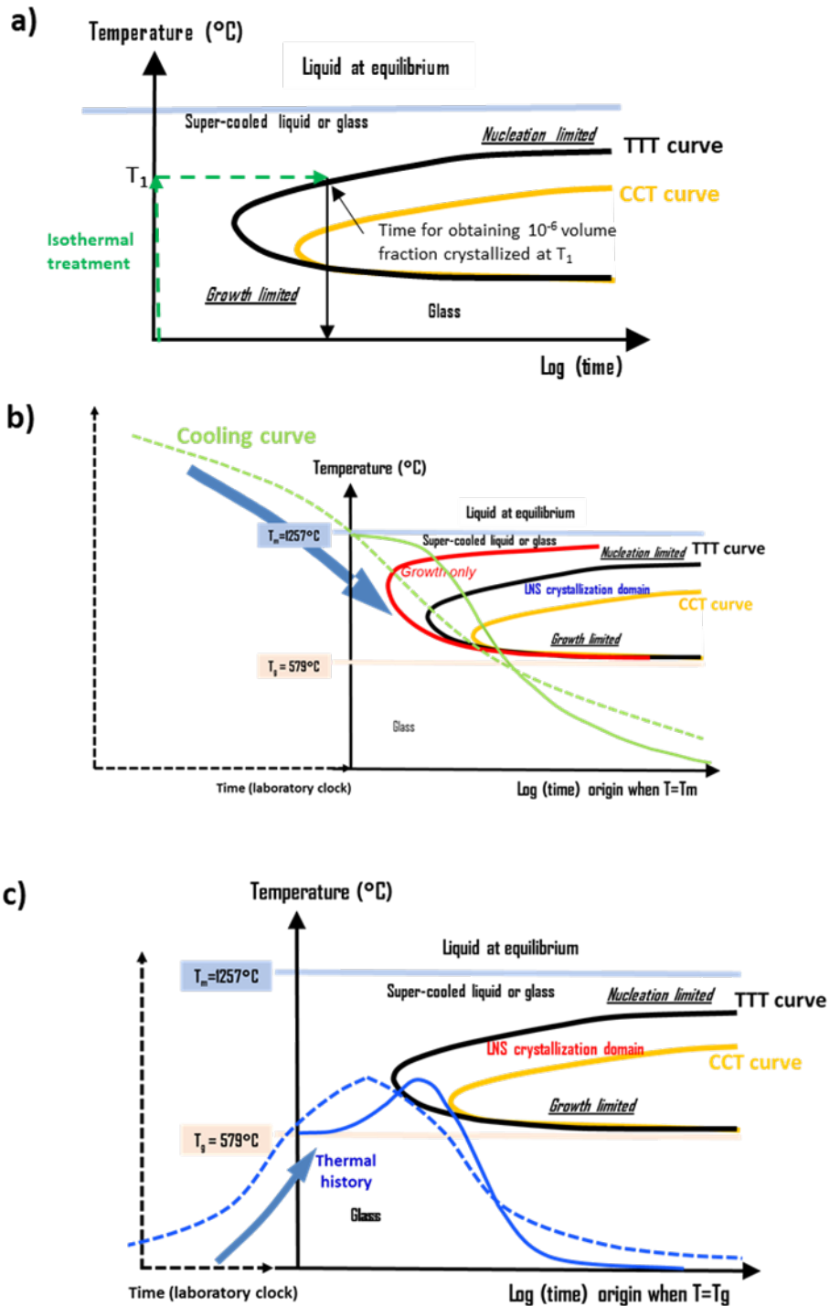
Figure 100: a) only the TTT and CCT curves; these curves with laser thermal treatment curve b) for places experiencing maximum average T larger than T_m and c) for places at maximum temperature smaller than T_m [3]
