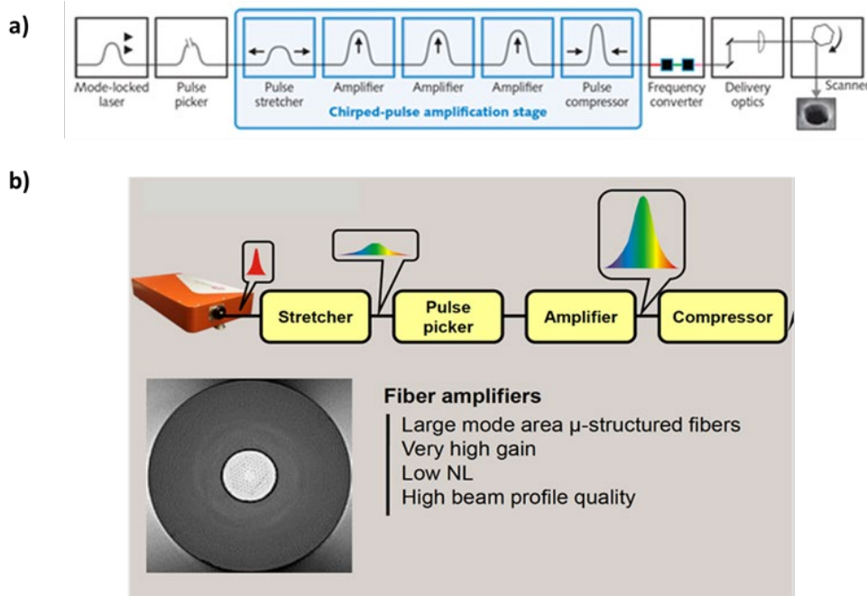
Figure 25: a) CPA Scheme [14]; b) our CPA configuration in which the chirp is illustrated with colours and the signal is treated by a fiber amplifier.
