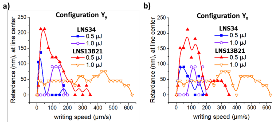
Figure 55: Retardance in nm measured at 550 nm at the center of the irradiated lines as a function of scanning speed for LNS34 and LNS13B21, at two pulse energies (0.5 and 1 \mu\text{J}/\text{pulse} ), repetition rate fixed at 200 kHz and for a) Y_y and b) Y_x laser polarization configurations [18].
