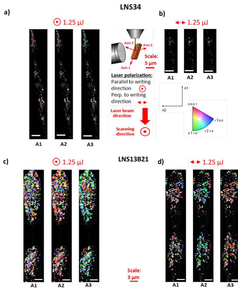
Figure 85: Inverse Pole Figure (obtained from EBDS analysis) for LNS34 at a) Y_y and b) Y_x and for LNS13B21 sample at c) Y_y and d) Y_x , coding the crystal orientation
