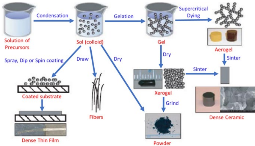
Figure 112: Scheme of sol-gel steps highlighting the variability of different final products that can be achieved (adapted from [1])
