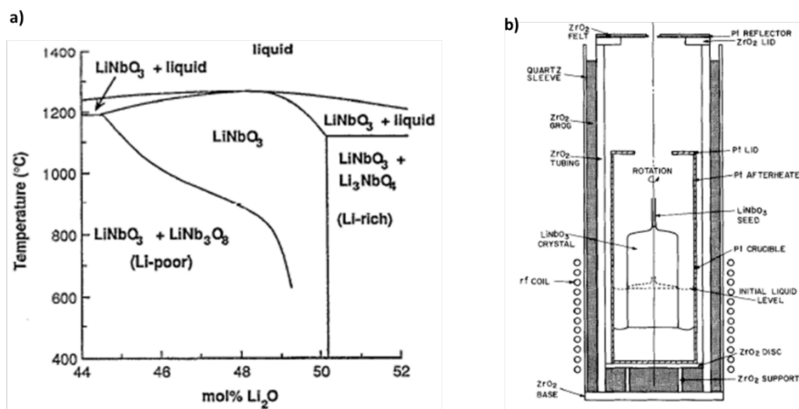
Figure 15: a) Phase-equilibrium diagram for \text{LiNbO}_3 [36] and b) scheme of the furnace for Czochralski growth at \text{LiNbO}_3 [37]
