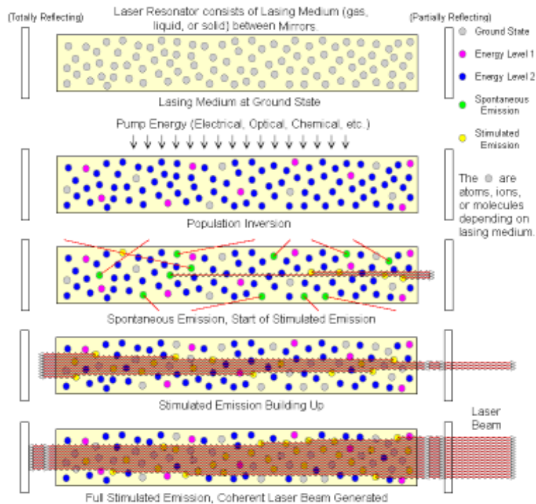
Figure 23: Schematic diagram of laser basic working principle ( https://sites.google.com/site/puenggphysics/home/unit-i/basic-of-laser-action )
