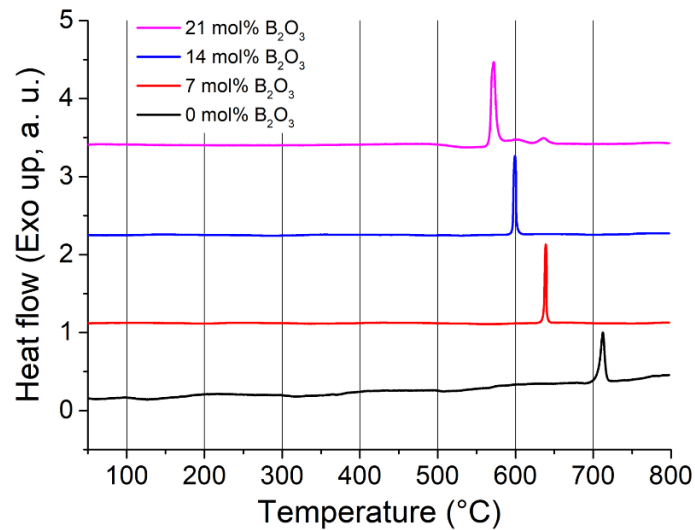
Figure 10: Differential scanning calorimetry (DSC) scans for four glasses composition with an increasing amount of \text{B}_2\text{O}_3 in the batch compositions in mol%
