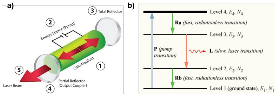
Figure 21: a) Principal laser components ( https://www.ulsinc.com/learn ); b) Four-level laser system ( https://it.wikipedia.org/wiki/population_inversion )
