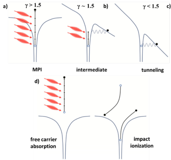
Figure 29: Schematic diagram of the photoionization of an electron in an atomic potential for different values of the Keldysh parameter ( \gamma ). In a solid, the electron is promoted from the valence band to the conduction band rather than ionized: a) multiphoton ionization, c) tunneling ionization, b) the above processes combined, and d) avalanche ionization: free carrier absorption followed by impact ionization [24].
