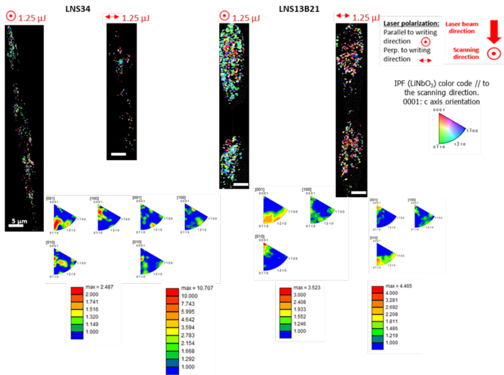
Figure 84: Inverse Pole Figure (IPF) obtained through electron backscatter diffraction (EBSD): the color in the black background represents the crystalline part for LNS34 and LNS13B21 according Y_x and Y_y at 1.25 \mu\text{J}/\text{pulse} . Other laser parameters are \lambda = 1030 \text{ nm} ; f = 200 \text{ kHz} ; \text{NA} = 0.6 ; pulse duration = 250\text{fs} ; focal depth = 240 \mu\text{m} (in air); scanning speed = 1 \mu\text{m}/\text{s} .
