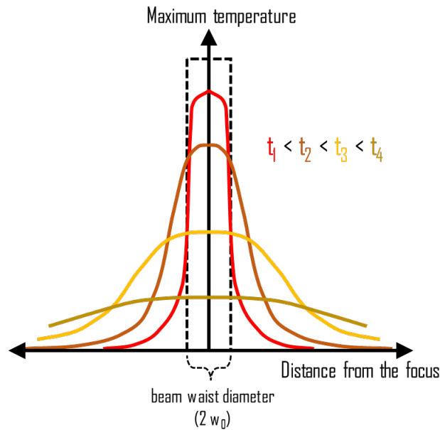
Figure 14: Temperature spatial distribution evolution T(r,t) after pulse deposition inside the glass, as time increases from t_1 to t_4 . At decreasing of maximum temperature with time, the width of the distribution increases [31].
