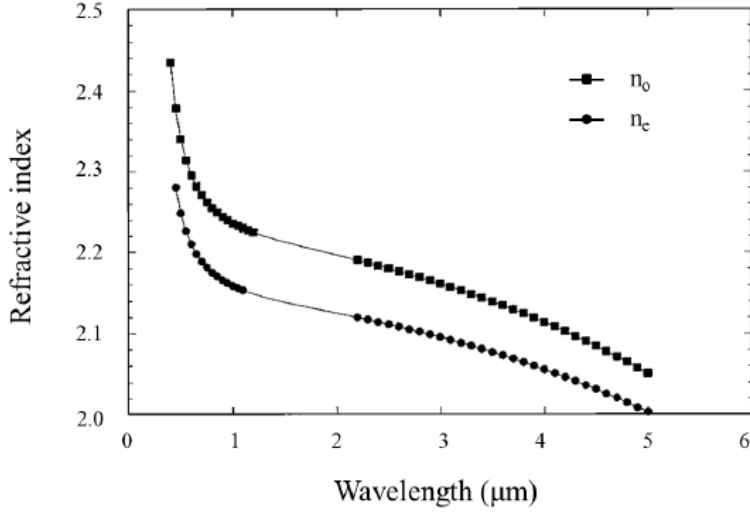
Figure 17: Trend of refractive indexes versus wavelength of congruently growth of \text{LiNbO}_3 [43]
