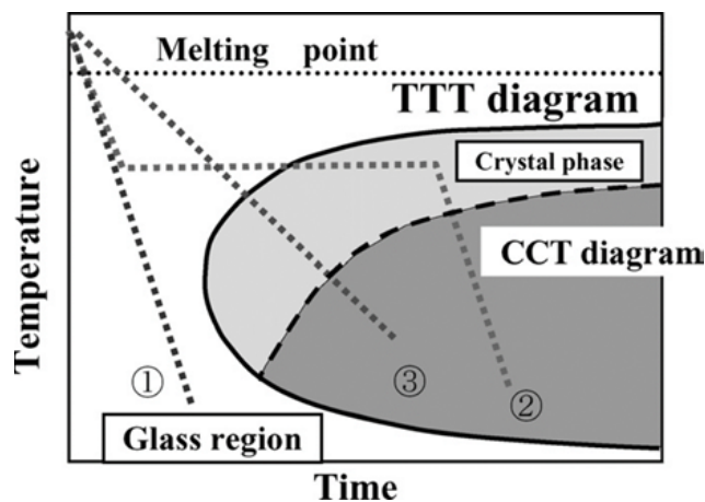
Figure 97: TTT and CCT diagrams [57]
