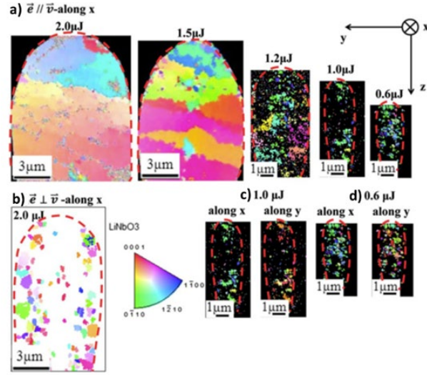
Figure 77: EBSD characterization of 33\text{Li}_2\text{O}-33\text{Nb}_2\text{O}_5-34\text{SiO}_2 : a) EBSD scan images of lines cross-sections irradiated at 2.0-0.6 \mu\text{J} with polarization parallel to the laser beam direction that is coding the crystal orientation along x ; b) EBSD images of lines cross-sections irradiated at 2.0 \mu\text{J} with polarization perpendicular to laser beam direction coding crystal orientation along x ; EBSD scan image coding the crystal orientation along the x -axis and along the y -axis at c) 1.0 \mu\text{J} and d) 0.6 \mu\text{J} , respectively. The polarization for writing is parallel to the laser motion direction. Other laser parameters: repetition rate = 300 \text{ kHz} , scanning speed = 5 \mu\text{m/s} , pulse duration = 300 \text{ fs} , wavelength = 1030 \text{ nm} , and \text{NA} = 0.6 [15].
