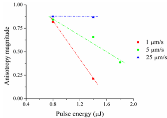
Figure 76: Variation of anisotropy magnitude-pulse energy trend as function of scanning speed. Other parameters: writing direction is along 45^\circ direction, laser polarization is parallel to Y [7].
