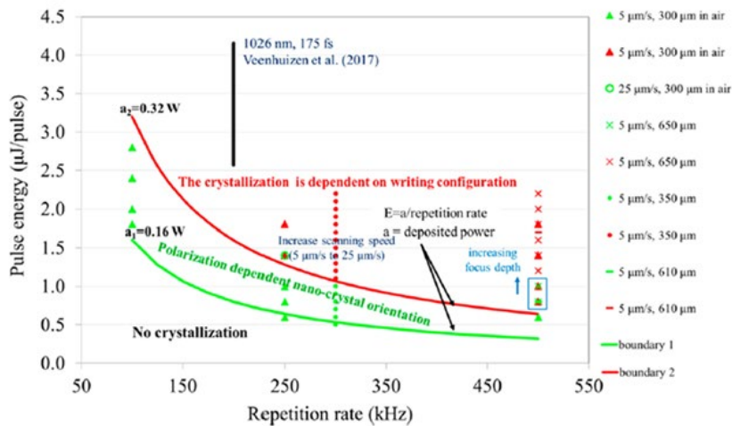
Figure 72: Pulse energy – repetition rate landscape in which domains of fs laser-induced crystallization in LNS glasses at varying scanning speed and focus depth
