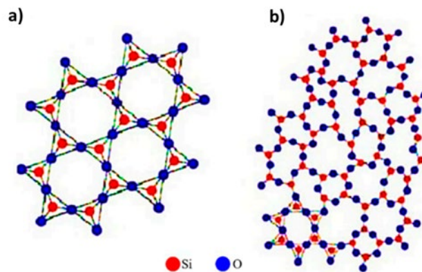
Figure 3: Atomic structure of SiO 2 a) crystal (Quartz) and b) glass (so-called silica) [18]
