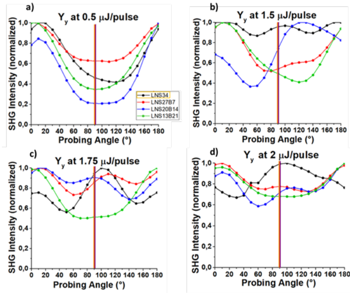
Figure 81: Comparison between four pulse energy values a) 0.5, b) 1.5, c) 1.75 and d) 2 \mu\text{J} at laser polarization configuration Y_y . Femtosecond laser conditions used: \lambda = 1030 \text{ nm} , \text{NA} = 0.6 , \text{RR} = 200 \text{ kHz} , focus depth = 240 \mu\text{m} in air, scanning speed = 1 \mu\text{m/s} .
