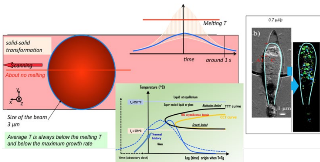
Figure 101: Time evolution of the temperature relative to a fixed point according to the distance from the focus center in scanning mode and SEM micrograph and EBSD map of the cross section of the laser track obtained at intermediate pulse energy in regime 2 for LNS glass [3]
