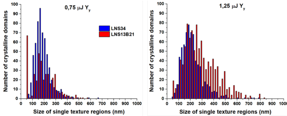
Figure 65: Size distribution of single texture regions for LS34 and LNS13B21 for Y_y configuration and two different pulse energies (0.75 and 1.25 \mu\text{J}/\text{pulse} ). Irradiations conditions: \lambda = 1030 \text{ nm} , \text{NA} = 0.6 , f = 200 \text{ kHz} , focus depth = 240 \mu\text{m} in air, writing speed = 1 \mu\text{m}/\text{s} [6].
