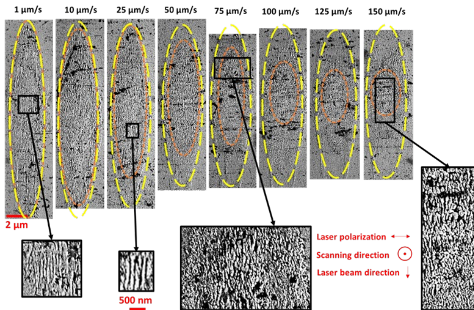
Figure 63: Scanning electron micrographs of the laser track cross-section induced by fs-laser on LNS13B21 glass sample and for different scanning speeds. In yellow there is the area where crystallization within the laser track, associated with crystallization, is detected; in orange, the area where lamella-like nanogratings are observed. Fixed parameters are: \lambda = 1330 nm; f = 200 kHz; NA = 0.6 ; pulse duration = 250 fs; focal depth = 240 \mu\text{m} (in air) [18].
