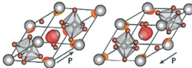
Figure 120: Mechanism promoting the coexistence of magnetic and electric long-range order: the case of lone - pair in \text{BiFeO}_3 . The two \text{Bi}^{3+} electrons shift away from the \text{Bi}^{3+} ion generating the ferroelectricity and towards \text{FeO}_6 octahedra, giving rise to a spontaneous polarization P along the [111] direction. Lone - pair is represented by the red isosurface of electron localization function of \text{BiFeO}_3 [45]
