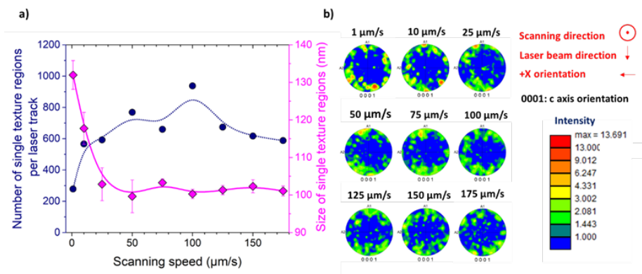
Figure 67: a) number of single texture regions and their averaged diameter, assuming a spherical shape, as a function of scanning speeds; b) pole figures of the
