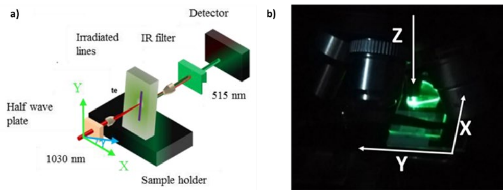
Figure 56: a) Second Harmonic Generation (SHG) setup used for all the experiments of this Ph.D. work [19]; b) SHG detected under static irradiation at the end of the incubation time of a few seconds [6]
