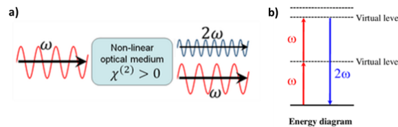
Figure A141: Scheme of SHG phenomenon from two different points of view: a) non-linear optical medium diagram and b) virtual energy diagram
