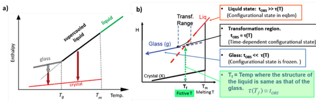
Figure 4: a) Scheme of a glass-forming substance, specifically enthalpy versus temperature plot showing four distinct states: liquid (L), supercooled liquid (SCL), glass (G) and crystal (C). T_m = melting temperature, T_g = glass transition temperature [13]; b) Change of enthalpy with the temperature for the different allotropic phase (cooling at a fixed rate, q ( t_{OBS} \sim 1/q )).
