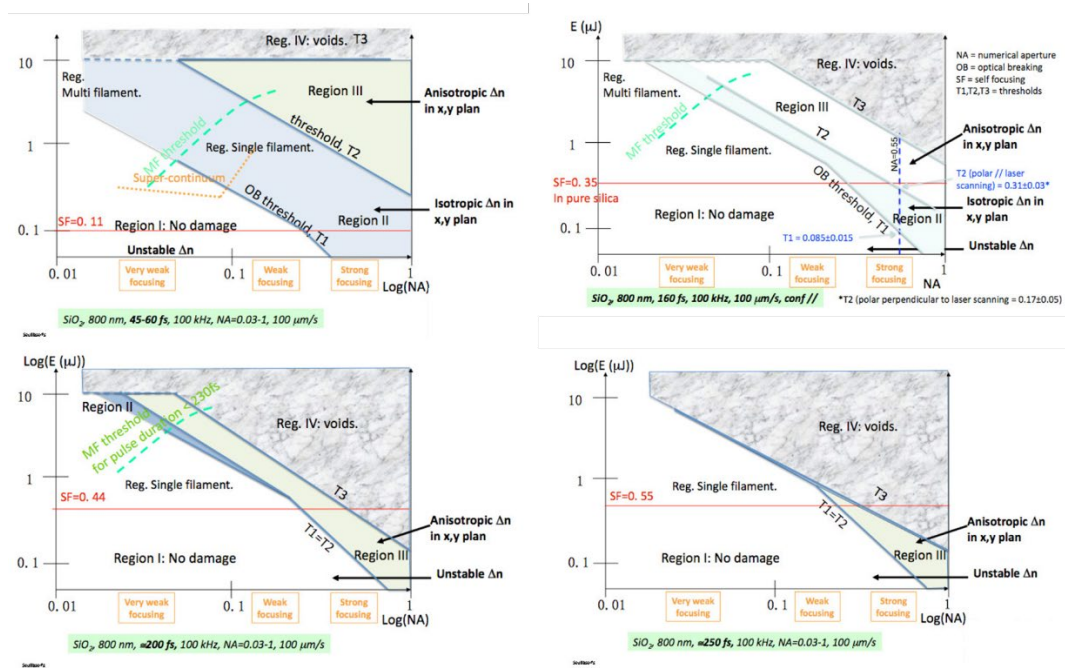
Figure 35: Pulse energy versus numerical aperture (NA) and pulse duration: diagram for a) small pulse duration (45 – 60 fs), b) 160 fs, c) 200 fs, and d) 250 fs (region II disappears) with SiO 2 [41]
