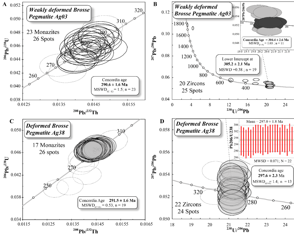
Figure 9 : Monazite U-Th-Pb concordia diagrams (A and C) and zircon Tera Wasserburg diagrams (B and D) of the Brosse ravine pegmatites Ag03 and Ag38. Error ellipses and uncertainties in ages are \pm 2\sigma . In the (A), (C) and (D) diagrams, the dotted ellipses are taken into account for the concordia age calculation while in diagram (B) these are the white ellipses.
