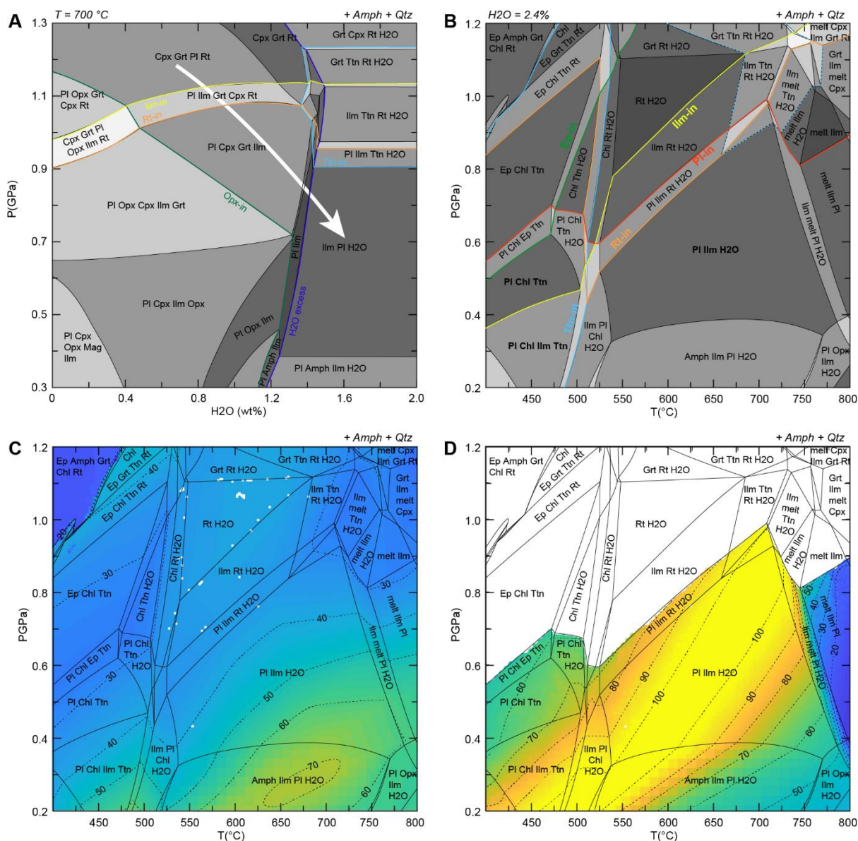
Figure 10: Phases diagrams obtained from sample AR481: (A) P – \text{MH}_2\text{O} diagram highlighting the increase of water content during the decompression of the eclogite constrained by the appearance of titanite at high-pressure and high-water content conditions and orthopyroxene at low-pressure and low-water content conditions. (B) Mineral assemblage diagram obtained from sample AR481 bulk composition with high-water content ( \text{H}_2\text{O} = 2.4 wt%). (C) Modelling of the Q_{\text{cmp}} factor of large euhedral amphibole ( \text{Amph}_3 ) based on CaO, FeO, MgO, \text{Na}_2\text{O} , \text{TiO}_2 , \text{SiO}_2 and \text{Al}_2\text{O}_3 contents (Table S2). (D) Modelling of the Q_{\text{cmp}} factor of the plagioclase ( \text{Pl}_3 ) based on CaO, \text{Na}_2\text{O} , \text{SiO}_2 and \text{Al}_2\text{O}_3 contents (Table S2). Amph: amphibole; Chl: chlorite; Cpx: clinopyroxene; Ep: epidote; Grt: garnet; Ilm: ilmenite; Opx: orthopyroxene; Pl: plagioclase; Qtz: quartz; Rt: rutile; Ttn: titanite.
