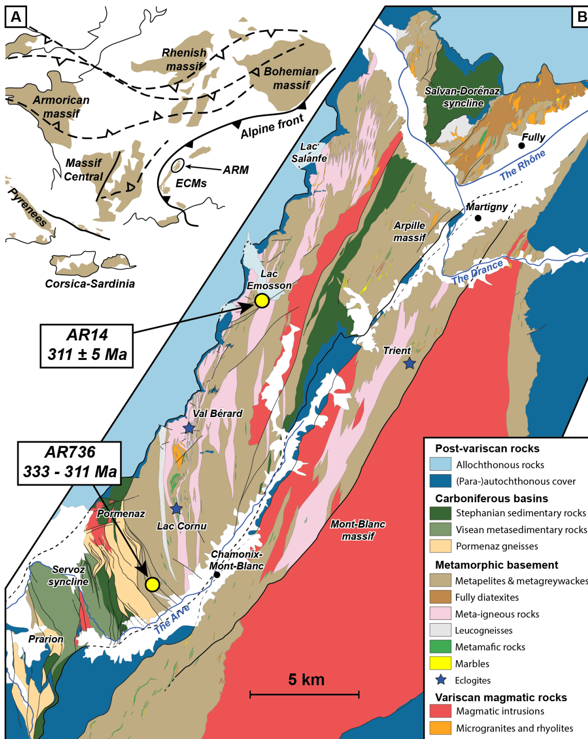
Figure 1 : (A) Paleogeographic reconstitution of the European Variscan Belt at the end of the Variscan orogeny modified from Franke et al. (2017). (B) Geological map of the Aiguilles-Rouges and the Mont-Blanc Massifs with localization of the two samples used in this study and the monazite ages obtained.
