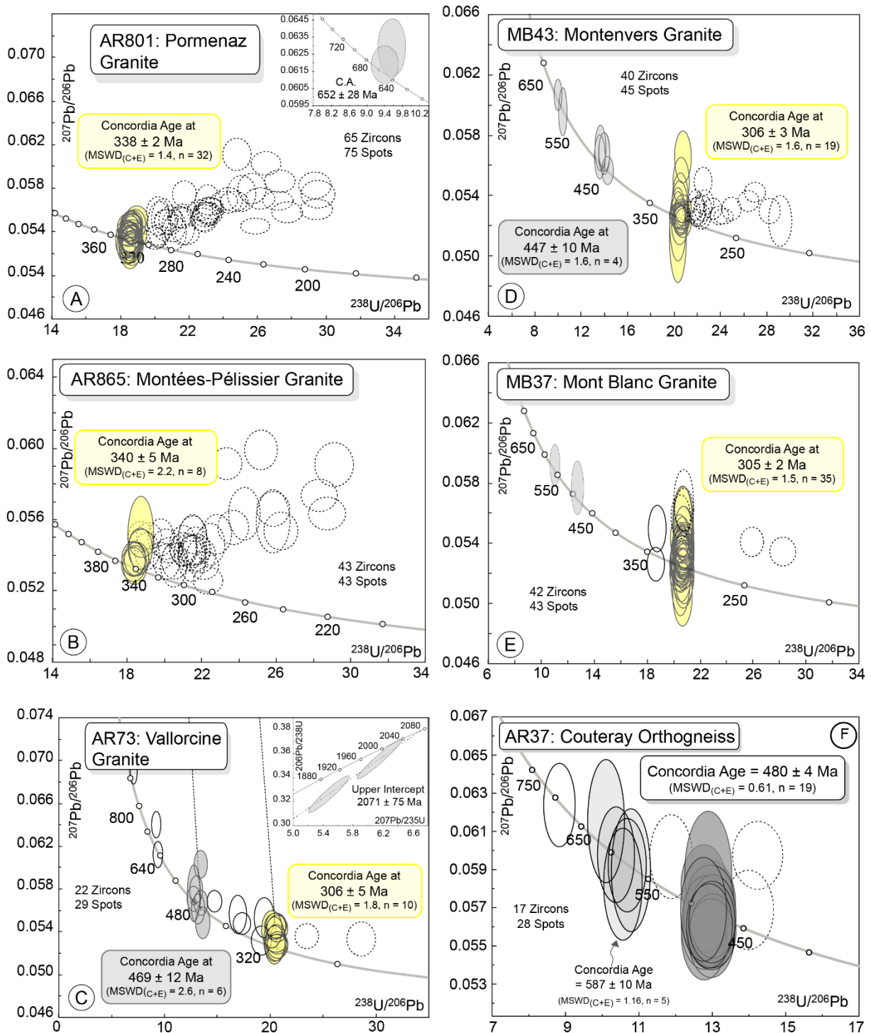
Figure 11 : Zircon U-Pb Tera Wasserburg diagrams obtained by LA-ICPMS on (A) the Pormenez granite (AR801), (B) the Montées Pélissier granite (AR865), (C) the Vallorcine granite (AR73), (D) the Monteners granite (MB43), (E) the Mont Blanc granite (MB37), (F) the Couteray orthogneiss. Error ellipses and uncertainties in ages are \pm 2\sigma level. The discordance of dotted ellipses is due to radiogenic Pb losses and common Pb contaminations. Dotted and white ellipses are not taken into account for the age calculation (see text for detail).
