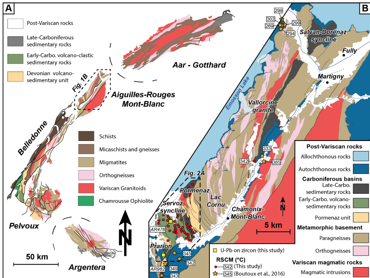
Figure 1 : (A) Geological map of the Variscan basement of the External Crystalline Massifs in the French and Swiss Alps. (B) Geological map of the Aiguilles-Rouges massif with locations of LA-ICPMS U-Pb dated samples AR476 and AR982 on zircon, and RSCM samples analysed in this study and those of Boutoux et al. (2016). Location of figure 2a is shown.
