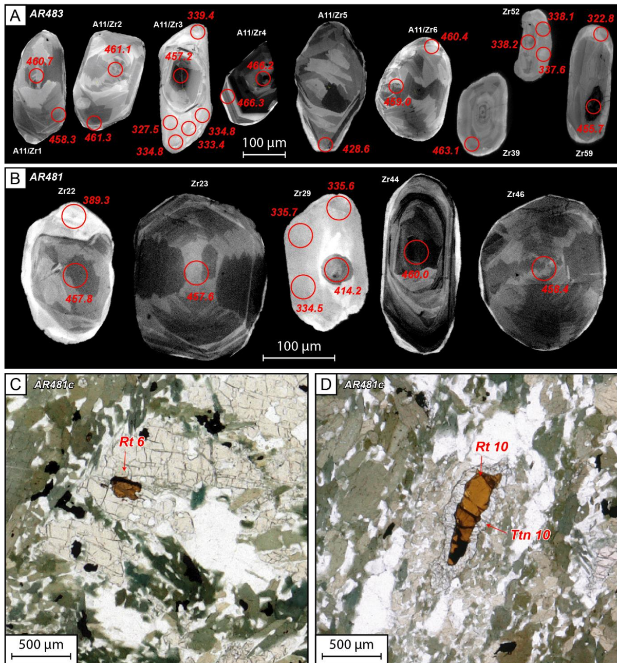
Figure 12: Cathodoluminescence photos of zircons from (A) Sample AR483 and (B) Sample AR481. Rutile from thin section AR481C (C) in garnet inclusion and (D) in the matrix with titanite-coronas also dated.
