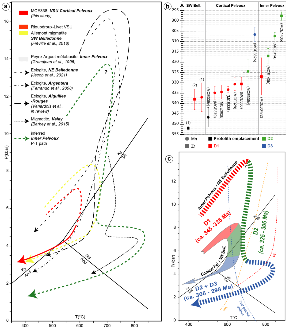
Figure 12: Geochronological and tectono-metamorphic interpretations for the Belledonne and Pelvoux massifs from Fréville et al. (in review). (a) P-T paths of the Cortical Pelvoux / SW Belledonne and of the Inner Pelvoux / NE Belledonne inferred from petrological and thermobarometric results from this study, Fréville et al. (2018), Grandjean et al. (1996), Ferrando et al. (2008), Jacob et al. (2021), Vanardois et al. (in review) and Barbey et al. (2015). (b) Geochronological results constraining the ages of D1, D2 and D3 from this study, (Fréville et al., 2018; Fréville, 2016). (c) Inferred tectono-metamorphic evolutions of the external and internal domains of the Belledonne and Pelvoux areas.
