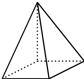
Figure 7: The pyramid model P_4 .
