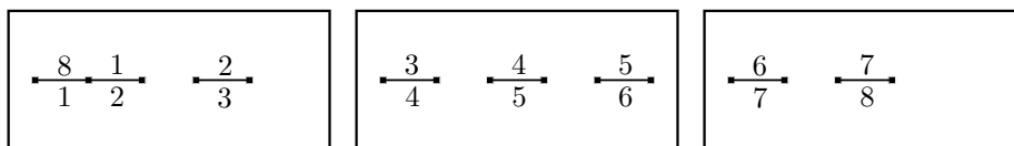
Figure 8: Construction for (n, k, l, g) = (6, 1, 2, 5) .
