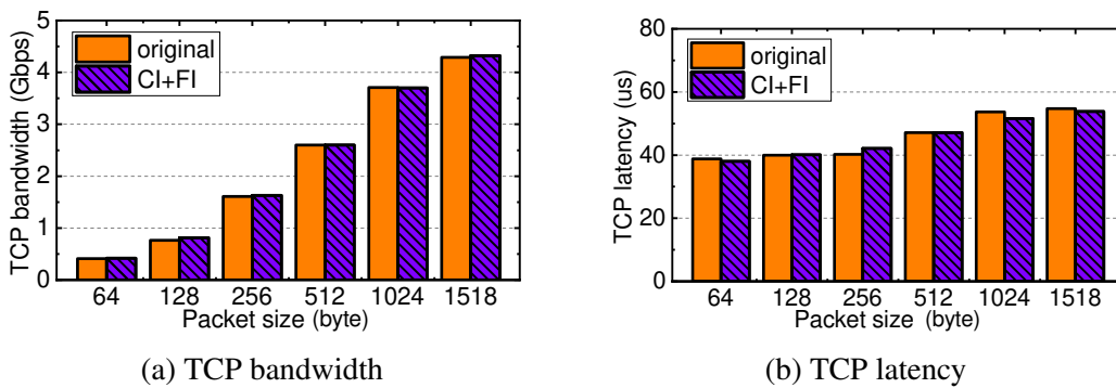
Figure 4.8 The TCP performance under D-TSE strategy
