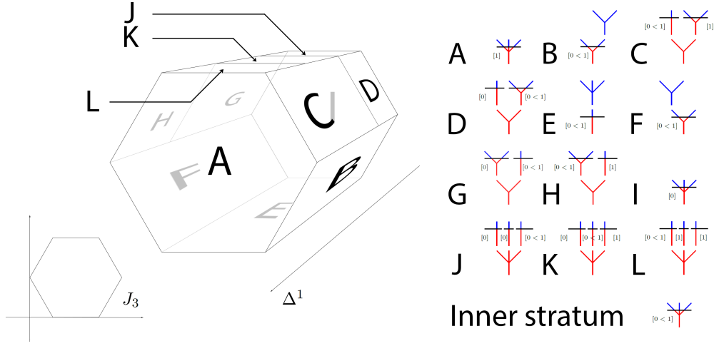
FIGURE 3 – Le 1-multiplièdre \Delta^1 \times J_3
