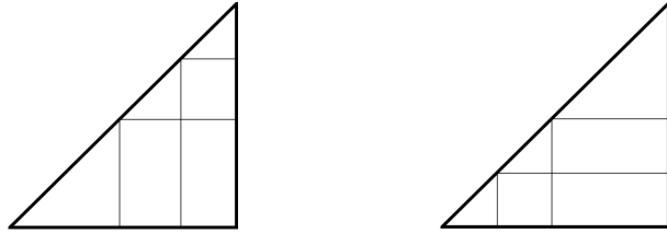
FIGURE 4. The (AW \times \text{id}) \circ AW -subdivision and the (\text{id} \times AW) \circ AW -subdivision of \Delta^2
