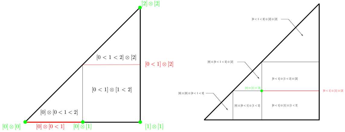
FIGURE 6. The AW and \text{AW}^{\circ 2} subdivisions of \Delta^2
