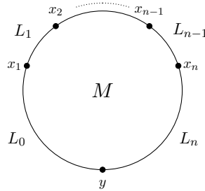
FIGURE 3 – A pseudo-holomorphic disk with Lagrangian boundary conditions on the L_i and n + 1 marked boundary points
