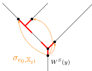
FIGURE 31. Representation of the map \sigma_{e_0, \mathbb{X}_{t^1}} .
