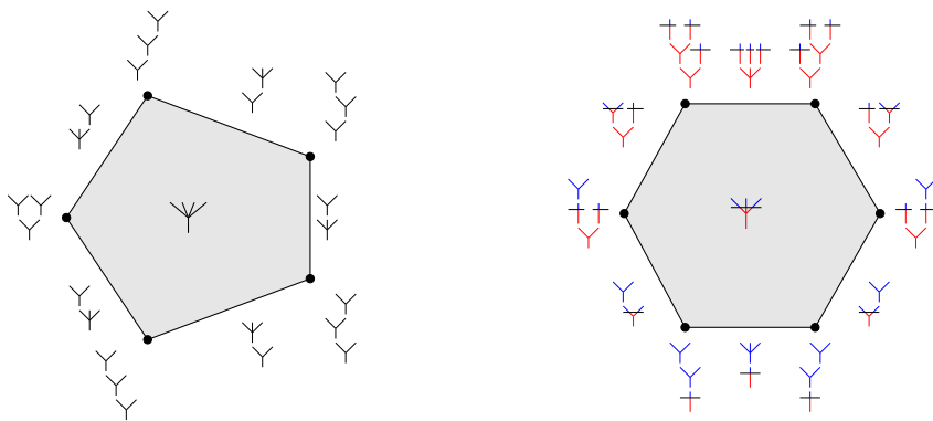
The associahedron K_4 and the multiplihedron J_3 \dots
