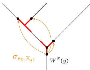
FIGURE 31. Representation of the map \sigma_{e_0, \mathbb{X}_{t^1}} .
