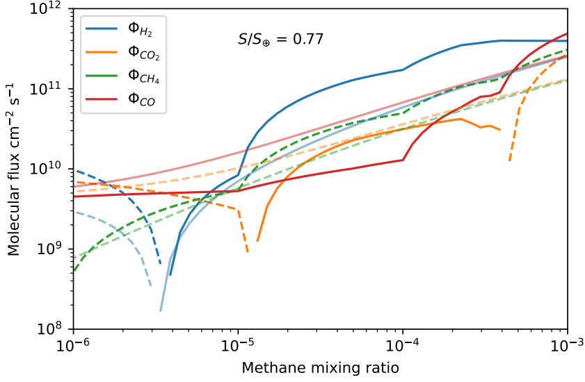
Figure 5.10. | Comparison between the photochemical fluxes in the atmosphere of the early Earth (3.8 billion years ago, S/S_{\oplus} = 0.77 ) as calculated by the Atmos model (solid colored lines) and as parameterized in Sauterey et al. (2020) 22 (soft-colored lines). Blue: dihydrogen flux \Phi_{H_2} . Orange: carbon dioxide flux \Phi_{CO_2} . Green: methane flux \Phi_{CH_4} . Red: carbon monoxide flux \Phi_{CO} . Solid lines: positive fluxes. Dashed lines: negative fluxes. Fluxes are given in molecules \text{cm}^{-2} \text{s}^{-1} , methane abundance is given in mixing ratio (or bar for the 1 bar atmosphere). For these computations, constant mixing ratios p_{CO_2} = 10^{-3} and p_{H_2} = 10^{-3} are set.
