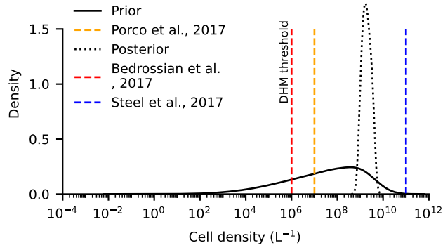
Figure 4.3. | Cell densities in the plume. The continuous and dotted black curves are respectively the prior and posterior probability estimates of dead cells concentration in water escaping the hydrothermal environment. It is important to note that this estimate ignores possible dilution occurring during the ocean plume’s ascension and bubble scrubbing at the ocean-ice interface. The orange dashed line corresponds to the estimate of plausible cell density in the plume from Porco et al. (2017) 119 . The blue dashed line represents the calculation in Steel et al. (2017) 120 ( \approx 10^{11} cells \text{kg}^{-1} ). The red dashed line highlights the lower density threshold for detecting cells using digital holographic microscopy (DHM) 167 .
