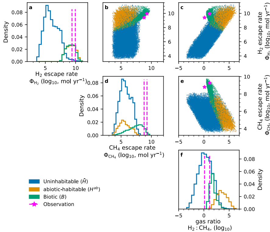
Figure 3.2. | Cassini observations and distributions of model outputs over the space of observables : inferred H_2 and CH_4 fluxes ( \Phi_{H_2} and \Phi_{CH_4} ), and gas ratio H_2 : CH_4 . a, d, f , Density distributions of observables pseudo-data generated by model simulations. In blue, subset of simulations in which no population of methanogens could grow ('uninhabitable' scenario, \bar{H} ). In orange, subset of simulations in which a population of methanogens is possible but their activity is not taken into account ('abiotic-habitable' scenario, H^{ab} ). In green, subset of simulations in which methanogens can grow, and their activity is taken into account to produce pseudo-data ('biotic' scenario, B ). Magenta dashed lines (vertical) indicate the actual Cassini observations 64 . Note the \log_{10} scale on the horizontal axis. b, c, e , Joint distributions of observable pseudo-data generated by the model. Magenta stars indicate the Cassini observations. Note the \log_{10} scale on both axes. This figure was generated from a set of 50,000 simulations using random values of internal parameters drawn from the distributions described in Extended Data Table C.1. In about 32% of these simulations, the drawn set of parameters allowed the modeled population of methanogens to grow ('habitable', H ), the remaining 68% were found to pertain to the 'uninhabitable' scenario ( \bar{H} , blue). The 'habitable' subset was evenly split at random into two subsets of 8,008 simulations. In one subset, we did not simulate methanogenesis ('abiotic-habitable' scenario, H^{ab} , orange), while we simulated methanogenesis coupled with the geochemical model in the second subset ('biotic' scenario, B , green). See Methods and Extended Data Tables C.2 and C.3 for model equations and parameter values.
