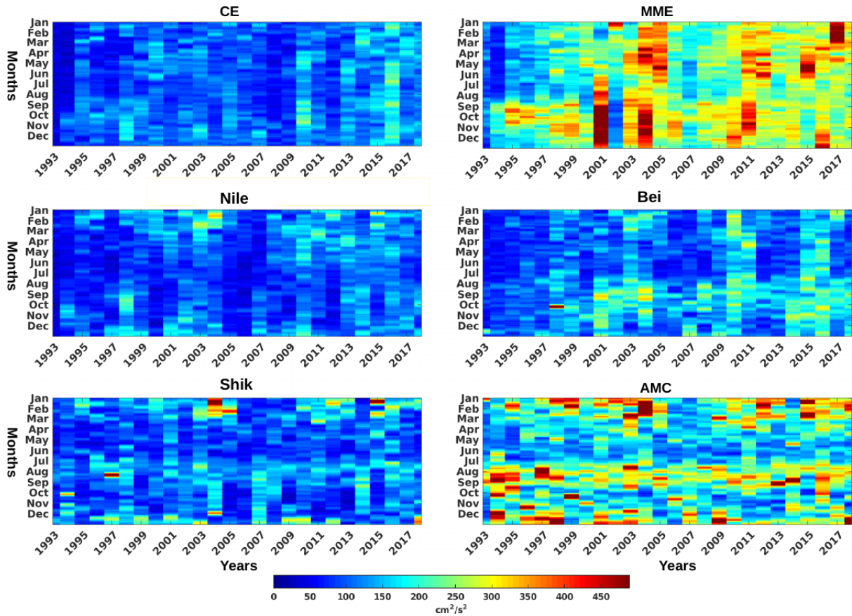
FIGURE 7.4: The variation of the daily average Kinetic energy ( \text{MKE } \text{cm}^2/\text{s}^2 ), in each box from 1993 to late 2018.
