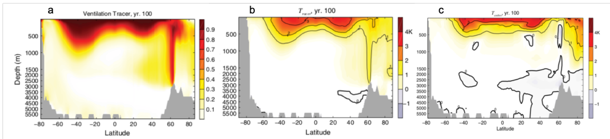
Figure 0.12: From Marshall et al. [2015]. Zonal mean (a) Idealized ventilation tracer whose value at the surface is set to unity (b) Passive temperature tracer anomaly (c) Temperature anomaly, after 100 years of a simulation forced with homogeneous radiative forcing and a constant climate feedback parameter.
