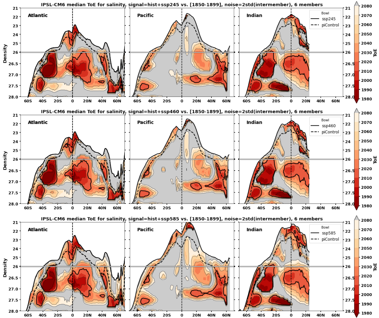
Figure I.2: Ensemble median Time of Emergence for the ssp245, ssp460 and ssp585 scenarios (6 members each).
